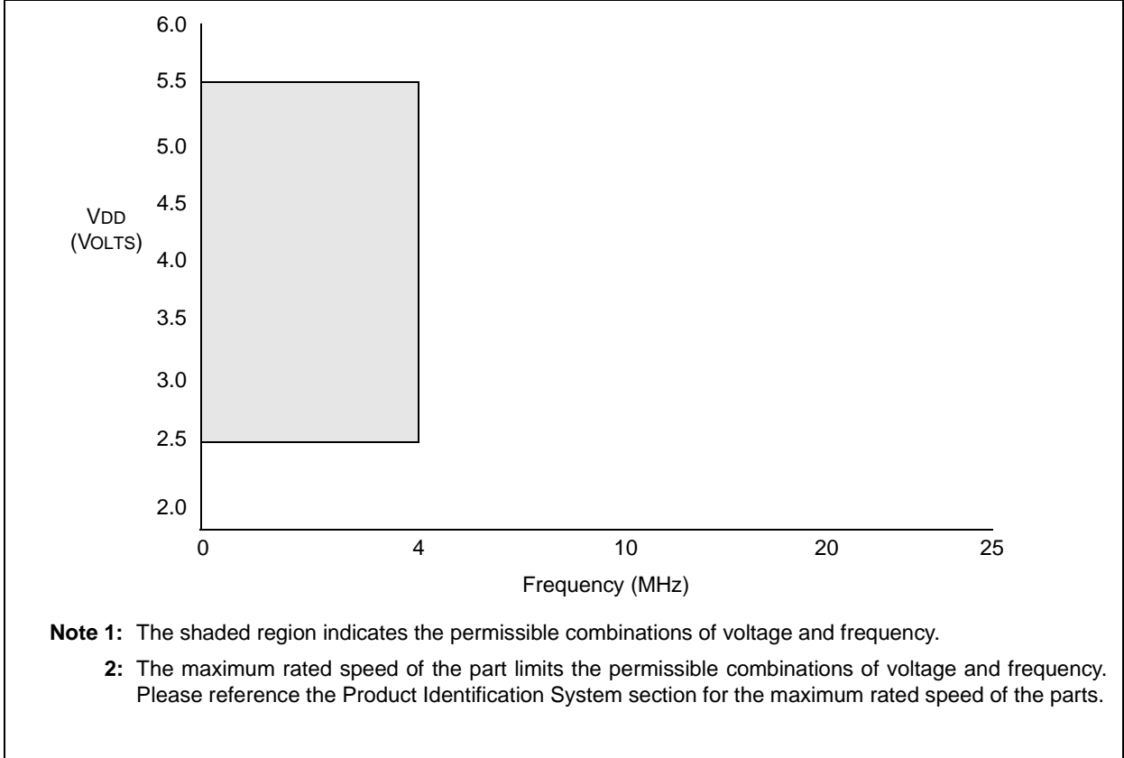
FIGURE 5: PIC16LCR620A VOLTAGE-FREQUENCY GRAPH, -40^{\circ}\text{C} \leq T_A \leq +125^{\circ}\text{C}
