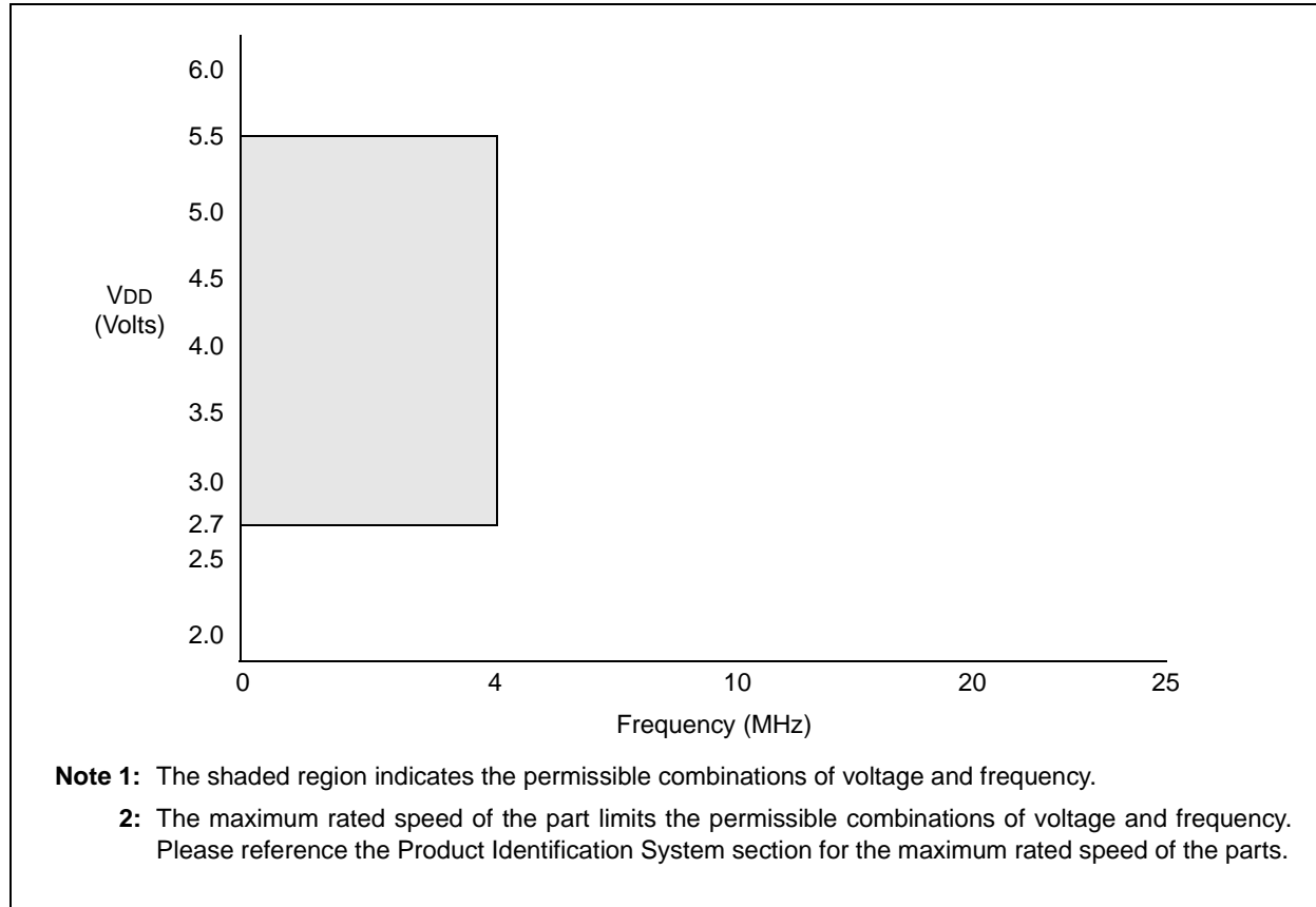
FIGURE 2: PIC16LC620A VOLTAGE-FREQUENCY GRAPH, -40^{\circ}\text{C} \leq T_A \leq 0^{\circ}\text{C}
