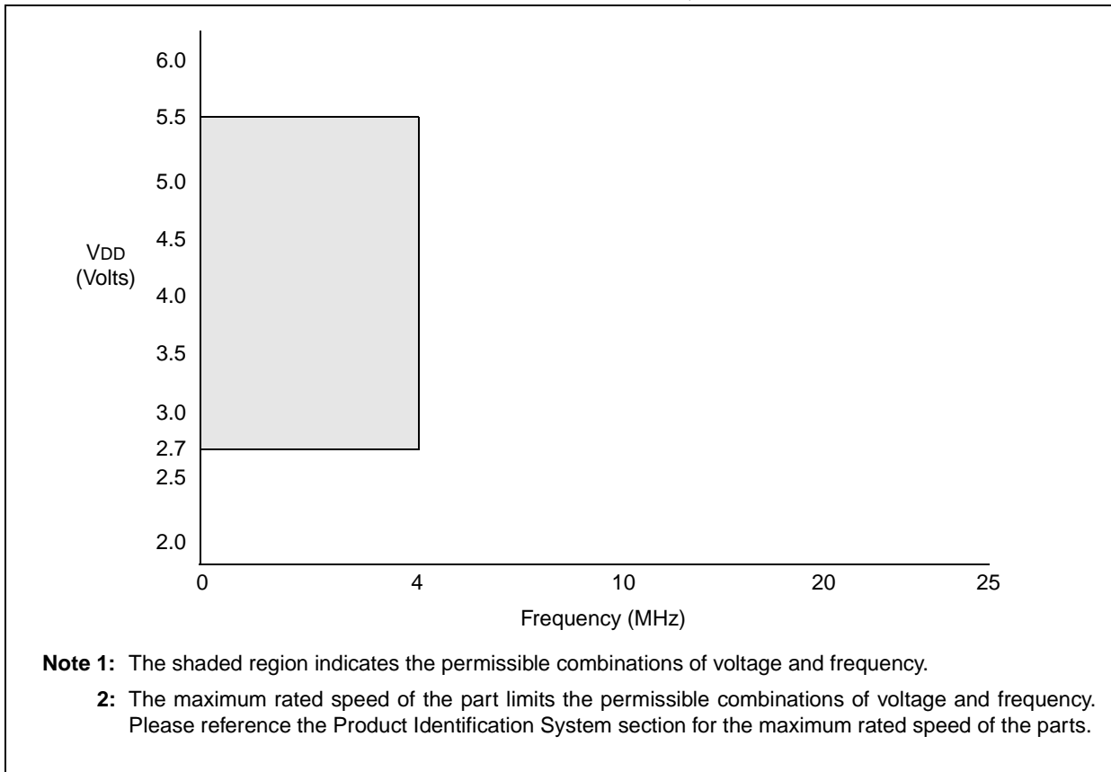
FIGURE 1: PIC16LC56A VOLTAGE-FREQUENCY GRAPH, -40^{\circ}\text{C} \leq T_A \leq 0^{\circ}\text{C}
