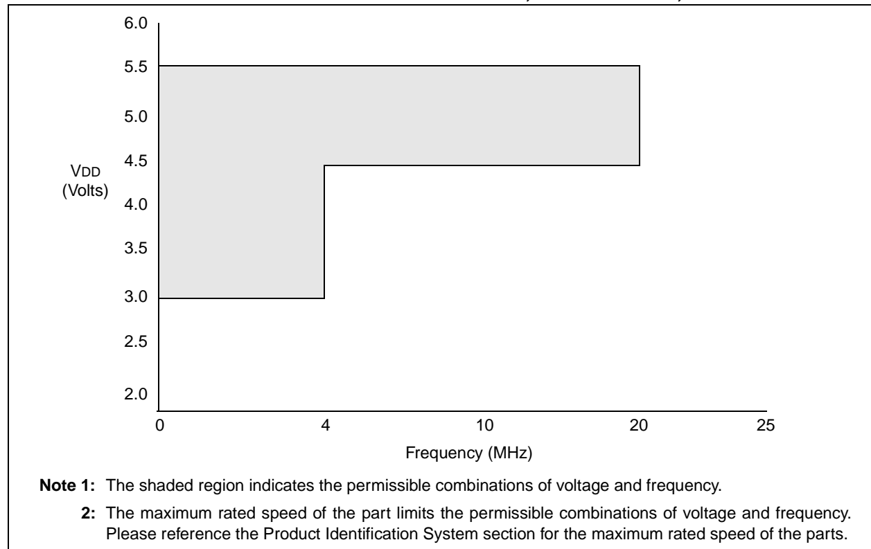
FIGURE 2: PIC16C56A VOLTAGE-FREQUENCY GRAPH, -40^{\circ}\text{C} \leq T_A < 0^{\circ}\text{C} , +70^{\circ}\text{C} < T_A \leq +125^{\circ}\text{C}
