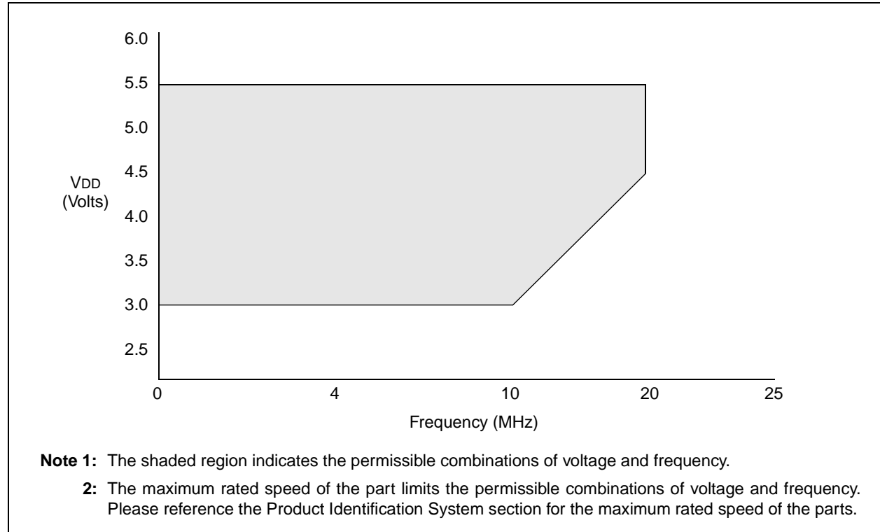
FIGURE 2: PIC16C56A VOLTAGE-FREQUENCY GRAPH, -40^{\circ}\text{C} \leq T_A < 0^{\circ}\text{C} , +70^{\circ}\text{C} < T_A \leq +125^{\circ}\text{C}
