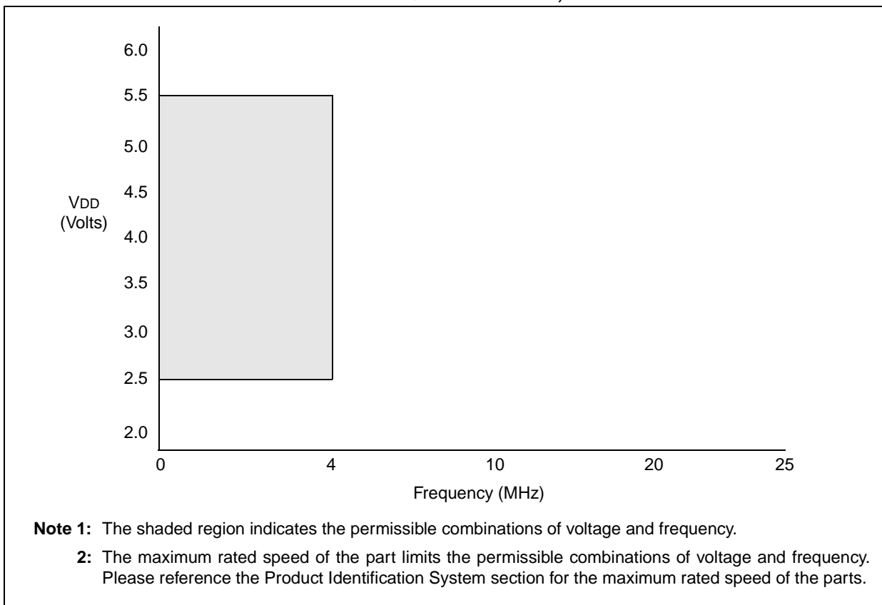
FIGURE 3: PIC16LCE62X VOLTAGE-FREQUENCY GRAPH, +70^{\circ}\text{C} \leq T_A \leq +125^{\circ}\text{C}
