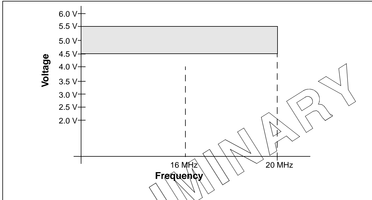
FIGURE 1: PIC16F84A-20 VOLTAGE-FREQUENCY GRAPH
