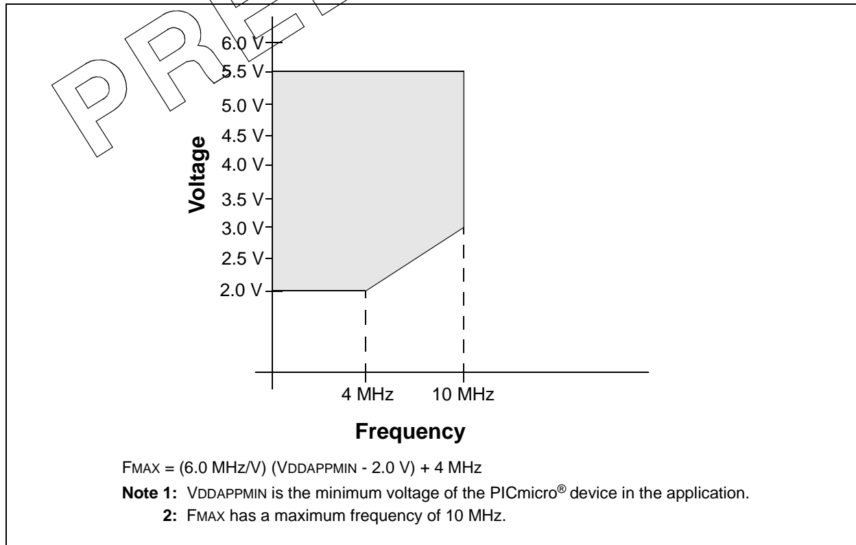
FIGURE 2: PIC16LF84A-04 VOLTAGE-FREQUENCY GRAPH
