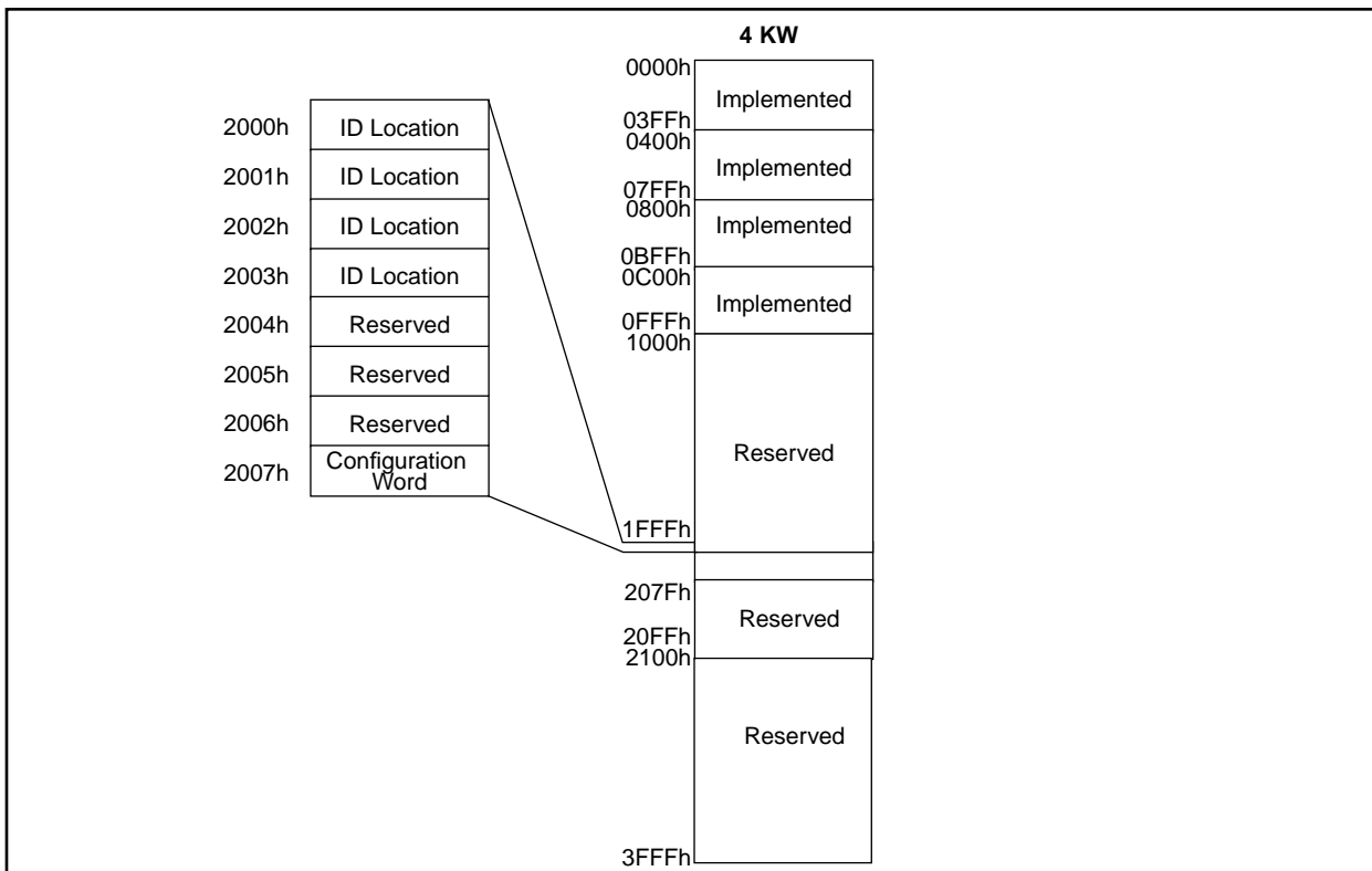
FIGURE 2-1: PROGRAM MEMORY MAPPING
