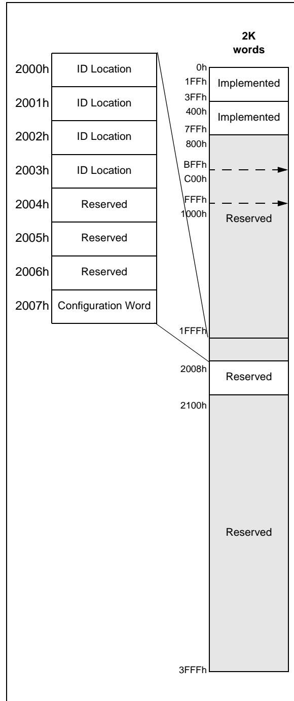
FIGURE 2-1: PROGRAM MEMORY MAPPING
