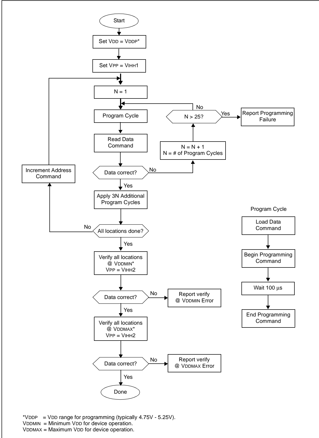
FIGURE 2-2: PROGRAM FLOW CHART - PIC16C432 PROGRAM MEMORY
