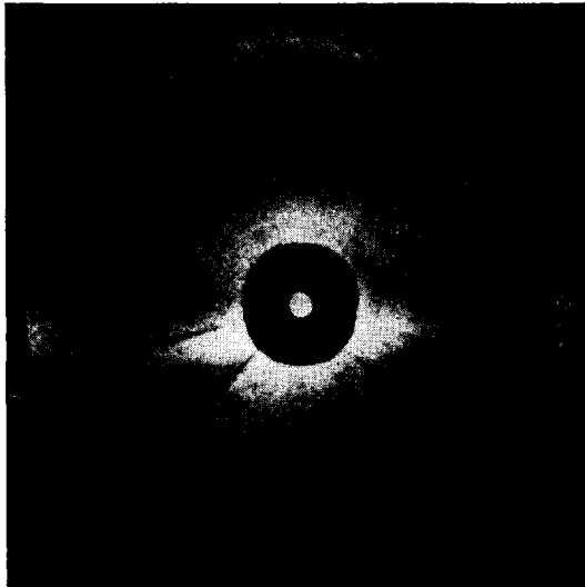
FIG. 6-2.—A shadow on the PPI caused by a large airplane that blocks the radar beam. This airplane is flying just below and slightly behind the one in which the photograph was taken. The radar signal from the airplane is lost in the bright spot at the center of this picture.
