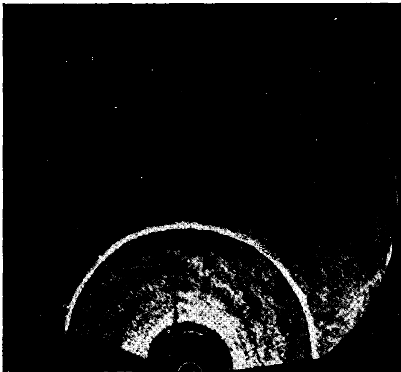
FIG. 3-12.—Highway displayed on an off-center PPI, 0.8^\circ beamwidth, \frac{1}{4} - \mu sec pulse.
