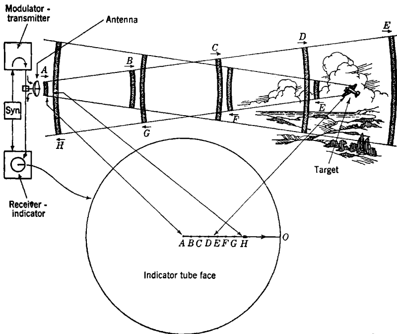
FIG. 1-3.—The life of a single pulse. The letters denoting the position of the pulse in space are also used to show the corresponding positions of the electron beam as it sweeps across the face of the indicator tube from A to O. The observer would see the signal at H only.
