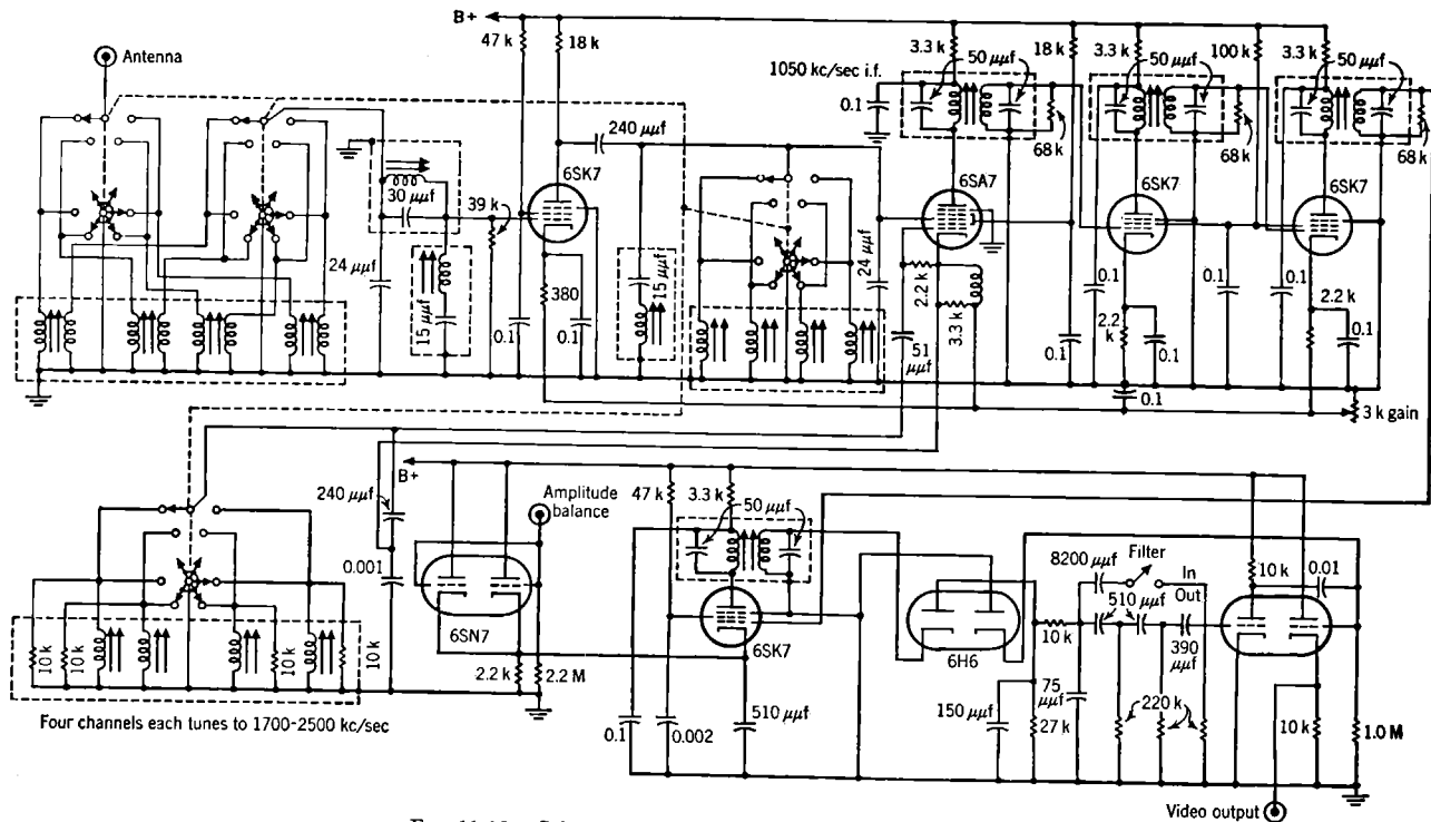
Fig. 11-12.—Schematic diagram of Model AN/APN-4 receiver.
