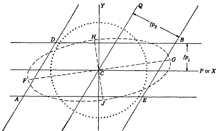
FIG. 3-18.—The error parallelogram, ellipse, and circle.
