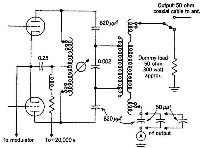
FIG. 9-8.—Simple diagram of output circuits.
