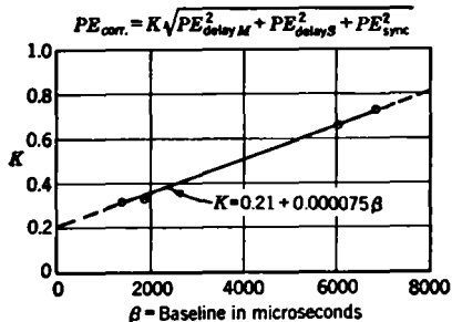
FIG. 5-20.—A form of the correlation coefficient defining the relative behavior of two points in the ionosphere, plotted against the separation between two transmitting stations, M (master) and S (slave).
