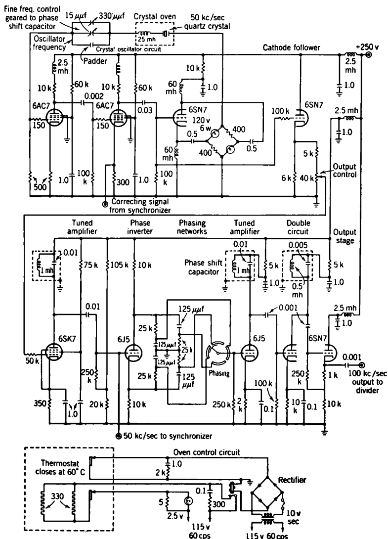
FIG. 7-7.—Schematic diagram of Model C-1 oscillator.
