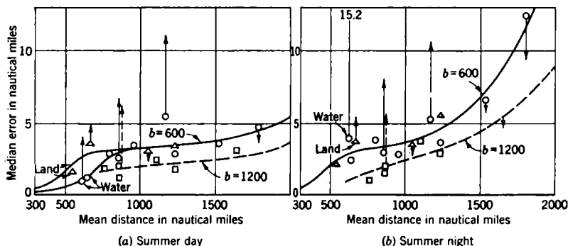
FIG. 5-47.—The median errors of the Low Frequency Loran experimental observations plotted as a function of distance. The curves are corrected to simulate operation at an angle of 45^\circ from a 600-mile baseline. The heads of the arrows appended to many of the experimental points indicate the values before correction.
