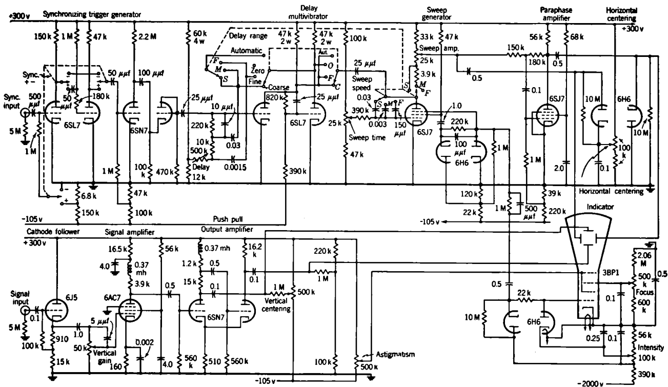
FIG. 7-6.—Schematic diagram of Model C-1 test oscilloscope.
