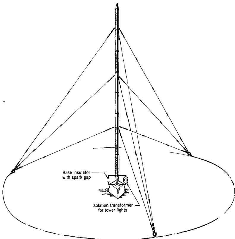
FIG. 10-20.—Elevation of Wincharger 110-ft transmitting antenna.
