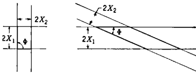
FIG. 3-16.—The parallelogram is larger when the crossing angle is smaller.
