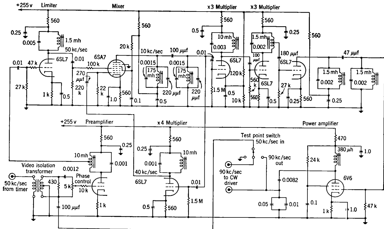
FIG. 9-13.—Circuit diagram of 90-kc/sec generator.
