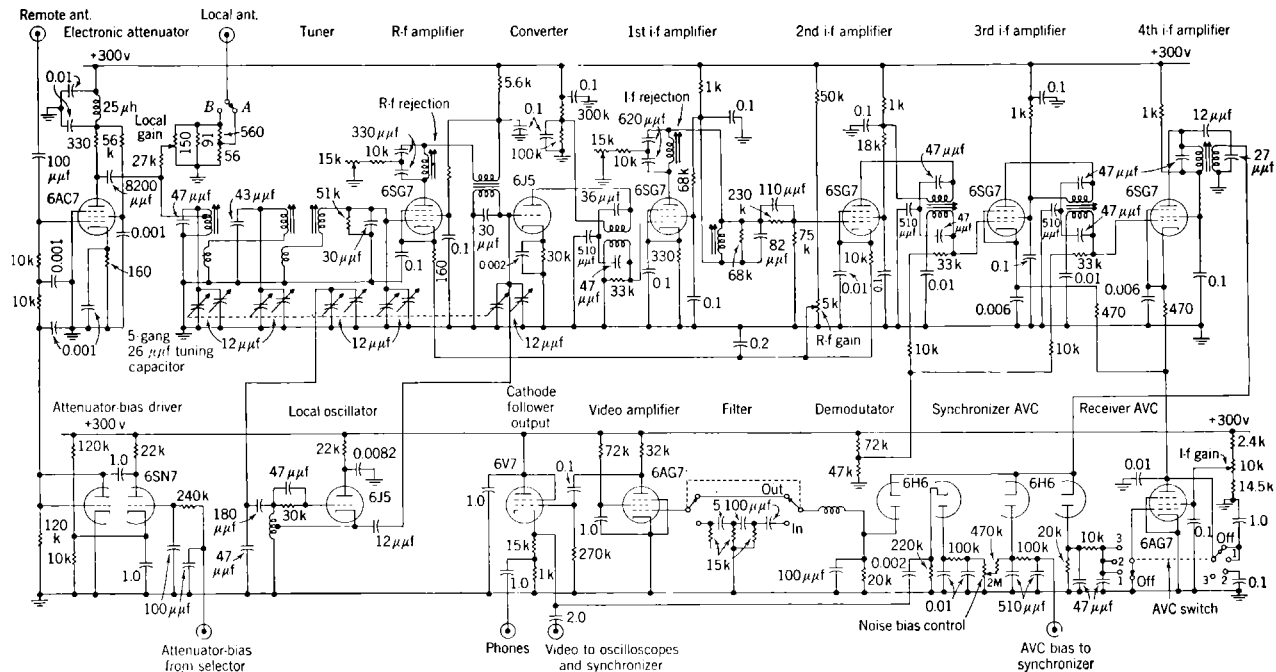
FIG. 7-16.—Schematic diagram of Model UE-1 receiver.
