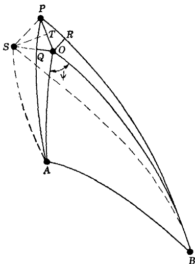
FIG. C-1.—The factor of geometrical precision.
