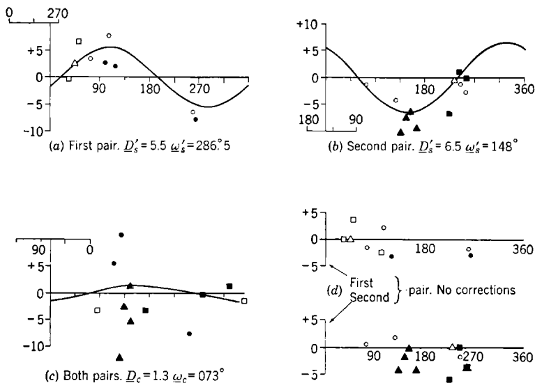
FIG. D-10.—Plots, Example III.
