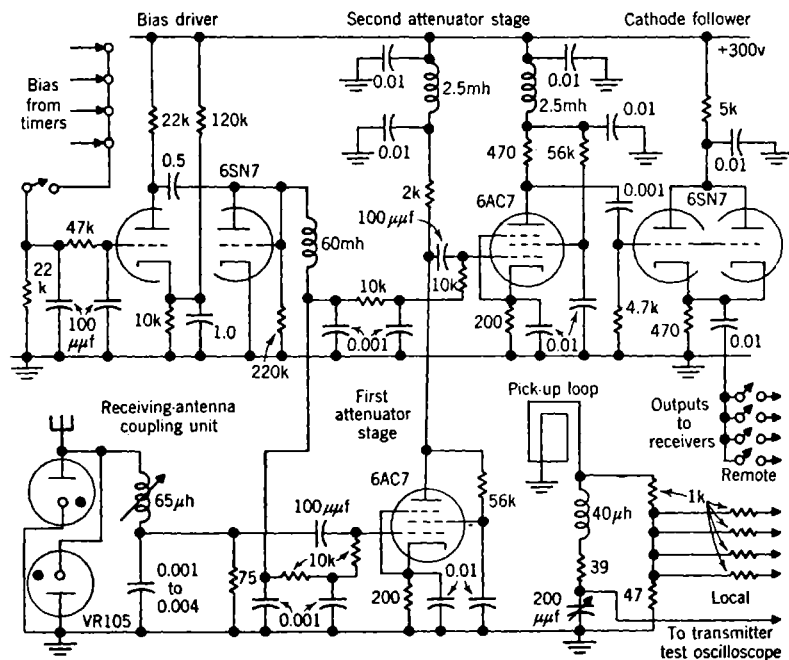
FIG. 8-3.—Schematic diagram of Model C-1 switching equipment.
