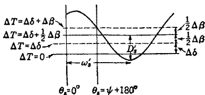
FIG. D-11.—Graphical solution if \Delta\beta and \Delta\delta are unknown.
