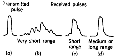
FIG. 5-14.—A representation of the complex pulse observed at short distances from a Loran transmitter. Loran sky-wave operation is uncertain and inaccurate except at medium and long ranges.
