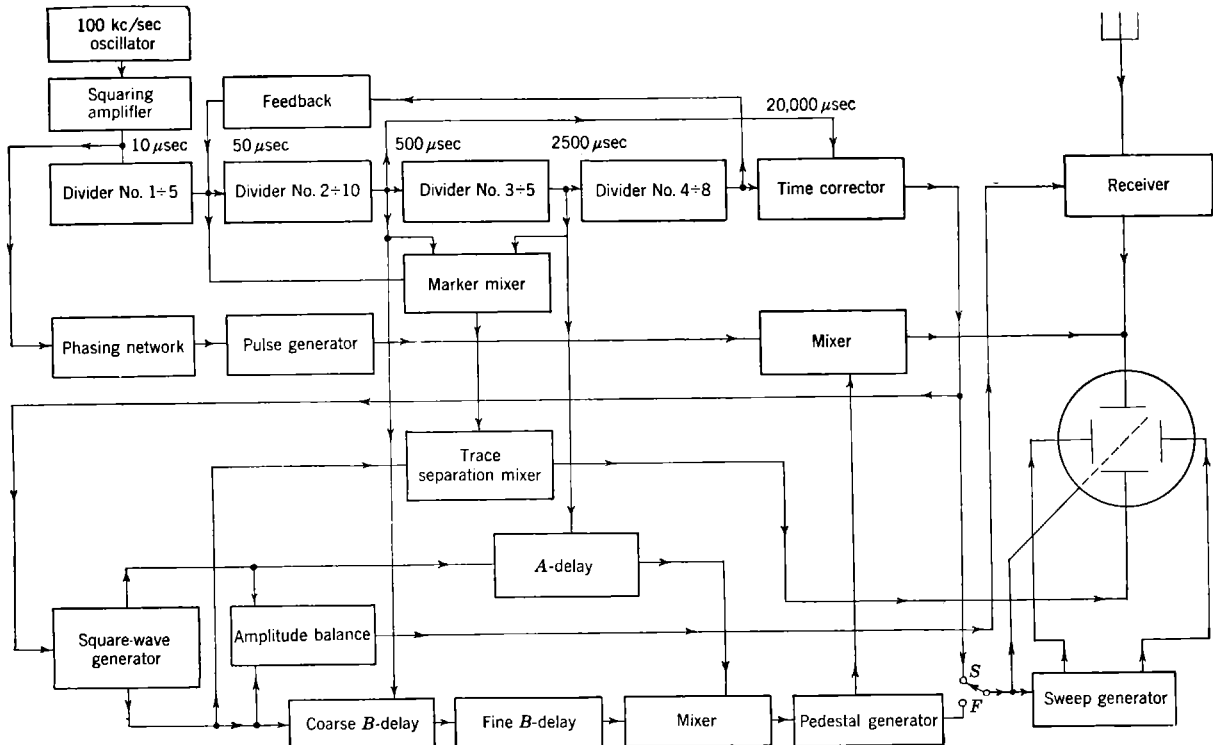
FIG. 11-5.—Block diagram of Model DAS-2 receiver-indicator.
