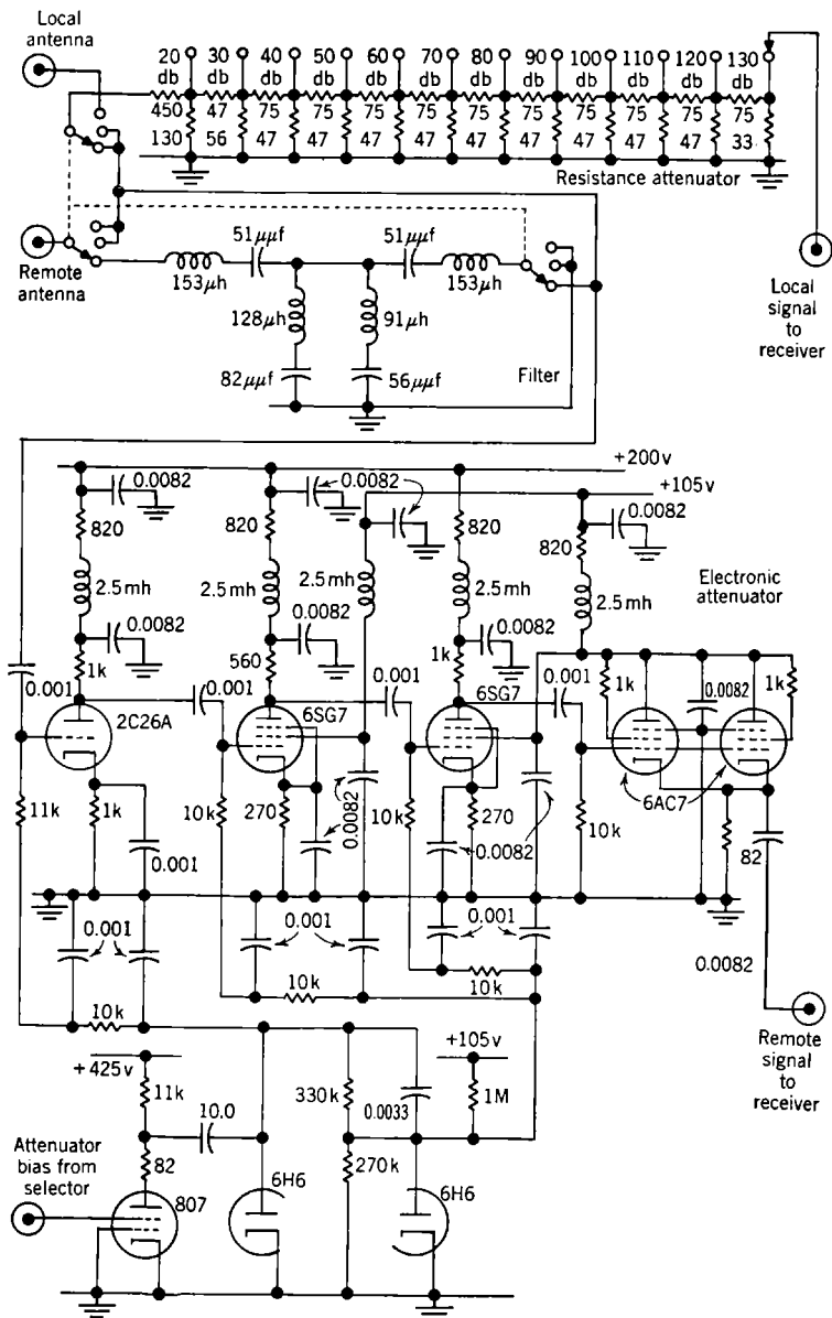
Fig. 8-7.—Schematic diagram of Model UM discriminator.
