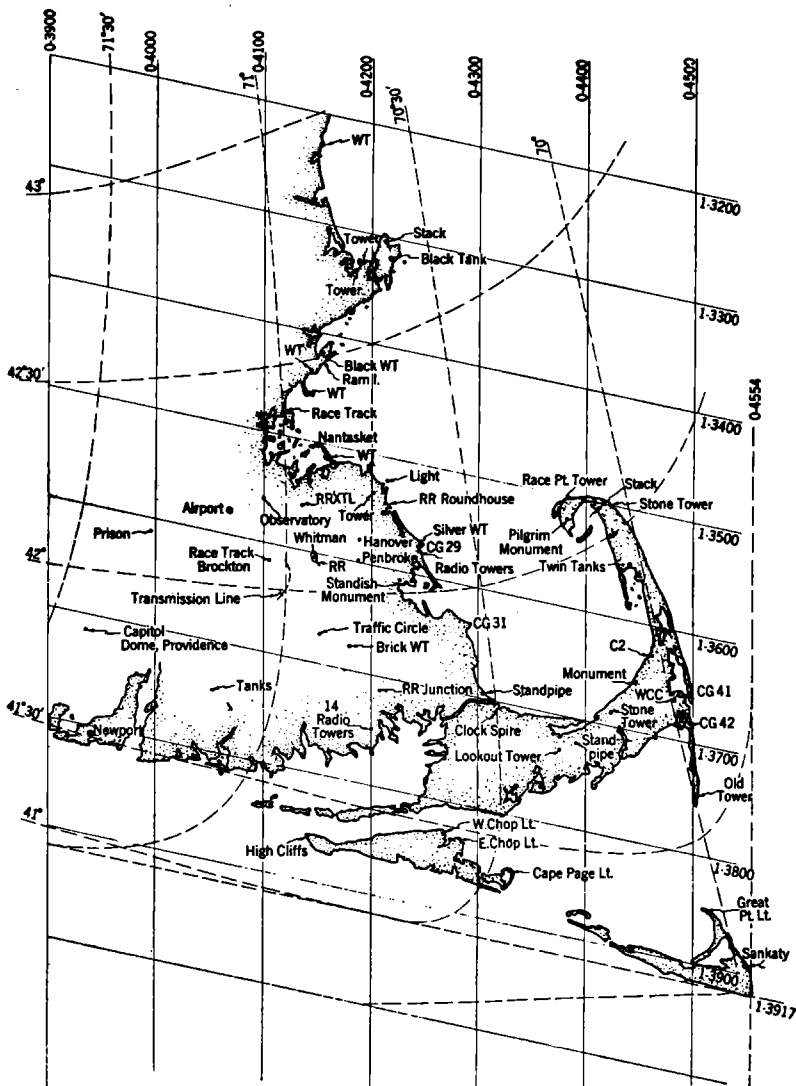
FIG. 4-1.—Rectilinear Loran projection of eastern Massachusetts.
