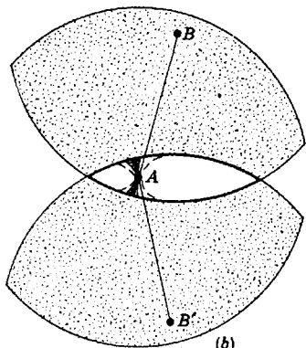
FIG. 3-11.—Standard form of a Loran triplet.
