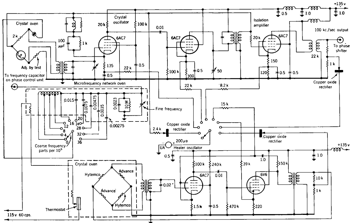
Fig. 7-13.—Schematic diagram of Model UE-1 oscillator.
