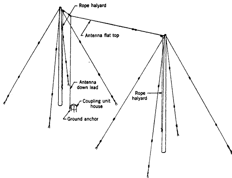
FIG. 10-18.—Standard "L" transmitting antenna.
