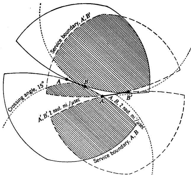
FIG. 3-22.—Common ground-wave service area for two pairs.
