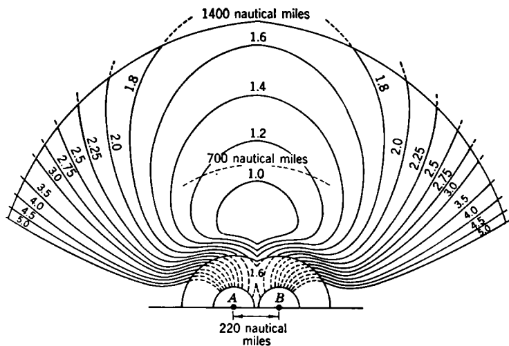
FIG. 5-22.—A contour diagram showing, as a function of the geographic position with respect to the transmitting stations, the probable error of a Standard Loran line of position when using sky waves.
