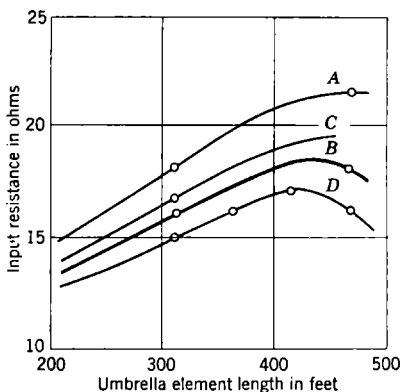
FIG. 10-32.—Input resistance at 180 kc/sec of 625-ft top-loaded antenna vs. length of loading elements. (A) Twelve elements anchored at 1250 ft; (B) twelve elements anchored at 835 ft; (C) eight elements anchored at 1250 ft; (D) eight elements anchored at 835 ft. (All data from measurement on 50-ft scale model.)
