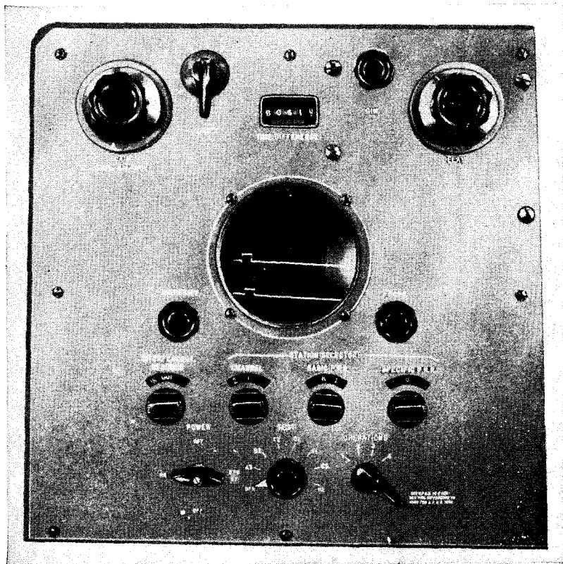
FIG. 11-7.—Front panel of Model DBE receiver-indicator showing slow-trace presentation without signals. (Courtesy of Sperry Gyroscope Co., Inc.)
