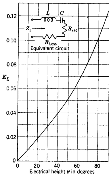
FIG. 10-16.—Factor for calculating equivalent series inductance of short antenna.
