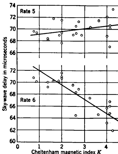
FIG. 5-25.—Variations in the sky-wave delay with magnetic activity over paths of approximately 1000 miles. The upper curve represents the behavior on a path whose midpoint was 39^\circ from the magnetic pole; the midpoint of the other path was within 26^\circ of the magnetic pole.
