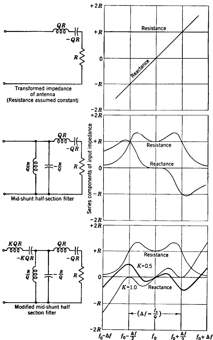
FIG. 10-8.—Simple coupling units with symmetrical impedance characteristics.
