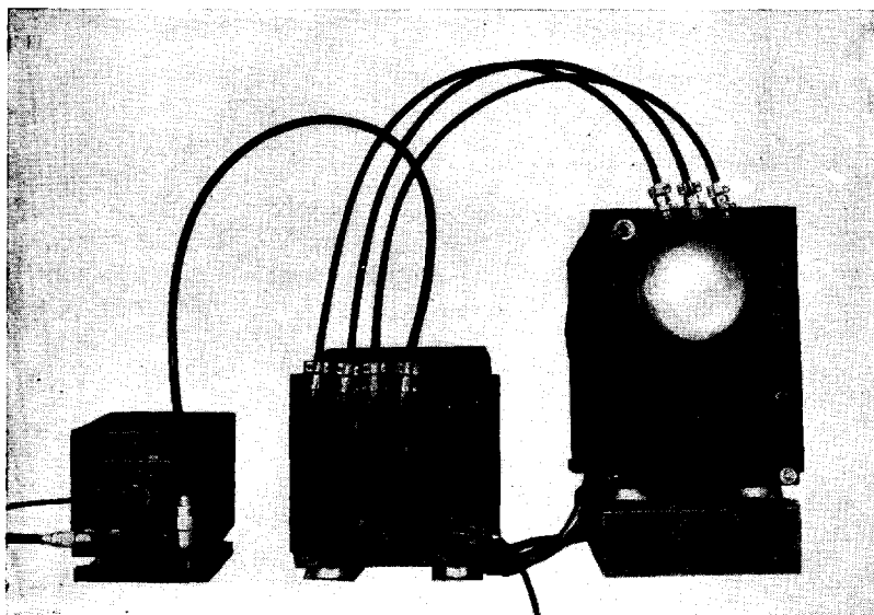
FIG. 11-9.—Converter attached to a standard receiver-indicator (AN/APN-4) to permit either Standard or Low Frequency signals to be observed.
