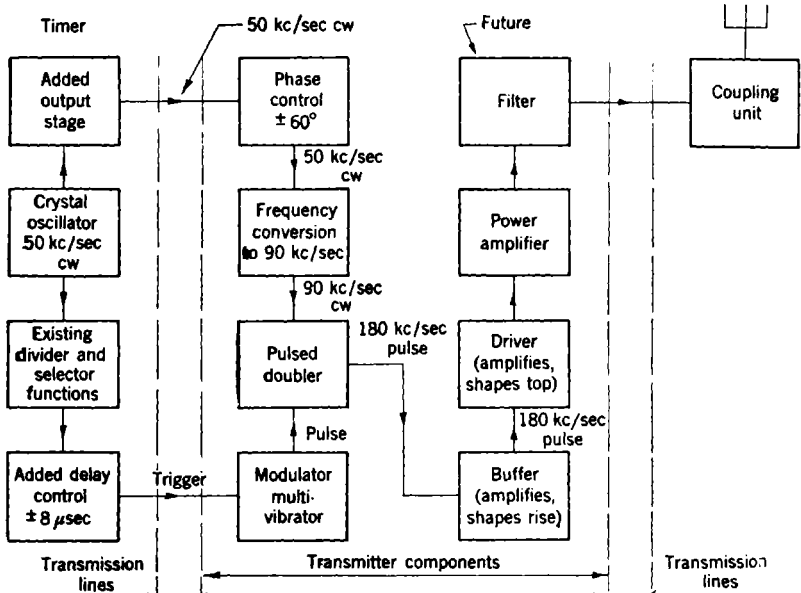
FIG. 9-11.—Block diagram of Low Frequency transmitter.
