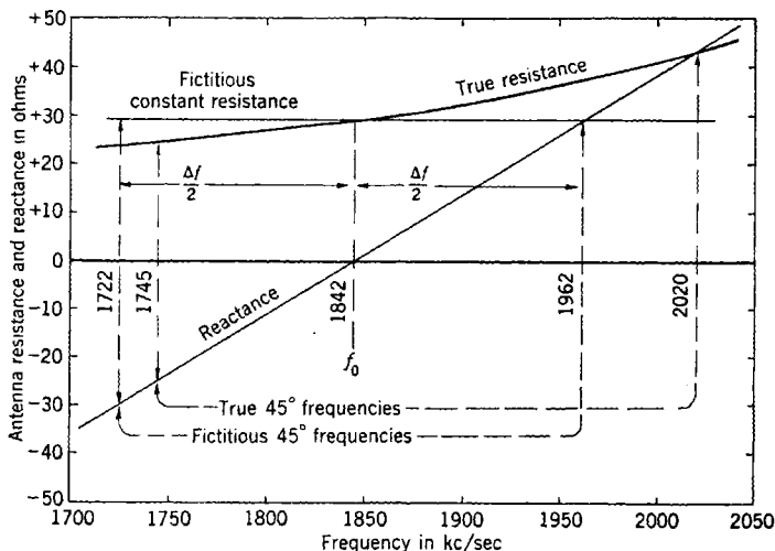
FIG. 10-2.—Illustrative bandwidth calculation for Wincharger antenna.
