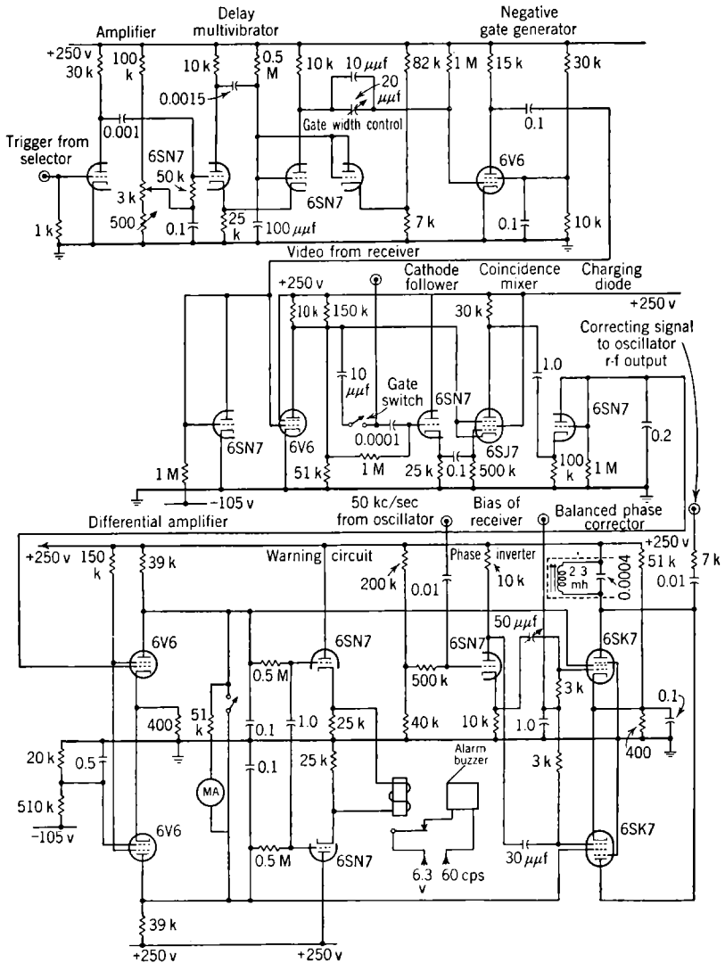
FIG. 7 10.—Schematic diagram of Model C-1 synchronizer.
