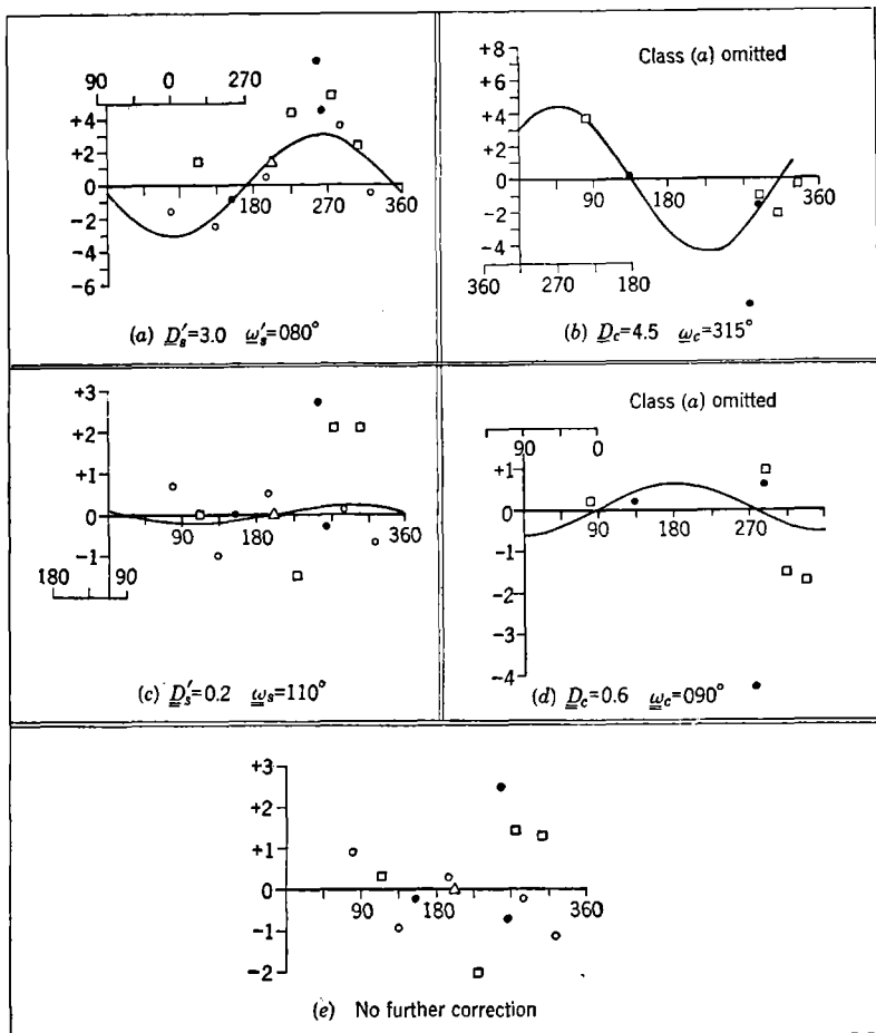
FIG. D-9.—Plots, Example II.
