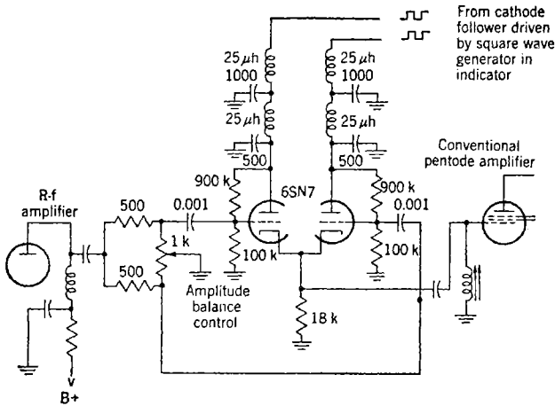
Fig. 12-2.—Dual cathode-follower gain-balance circuit.
