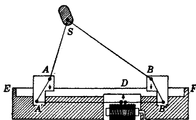
FIG. 6-2.—Diagram of the Hygraph.
