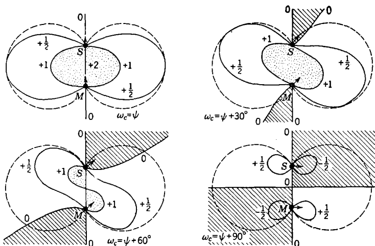
FIG. D-3.—Common displacement of stations, first quadrant. Reversing directions and signs gives patterns for third quadrant. Interchanging right and left of each pattern (mirror image) gives fourth quadrant patterns. Both changes together give second quadrant. Angles clockwise from vertical.
