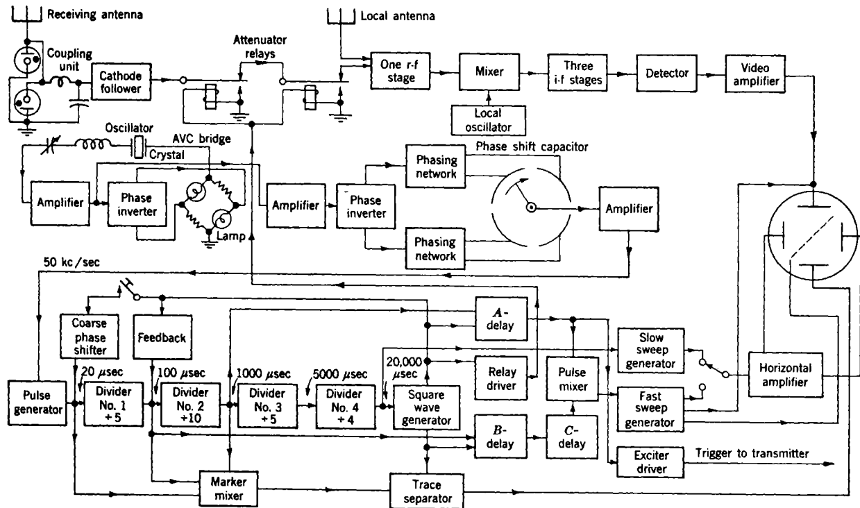
FIG. 7.2.—Block diagram of Model B-1 timer.
