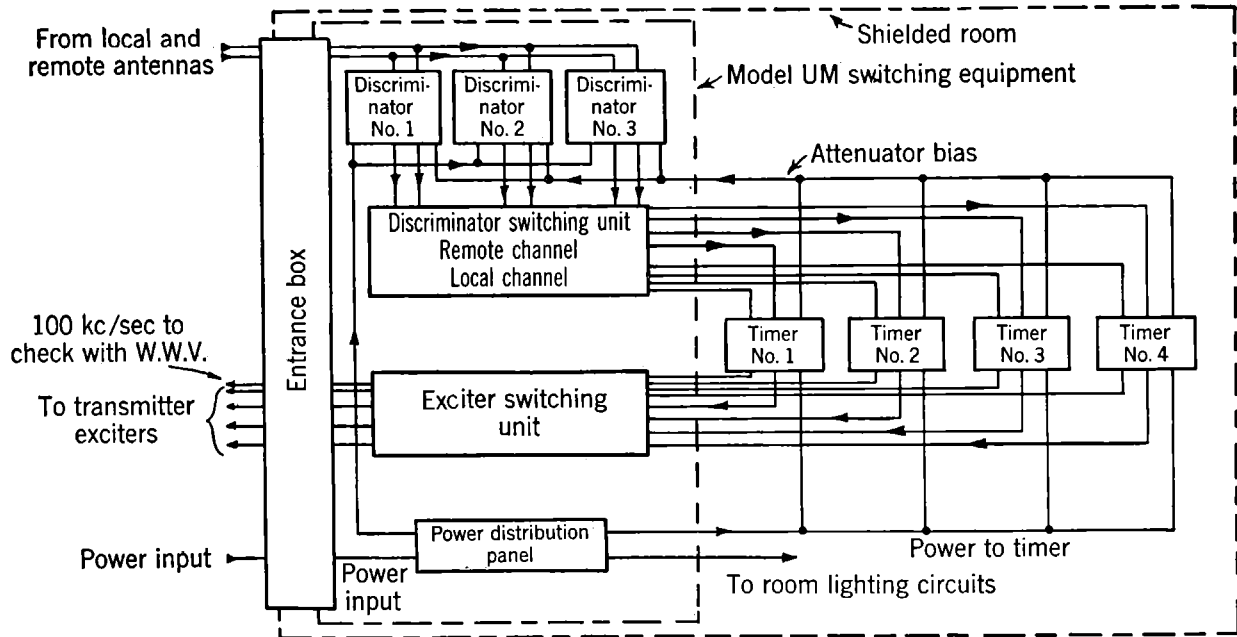
FIG. 8-5.—Block diagram of transmitting, timing, and Model UM switching equipment in a typical double-pulsed ground station.
