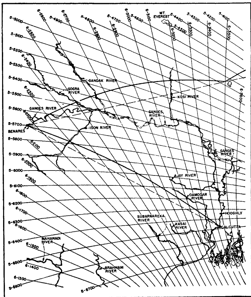
FIG. 4-2.—Lorhumb line in north India.
