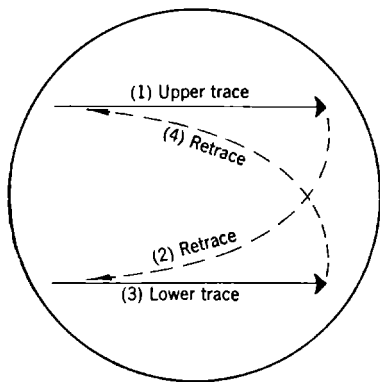
FIG. 3-6.—Indicator oscilloscope traces.
