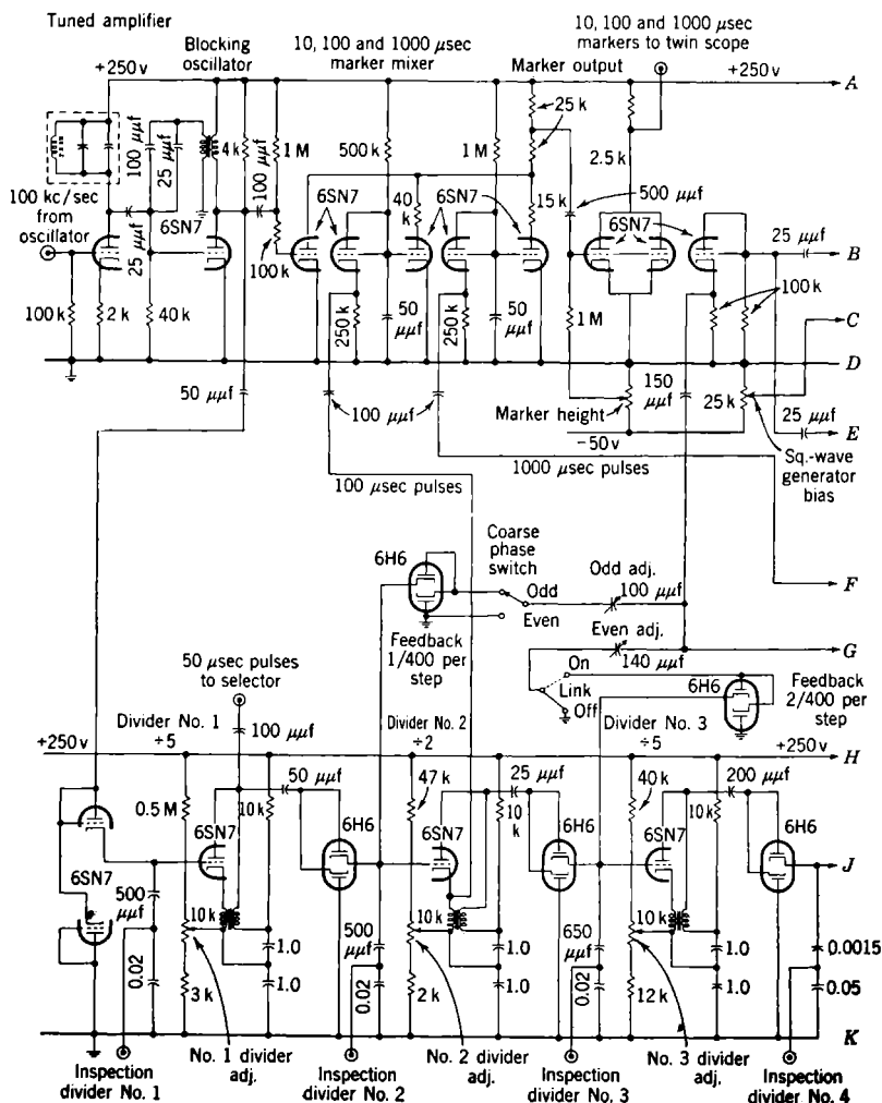
FIG. 7-8.—Schematic dia-
