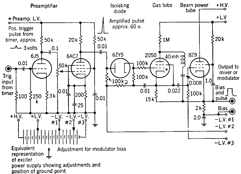
FIG. 9-4.—Simple diagram of exciter.
