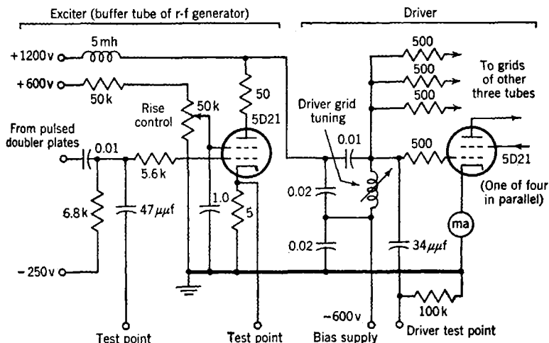
FIG. 9-16.—Simplified circuit of buffer.
