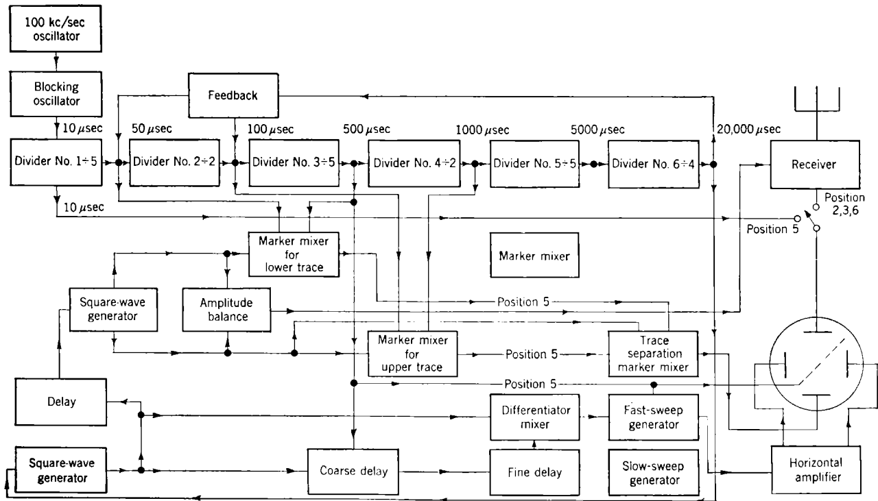
FIG. 11-17.—Block diagram of Model AN/APN-9 receiver-indicator on Positions 2, 3, 5, and 6 of function switch.
