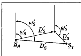
FIG. D-4.—First and second approximation.
