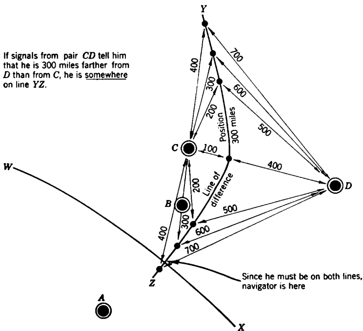
FIG. 3-2.—Determination of position by Loran.
