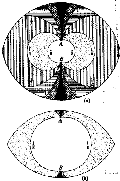
FIG. 3-10.—Service area of a pair.
