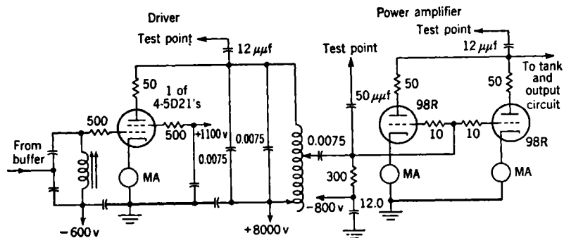
FIG. 9-17.—Simplified circuit of driver.
