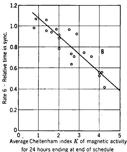
FIG. 5-24.—The reduction in the serviceability of a Sky-wave Synchronized Loran pair with increasing magnetic activity. This effect is important only when the midpoint of the pair is within about 30^\circ of the earth's magnetic pole.
