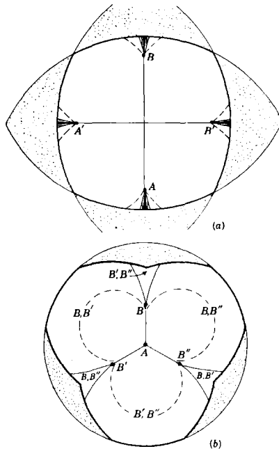
FIG. 3-15.—Quadrilateral and star chain.
