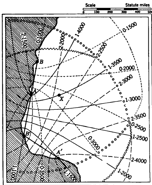
FIG. 3-12.—A Standard Loran chain of three pairs.
