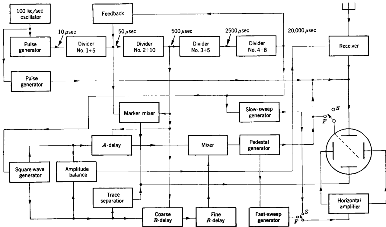
FIG. 11-3.—Block diagram of Model DAS-1 receiver indicator.
