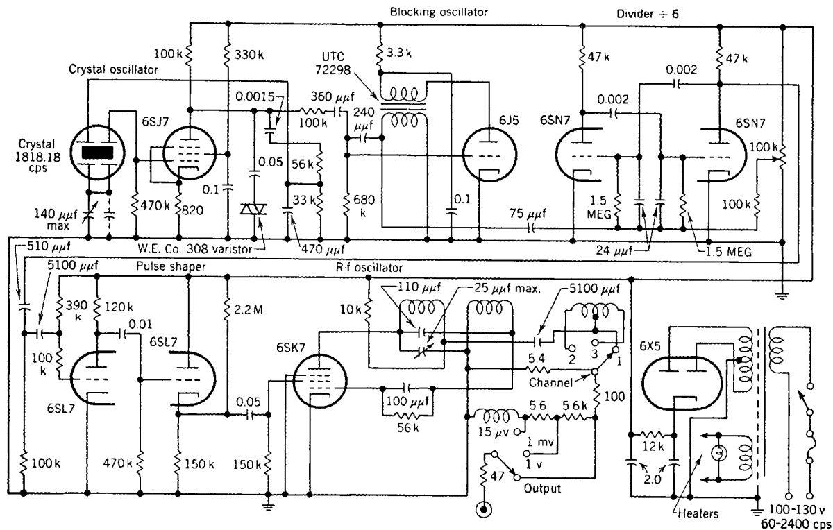
FIG. 11-19.—Schematic diagram of pulse-signal generator.
