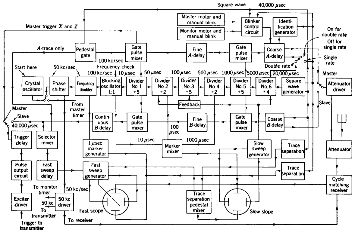
FIG. 7-19.—Block diagram of Model C-1 timer modified for Low Frequency Loran.
