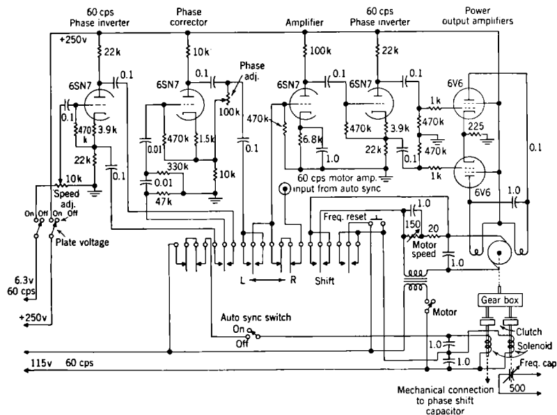
FIG. 7-15.—Schematic diagram of Model UE-1 phase-control unit.
