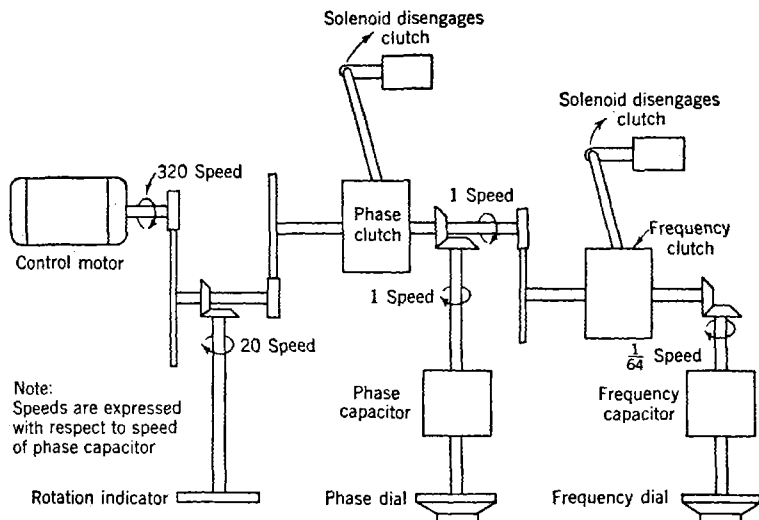
Fig. 7-14.—Functional diagram of phase- and frequency-control system of Model UE-1 timer.
