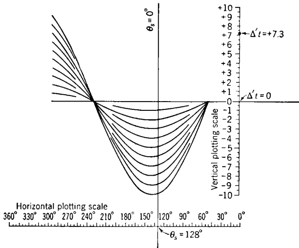
FIG. D-7.—Plotting the point, \theta_s = 128^\circ , \Delta'T = +7.3 .
