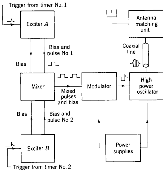
FIG. 9-3.—Block diagram of Model TDP transmitter.
