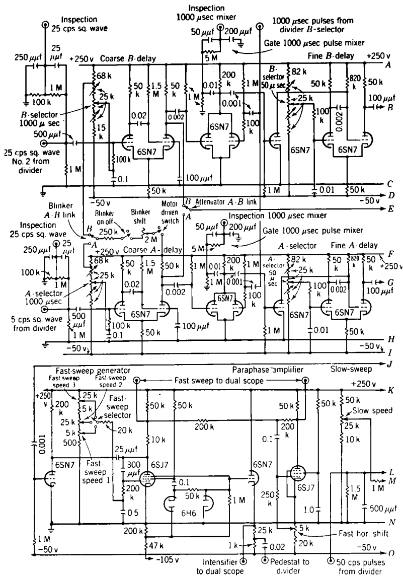
FIG. 7-9.—Schematic diagram
