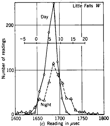
FIG. 5-45.—Distribution curves, similar to those of Fig. 5-39, of Low Frequency Loran readings at Little Falls.
