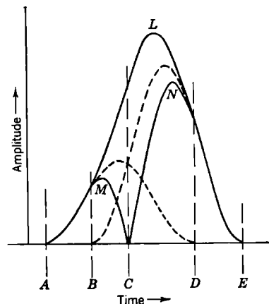
FIG. 5-31.—A simplified diagram indicating how Low Frequency Loran pulse shapes can vary with the phase relation between ground- and sky-wave components.
