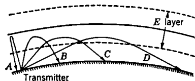
FIG. 5-9.—A diagram illustrating the variation of penetration into an ionized layer as a function of the distance traversed by a ray.
