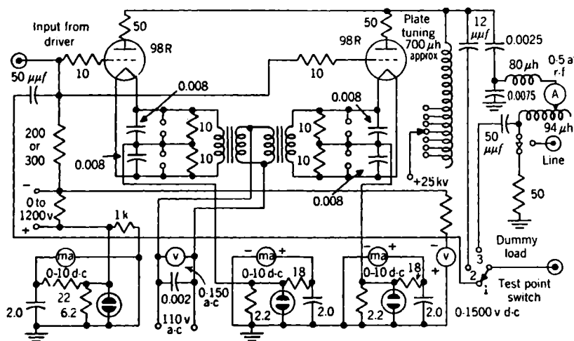
FIG. 9-18.—Simplified circuit of power amplifier.
