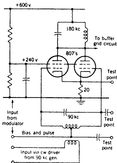
FIG. 9-14.—Simplified diagram of push-push doubler.
