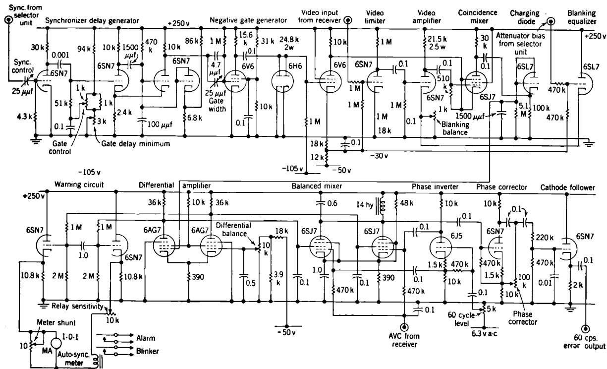
FIG. 7-17.—Schematic diagram of Model UE-1 synchronizer.
