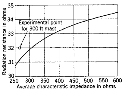
FIG. 10-11.—Radiation resistance at first resonance, as a function of characteristic impedance. (Data from Schelkunoff, Proc. IRE , September, 1941.)
