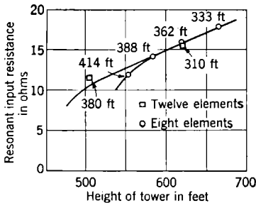
Fig. 10-30.—Effect of tower height on resonant input resistance. Numbers are lengths of elements at 180 kc/sec. Elements are anchored at distances of (1.33 \times \text{tower height}) .
