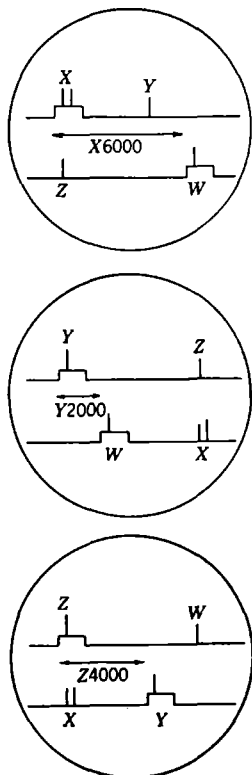
FIG. 3-25.—Low Frequency Loran readings.
