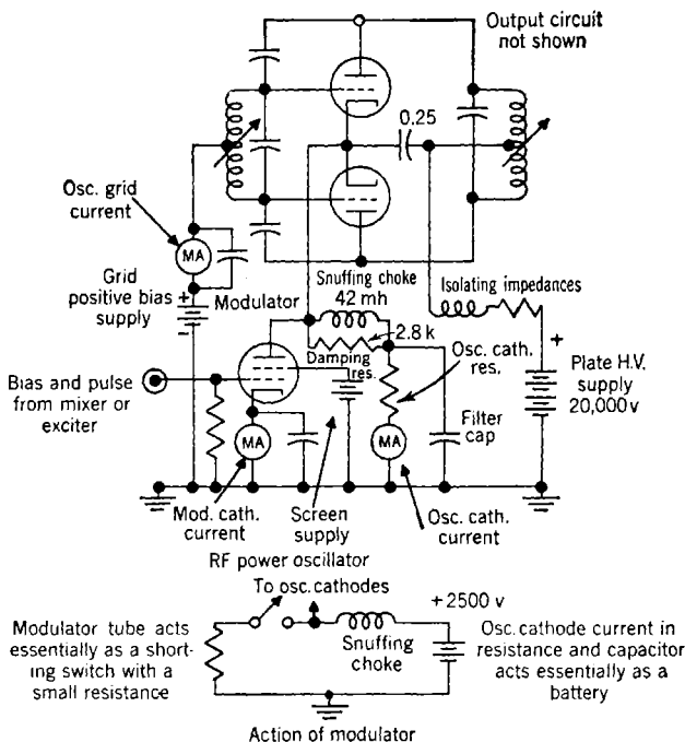
FIG. 9-6.—Simple diagram of modulator and oscillator.
