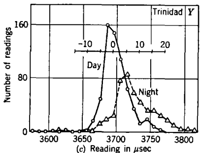
FIG. 5-43.—Distribution curves, similar to those of Fig. 5-39, of Low Frequency Loran readings at Trinidad.
