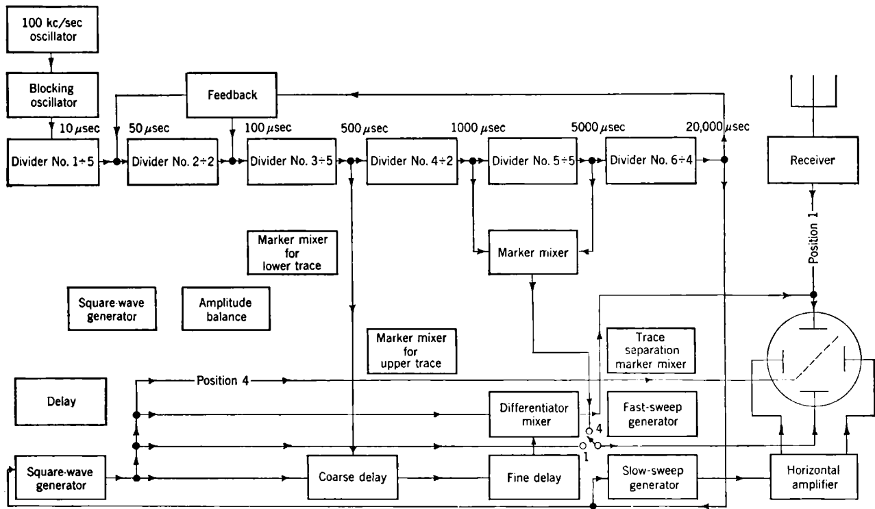
FIG. 11-16.—Block diagram of Model AN/APN-9 receiver-indicator on Positions 1 and 4 of the function switch.
