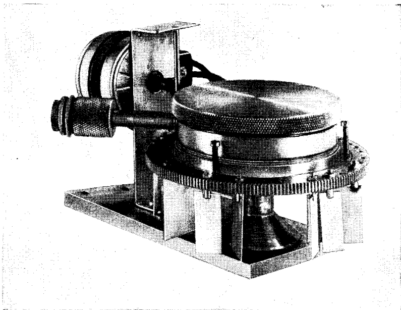
FIG. 11-20.—Supersonic pulse transmitter to simulate Loran ground station.
