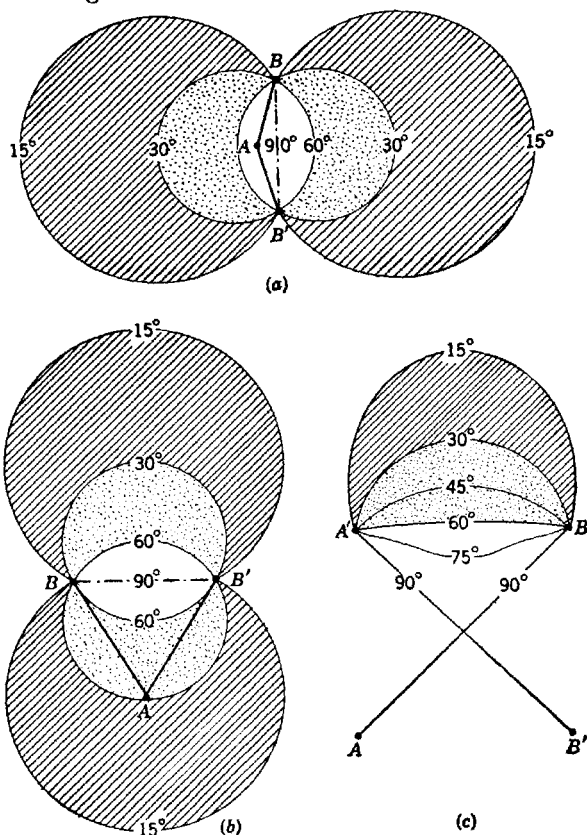
FIG. 3-17.—Curves of constant crossing angle.
