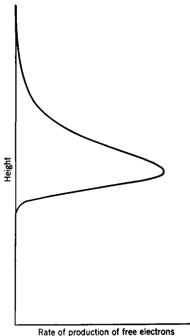
FIG. 5-5.—The vertical distribution of ionization that would be produced by a single ionizing agent acting upon a homogeneous atmosphere. The actual ionosphere may be simulated by a number of curves of this form superimposed in various ways.
