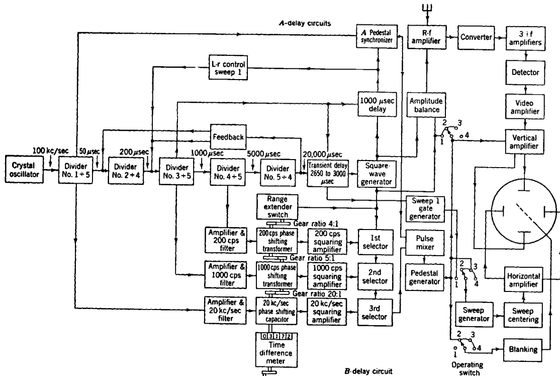
Fig. 11-8.—Block diagram of Model DBE receiver indicator.
