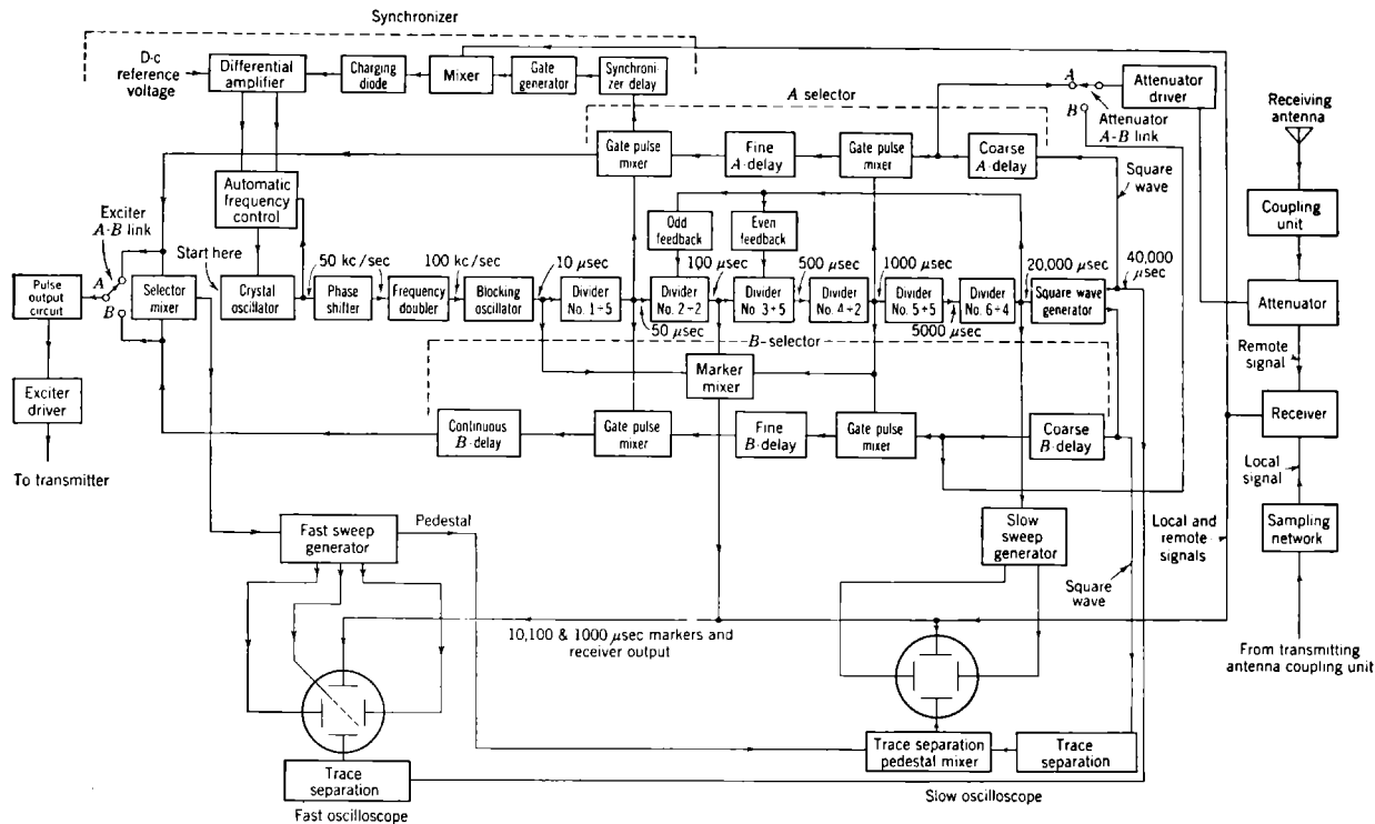
FIG. 7-4.—Block diagram of Model C-1 timer.
