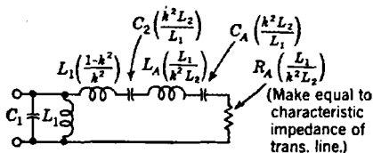
FIG. 10-7.—Use of transformer in matching antenna to transmission line.
