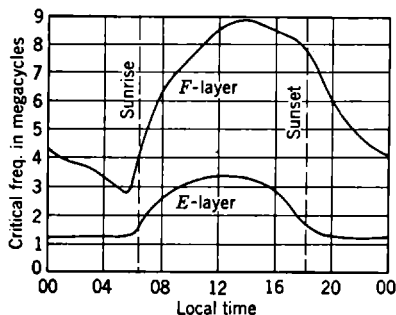
FIG. 5-8.—A typical diurnal variation of the critical frequencies of the E- and F-layers of the ionosphere. This quantity is proportional to the square root of the maximum density of ionization in a layer.
