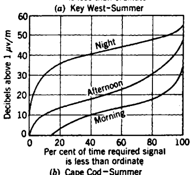
FIG. 5-2.—Diagrams showing the percentage of time that Low Frequency Loran signals must exceed certain values in order to be useful. Curves are shown for tropical summer and mid-latitude summer conditions. Each diagram shows curves for morning, afternoon, and night. For winter, or more northerly latitudes, noise conditions are less severe, and the required signals are correspondingly smaller.
