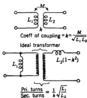
FIG. 10-6.—Equivalent circuit for practical transformer, in terms of ideal transformer.
