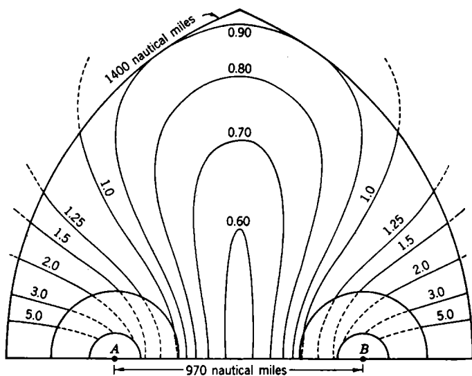
FIG. 5-23.—A contour diagram showing, as a function of the geographic position with respect to the transmitting stations, the probable error of a Sky-wave Synchronized Loran line of position.
