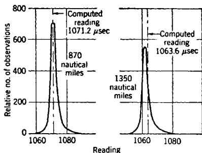
FIG. 5-18.—Two examples of the scattering of Loran sky-wave readings at medium and long distances. The average errors are four or five times those of Fig. 5.16.
