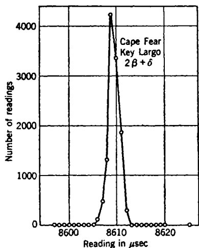
FIG. 5-36.—A distribution curve indicating the reliability with which Low Frequency Loran observations can be made at distances where the ground-wave component dominates the pulse shape.
