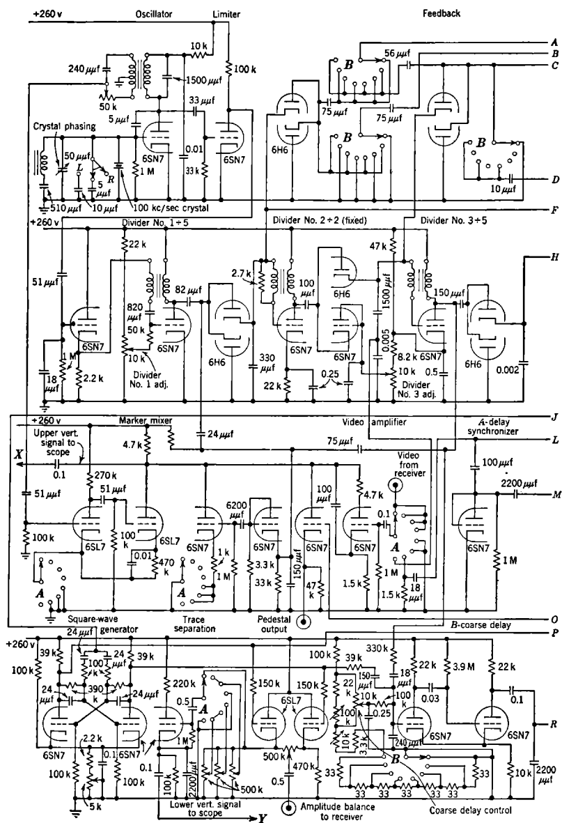
FIG. 11-13.—Schematic diagram
