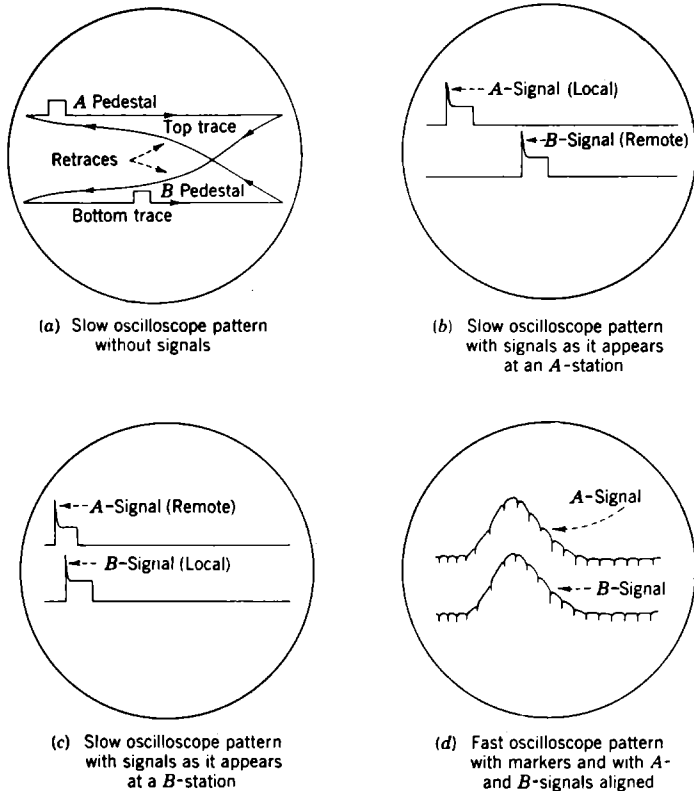
FIG. 7-5.—Basic oscilloscope patterns.
