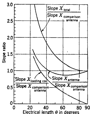
FIG. 10-13.—Reactance slopes with vertical antennas shorter than the length for first resonance.
