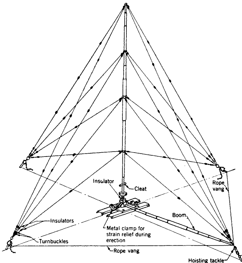
FIG. 10-34.—Perspective view of Lingo 59-ft mast.
