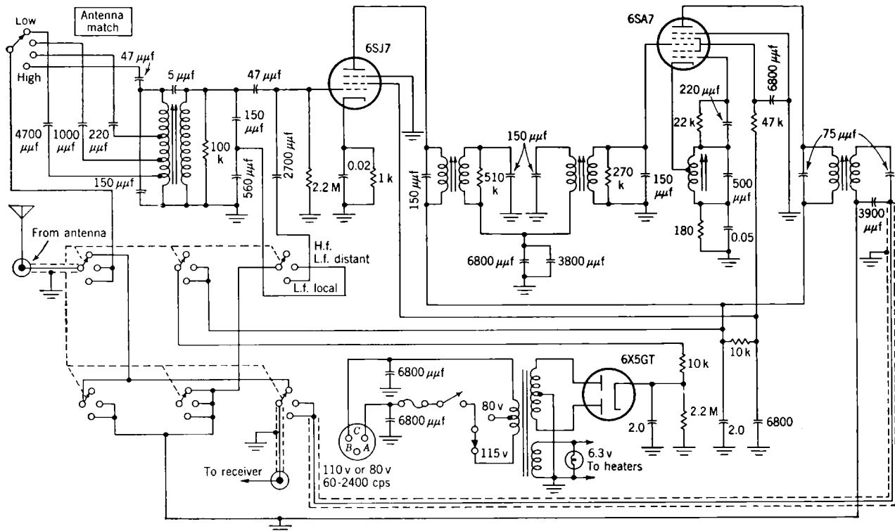
FIG. 11-10.—Schematic diagram of Low Frequency converter.
