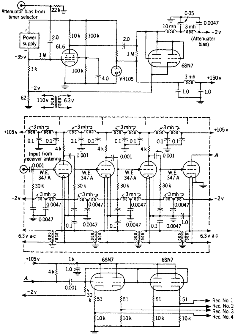
Fig. 8-8.—Schematic diagram of Low Frequency attenuator.
