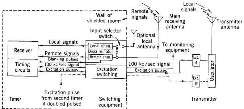
FIG. 8-6.—Block diagram of Model UM switching equipment.
