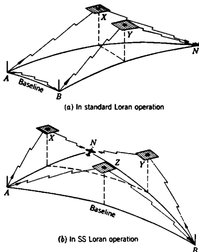
FIG. 3-23.—Sky-wave reflections.
