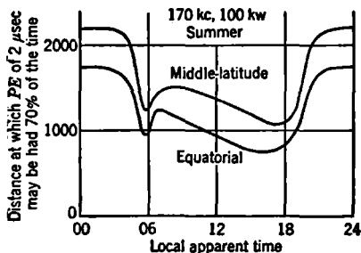
FIG. 5-4.—The approximate diurnal variation of the useful range of 100-kw Low Frequency Loran signal for tropical and temperate summertime conditions. The curves are drawn for a high degree of Loran accuracy. Useful results can be had at ranges 200 to 400 miles greater than those shown.
