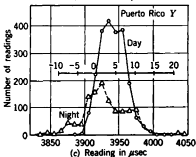
FIG. 5-42.—Distribution curves, similar to those of Fig. 5-39, of Low Frequency Loran readings at Puerto Rico.
