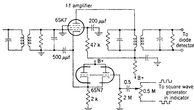
FIG. 12-1.—Early gain-balance circuit.
