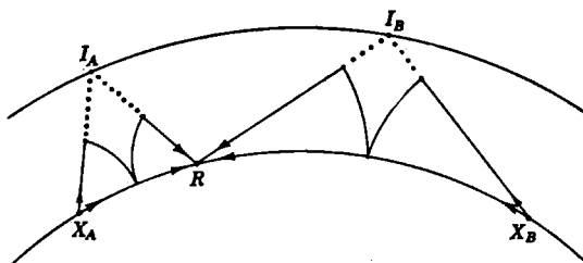
FIG. 3-5.—The sky-wave transmission delay.
