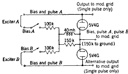
FIG. 9-5.—Simple diagram of mixer circuit.
