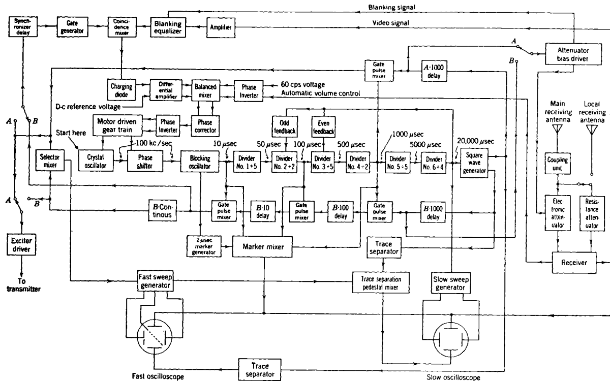
FIG. 7-12.—Block diagram of Model UE-1 timer.
