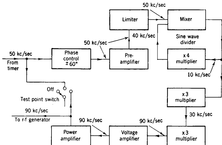
FIG. 9-12.—Block diagram of 90-kc/sec generator.
