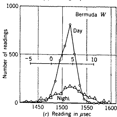
FIG. 5-39.—The distribution curves of the three Low Frequency Loran readings at Bermuda. In each case a subsidiary abscissa scale has been appended with its zero at the reading computed without benefit of sky-wave corrections. The subsidiary scale gives the line-of-position error in nautical miles.
