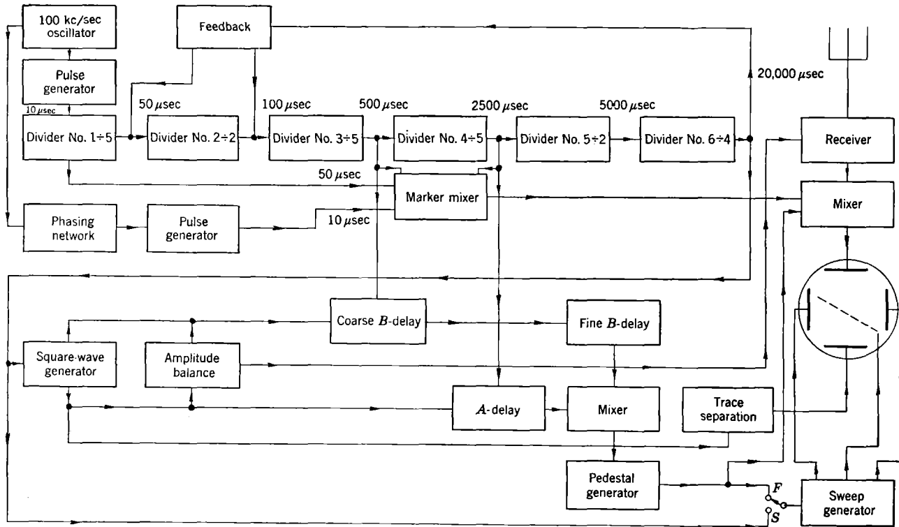
FIG. 11-11.—Block diagram of Model AN/APN-4 receiver-indicator.
