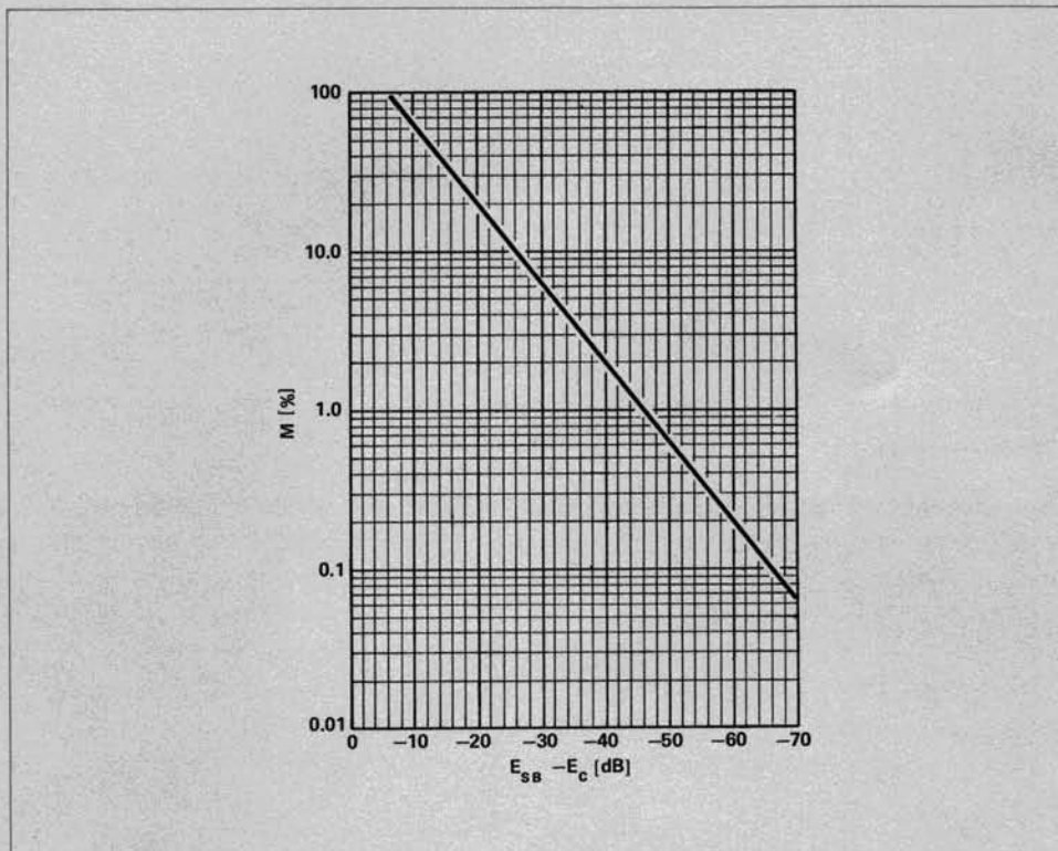
Figure 4. Modulation percentage M vs. Sideband level (Log Display).
