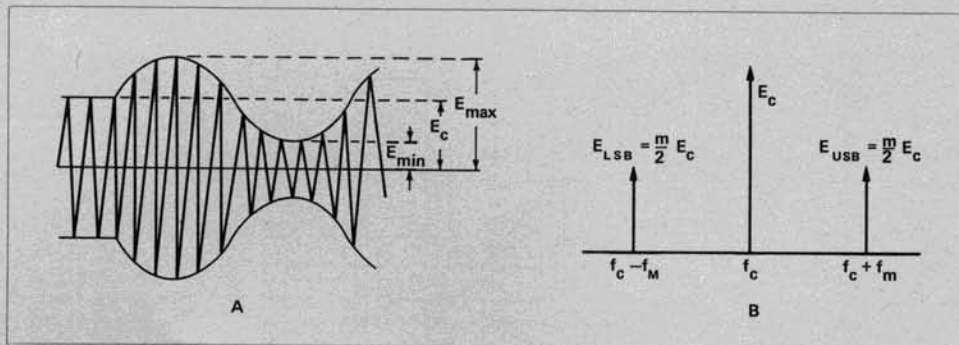
Figure 2. Calculation of degree of amplitude modulation from time domain and frequency domain displays.
