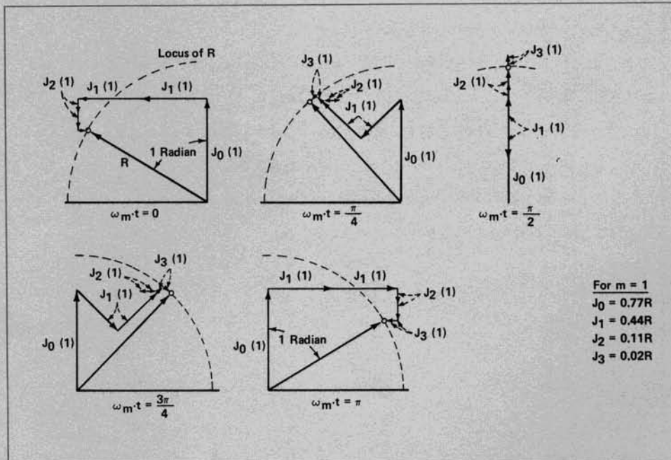
Figure I-6. Phasor diagrams of an FM signal with a modulation index m = 1 . Different diagrams corresponding to different points in the cycle of the sinusoidal modulating wave.
