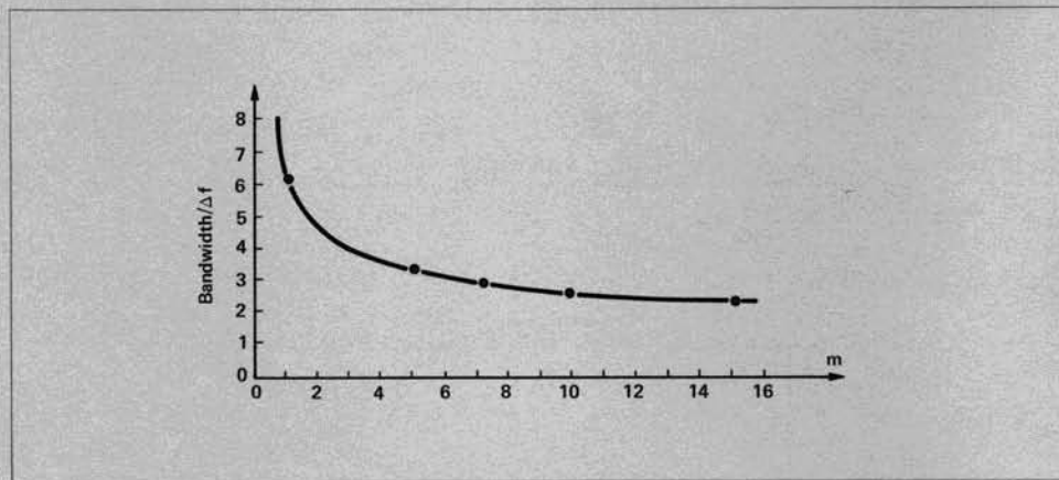
Figure 16. Bandwidth requirements vs. modulation index, m .
