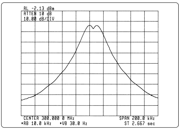
Figure 12. Two equal- amplitude sinusoids separated by the 3 dB BW of the selected IF filter can be resolved
