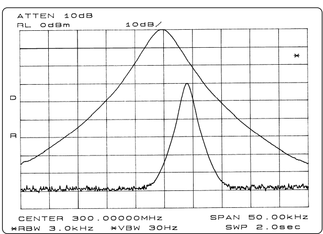
Figure 13. A low-level signal can be lost under skirt of the response to a larger signal
