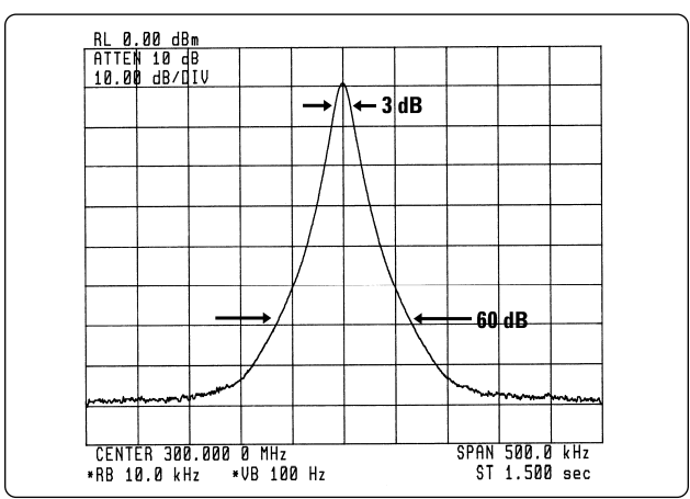
Figure 14. Bandwidth selectivity, ratio of 60 dB to 3 dB bandwidths, helps determine resolving power for unequal sinusoids
