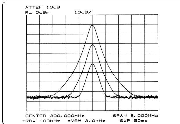
Figure 41. Some spectrum analyzers change reference level when RF attenuator is changed, so an input signal moves on the display, but the analyzer's noise does not
