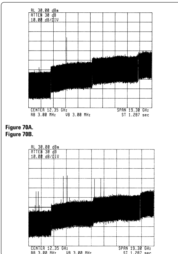
Figure 70. Preselection makes wide spans practical
