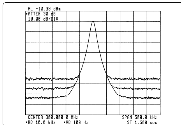
Figure 42. Other analyzers keep reference level constant by changing IF gain, so as RF attenuator is changed, the analyzer's noise moves, but an input signal does not
