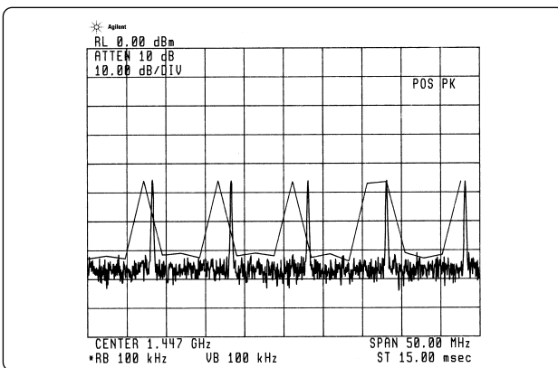
Figure 35. Pos peak display mode versus actual comb
