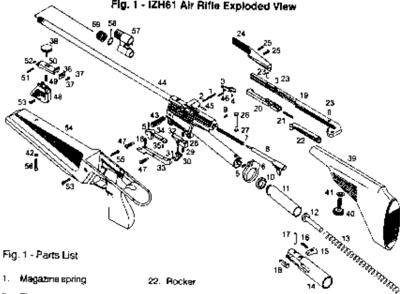
Fig. 1 - IZH61 Air Rifle Exploded View
