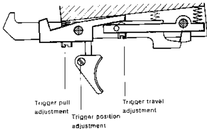
Fig. 2: IZH61 The Trigger Mechanism
