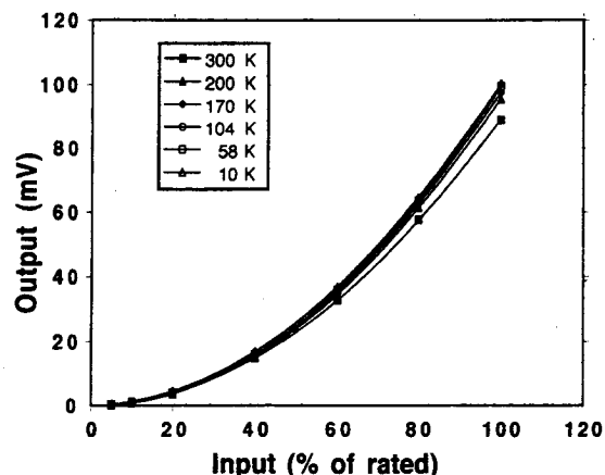
Fig. 7. Output emf of thin-film MJTC versus input level at various temperatures.
