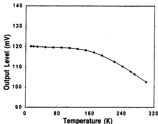
Fig. 6. Output emf of thin-film MJTC versus ambient temperature for fixed input power.
