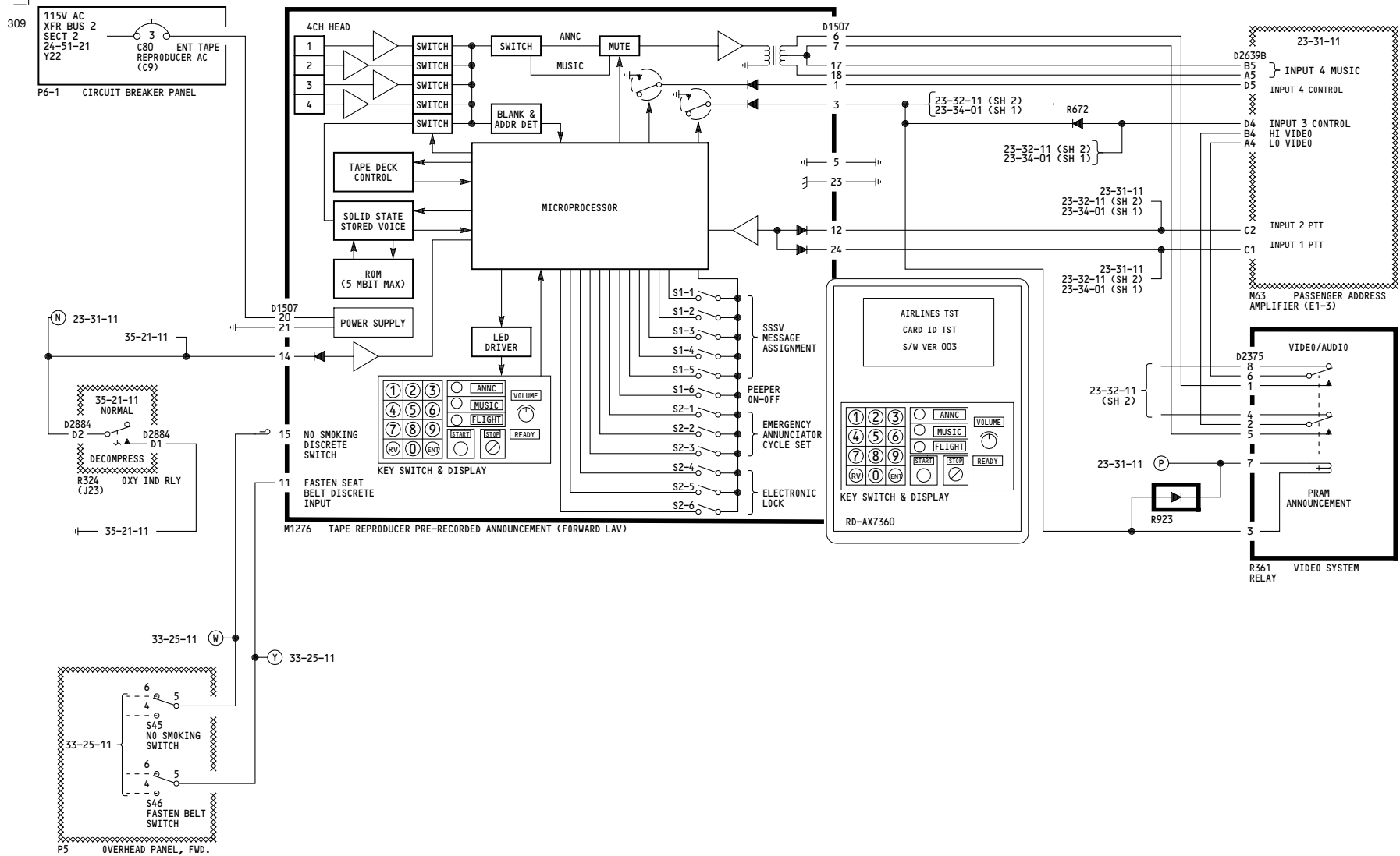
YK901-YM670 PRE-RECORDER ANNOUNCEMENT MACHINE D280A203
