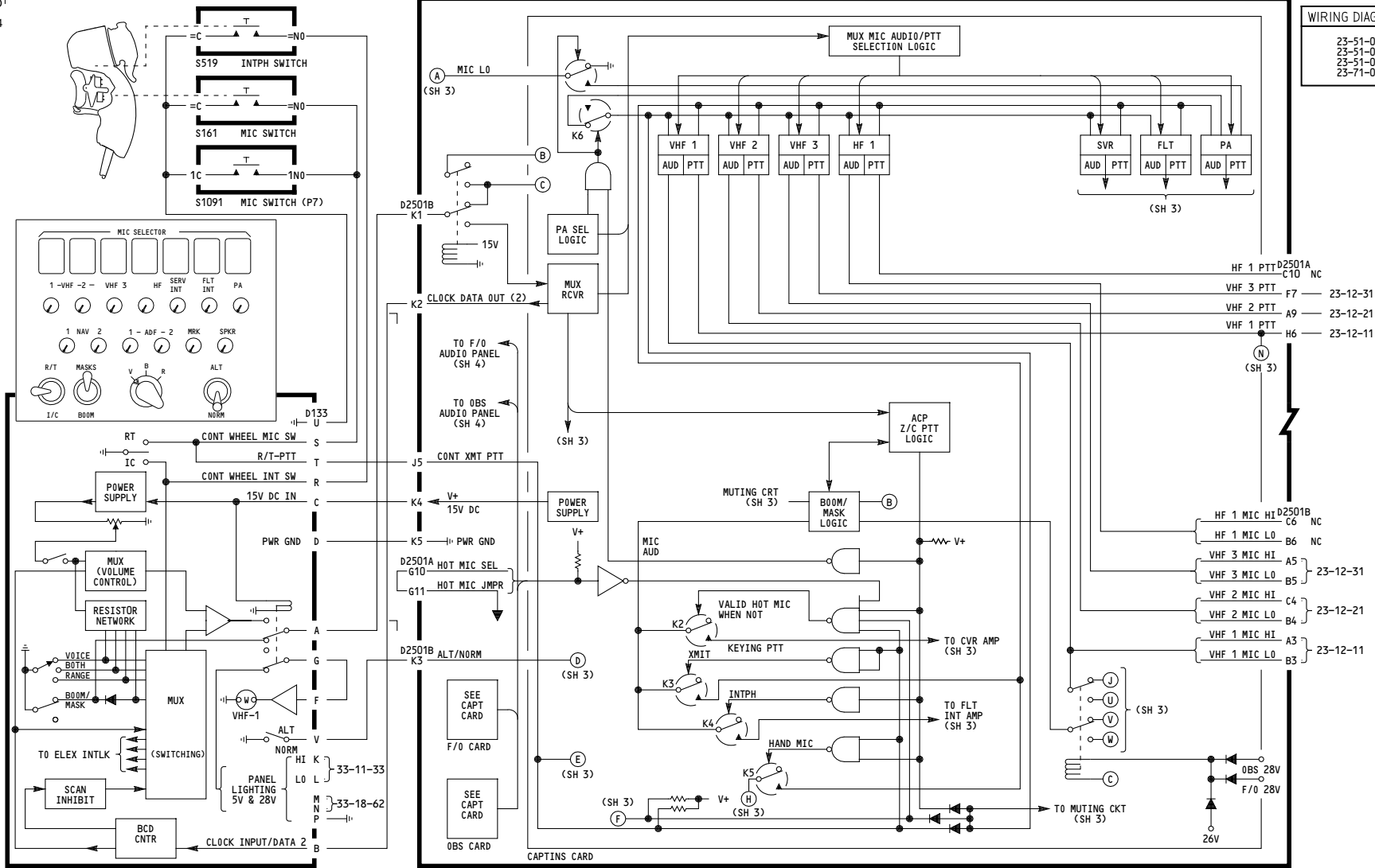
P8-6 CAPT AUDIO CONTROL PANEL
