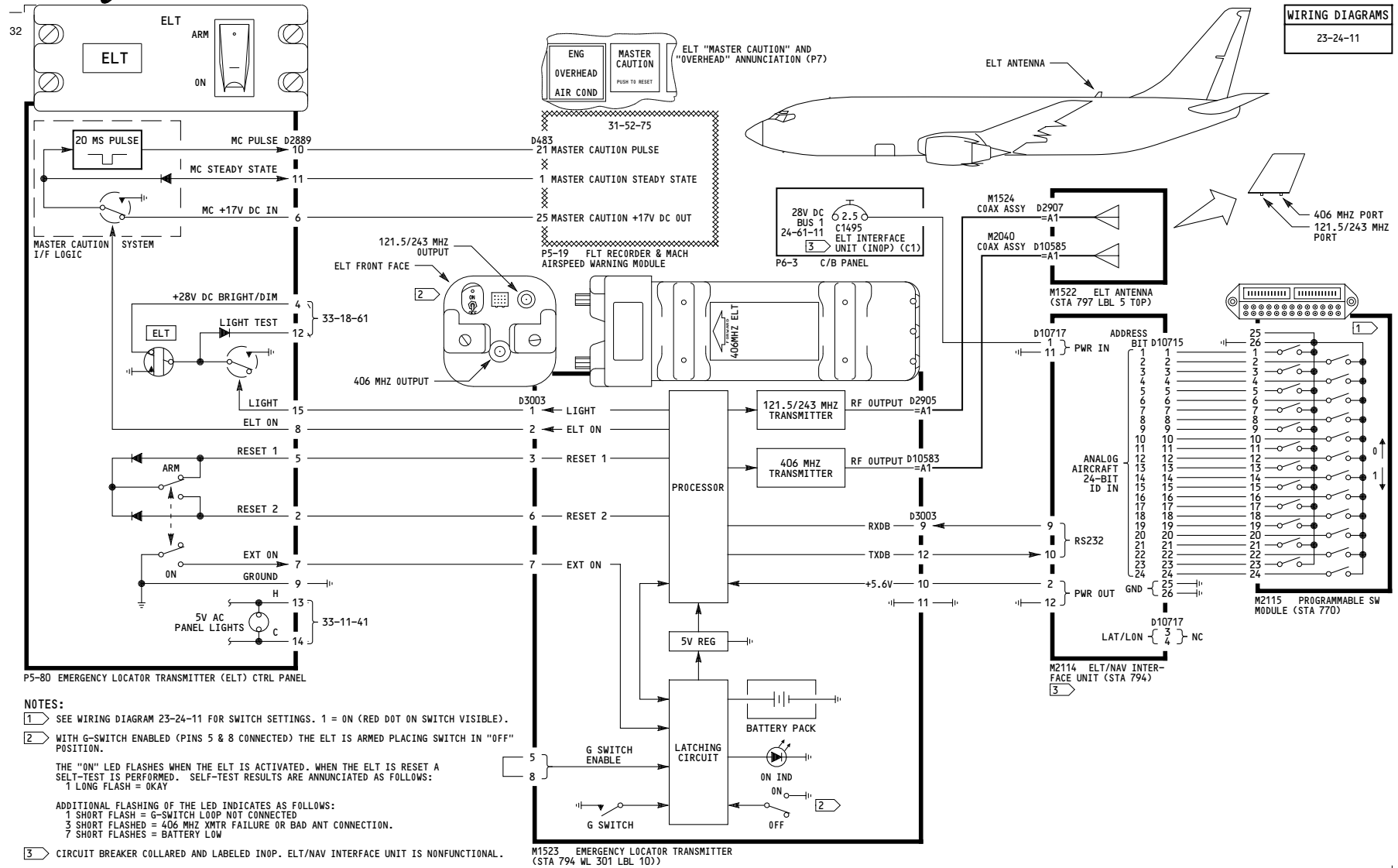
M1523 EMERGENCY LOCATOR TRANSMITTER (STA 794 WL 301 LBL 10)
