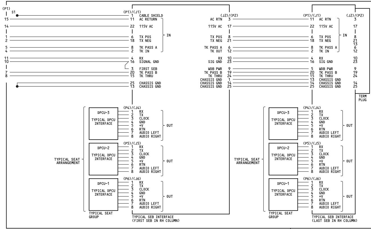
TYPICAL SIDEWALL TO SEAT INTERFACE (FOR LEFT AND RIGHT COLUMNS)
