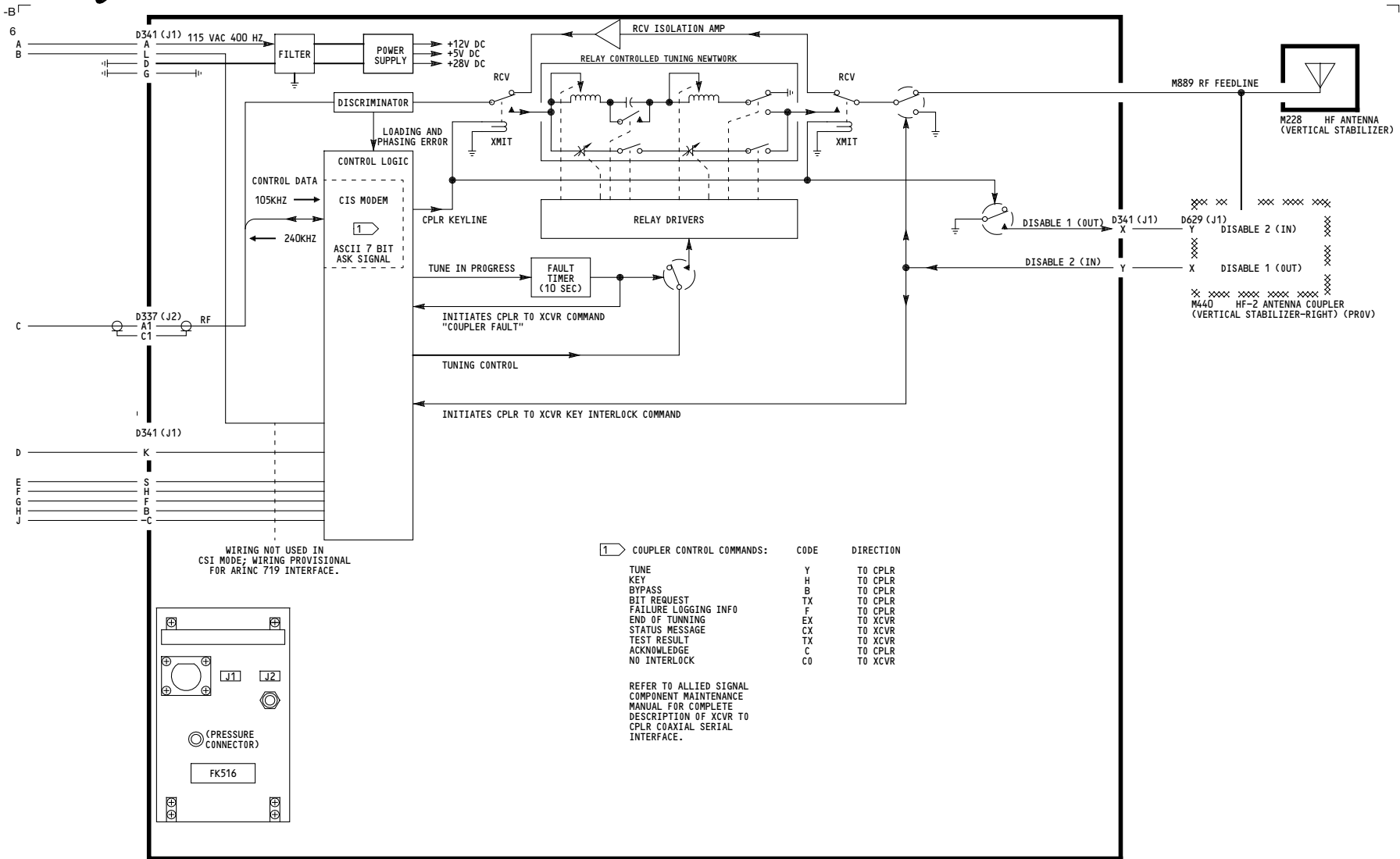
M227 HF-1 ANTENNA COUPLER (VERTICAL STABILIZER - LEFT)
