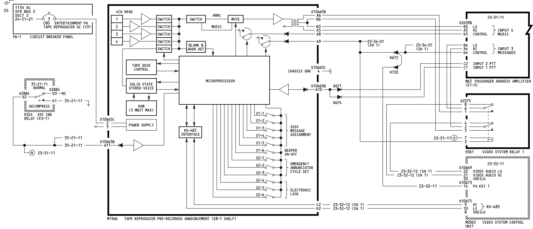
WIRING DIAGRAMS 23-31-06
