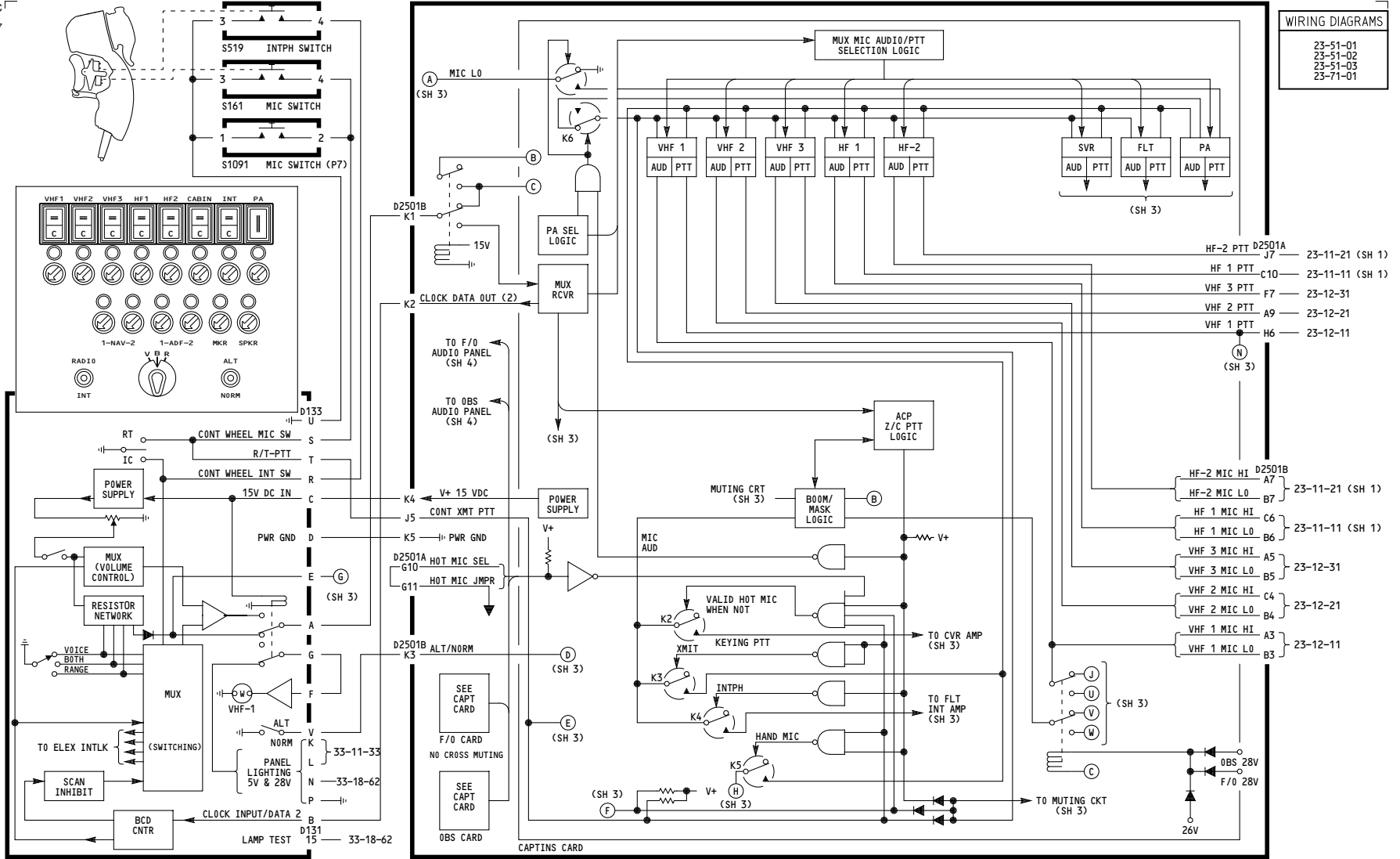
P8-6 CAPT AUDIO CONTROL PANEL
