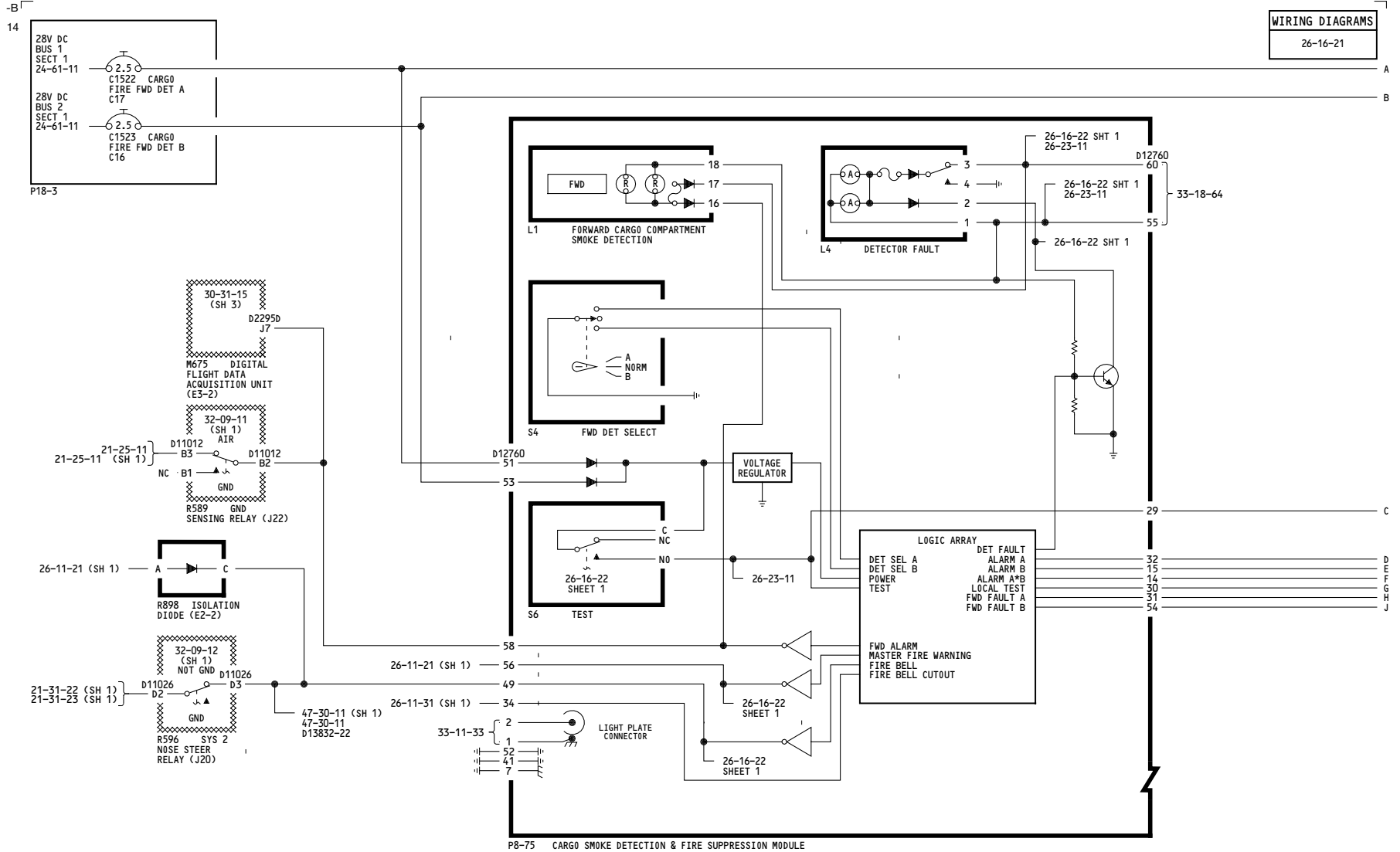
P8-75 CARGO SMOKE DETECTION & FIRE SUPPRESSION MODULE
