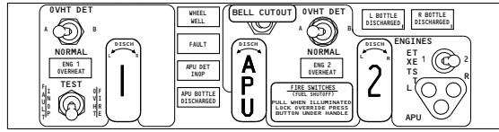
ENGINE AND APU FIRE CONTROL MODULE
