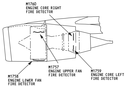
ENGINE FIRE DETECTORS (26-11-11, 26-11-21)
