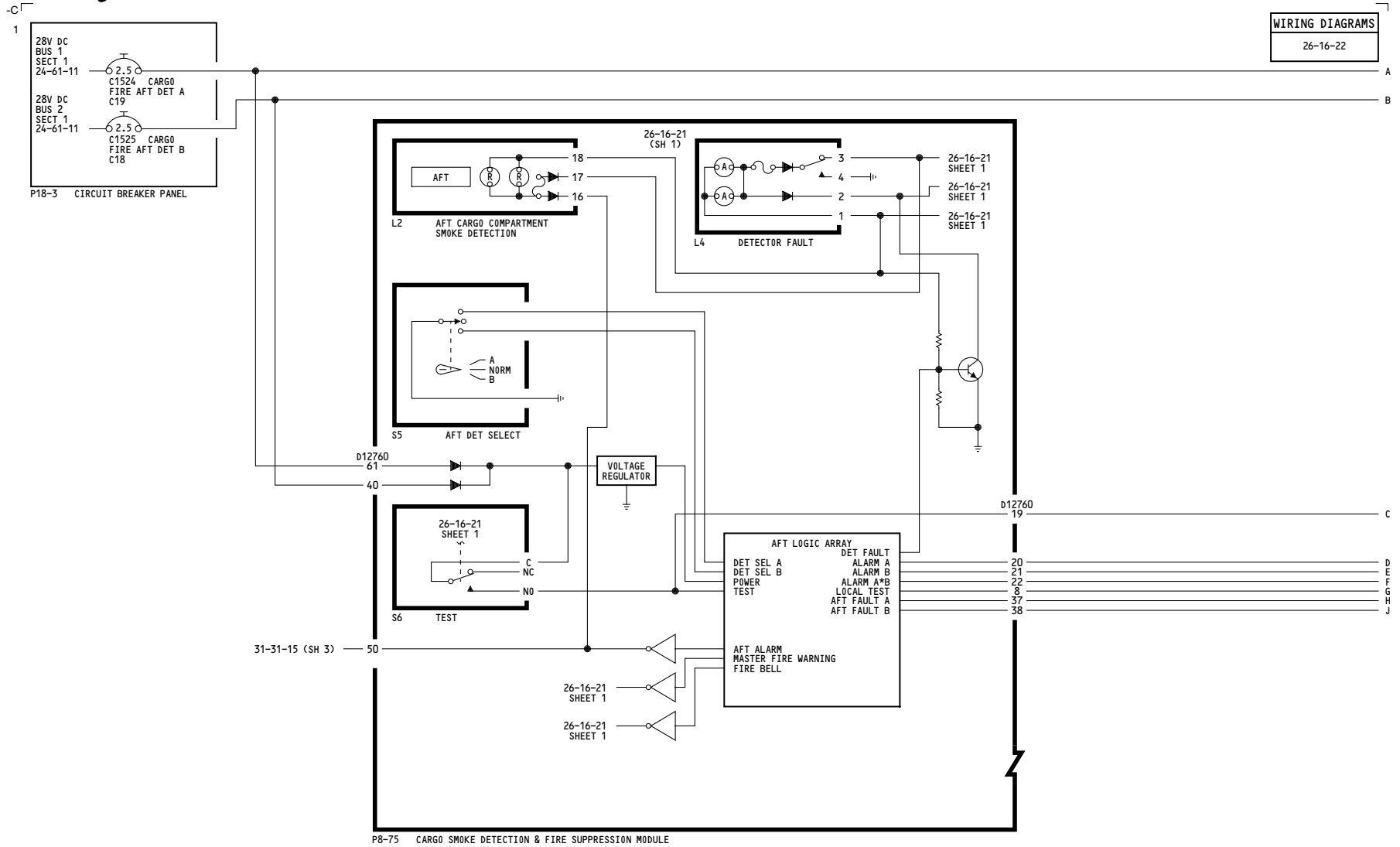
P8-75 CARGO SMOKE DETECTION & FIRE SUPPRESSION MODULE
