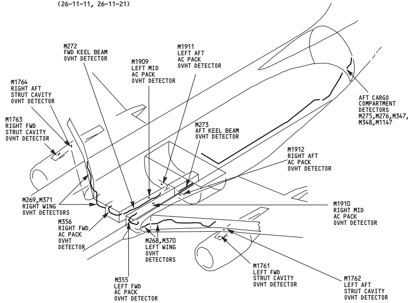
COMPARTMENT OVERHEAT DETECTORS (26-12-11)
