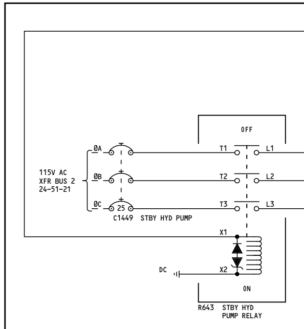
P92 POWER DISTRIBUTION PANEL 2
