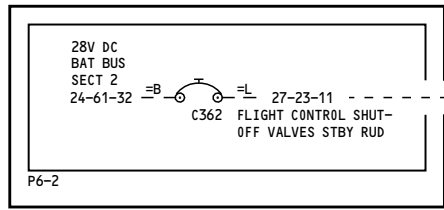
P6 LOAD CONTROL CENTER - RIGHT
