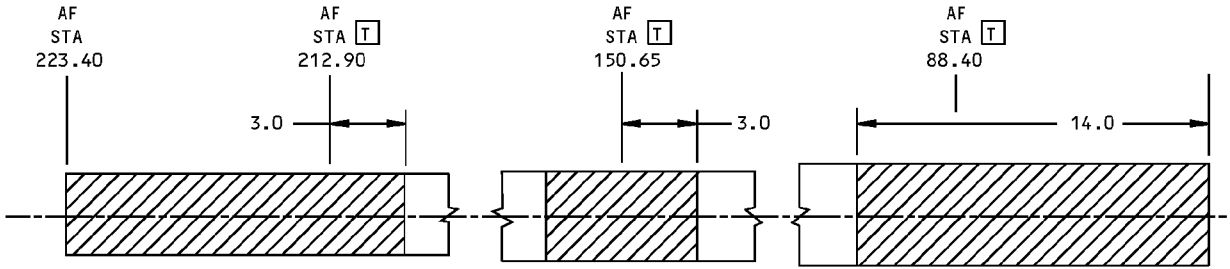
AFT FLAP SPAR INBOARD TRAILING EDGE FLAP DETAIL V
