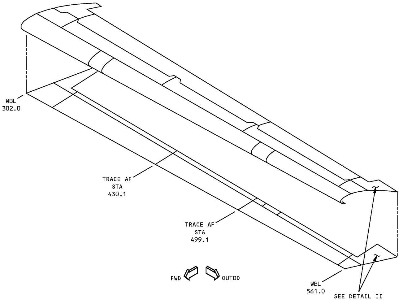
MAIN FLAP - OUTBOARD TRAILING EDGE FLAP DETAIL I
