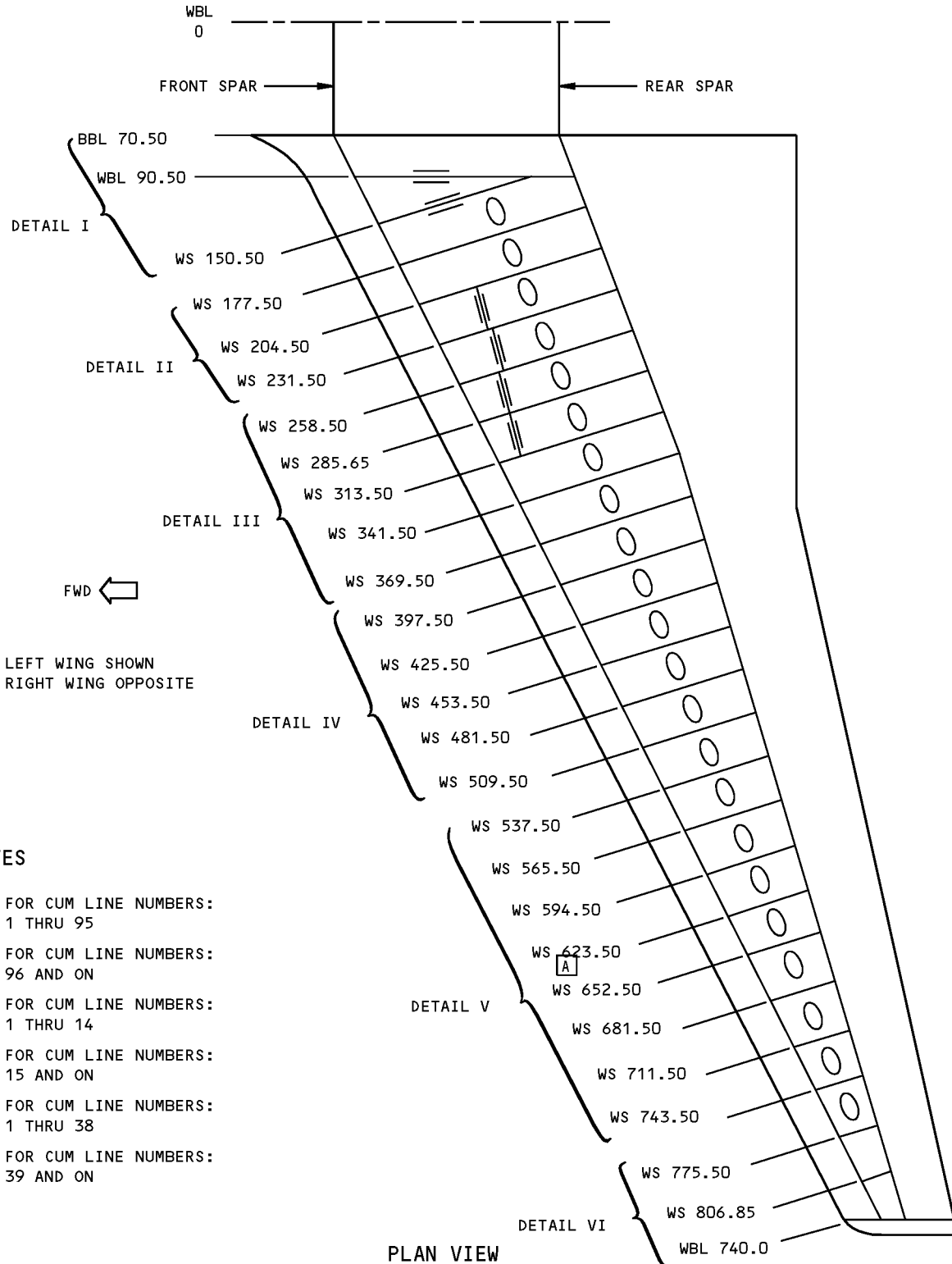
Outer Wing Rib Identification Figure 1 (Sheet 1 of 12)
