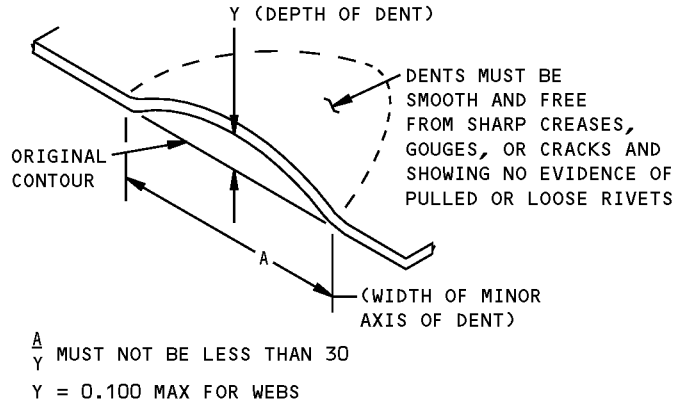
ALLOWABLE DAMAGE FOR DENT DETAIL XI
