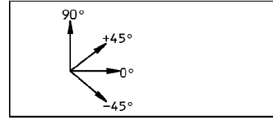
PLY ORIENTATION DIAGRAM SEE TABLE V FOR INDIVIDUAL PLY ORIENTATION AND MATERIALS
