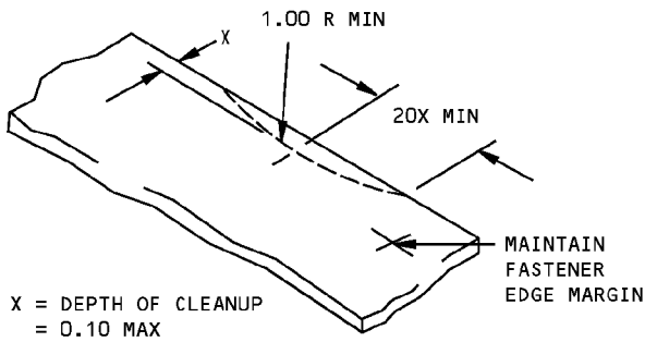
REMOVAL OF NICK OR CRACK DAMAGE ON AN EDGE DETAIL IX
