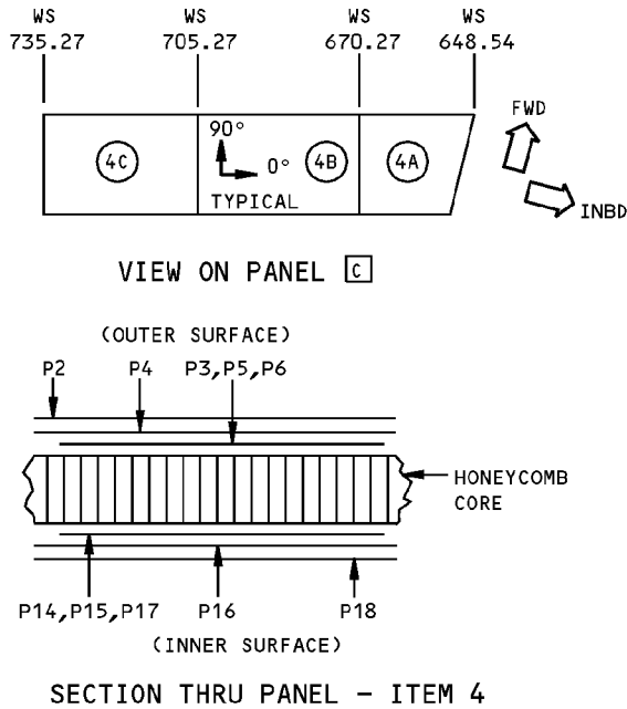
DETAIL XIII
