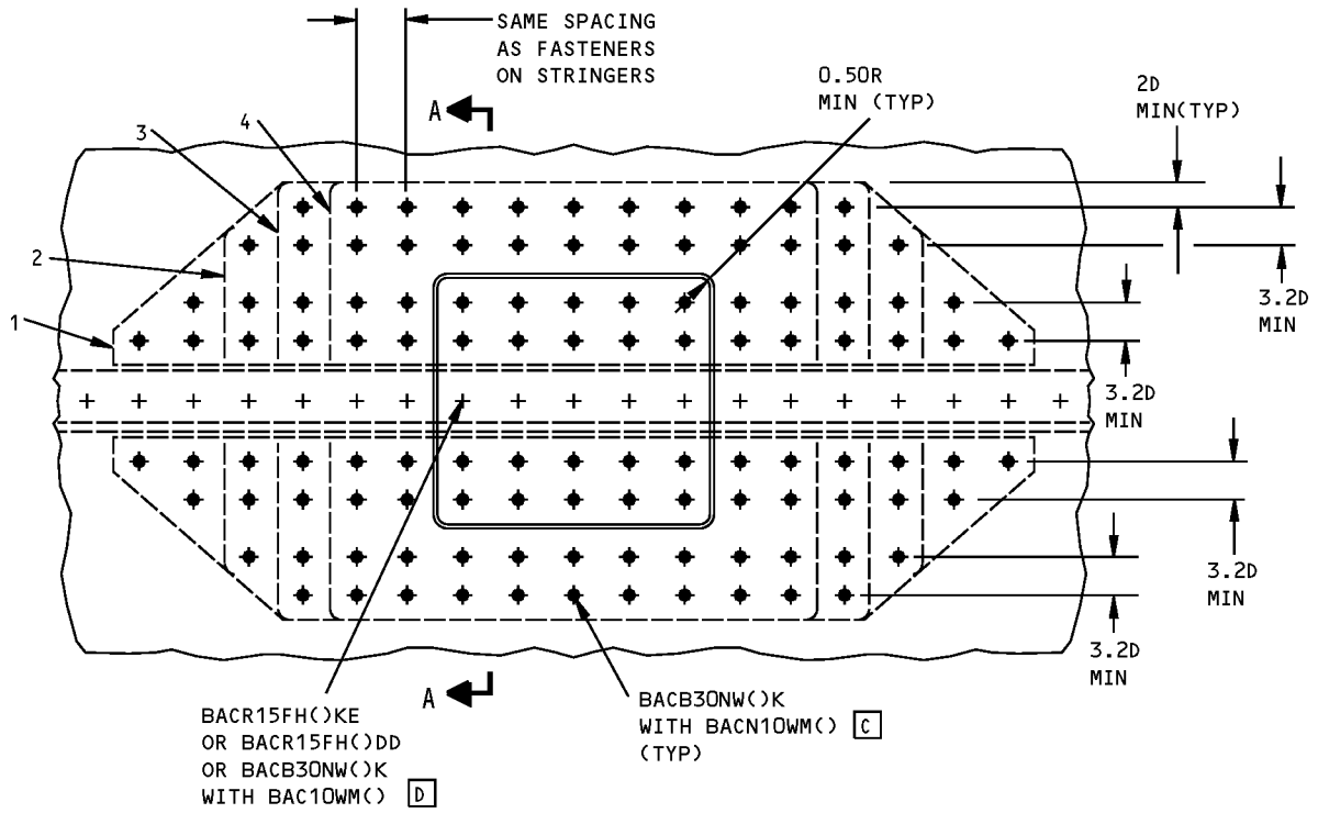
DETAIL I
