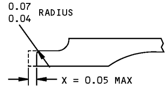
TYPICAL BLENDOUT AROUND DOOR CUTOUT PERIPHERY SECTION B-B
