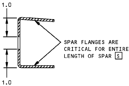
SECTION THRU SPAR - OUTBOARD FLAP
