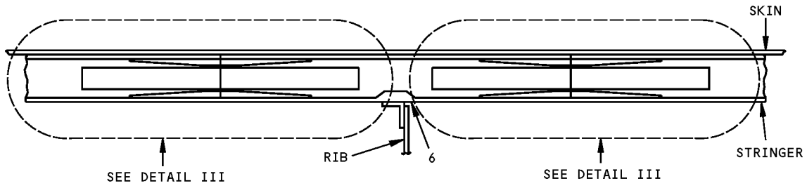
ALTERNATE REPAIR INSTALLATION FOR DAMAGE NEAR RIBS
