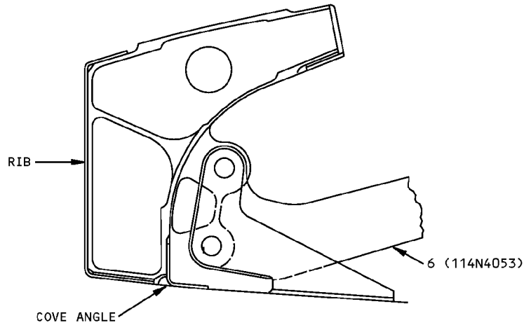
DETAIL V
