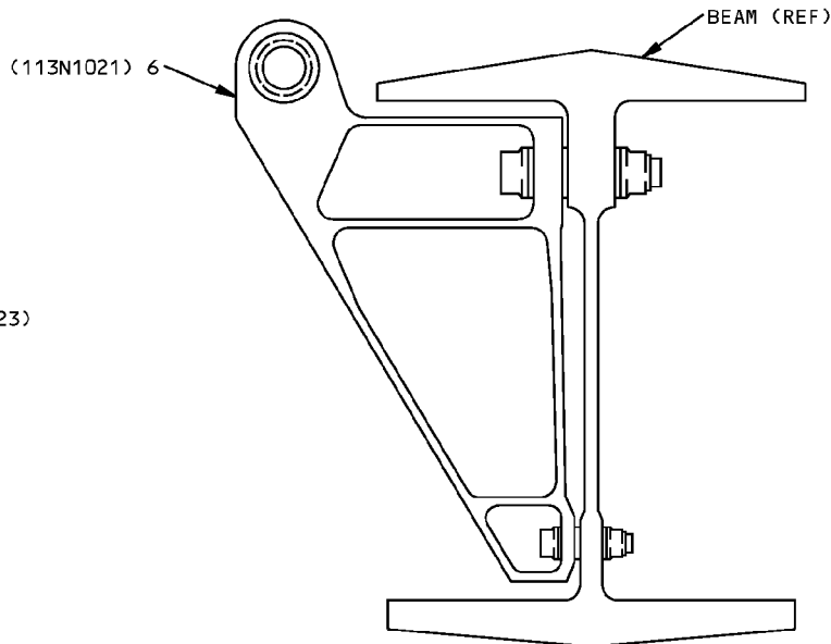
SECTION B-B
