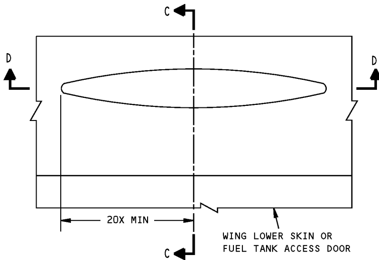
DAMAGE REMOVAL ON THE MILLED STEP IN THE SKIN
