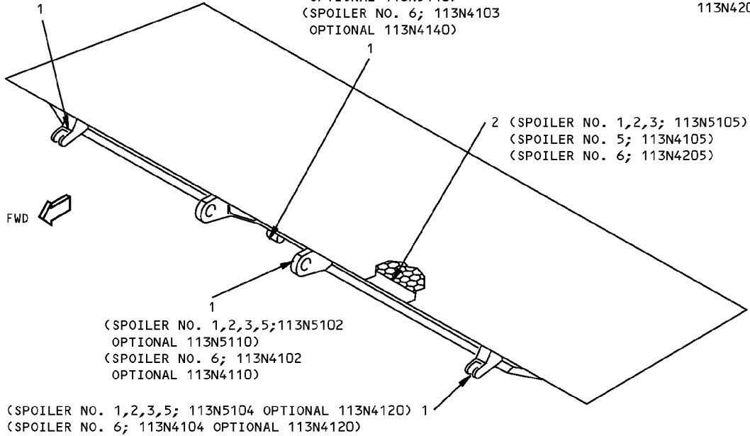
SPOILER NO. 1,2,3,5,6 DETAIL I J
