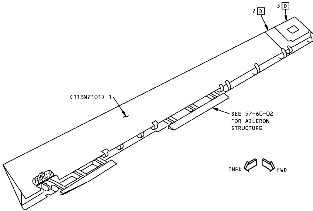
DETAIL I
