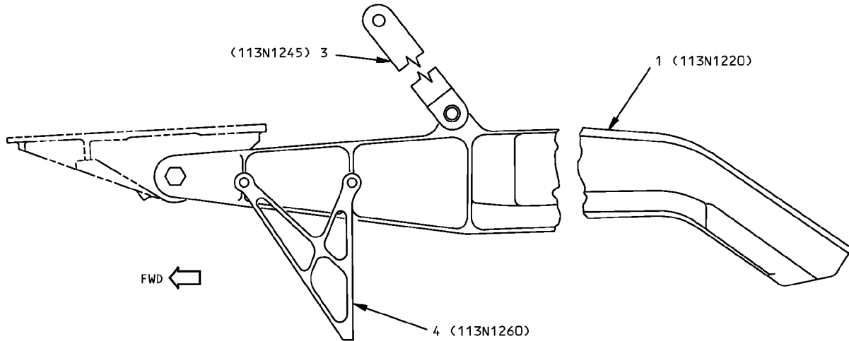
OUTBD TRACK - INBD FLAP DETAIL III
