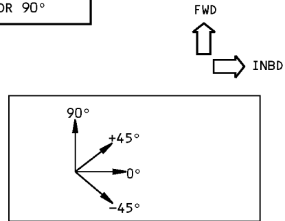
PLY ORIENTATION DIAGRAM SEE TABLE II FOR INDIVIDUAL PLY ORIENTATION AND MATERIALS
