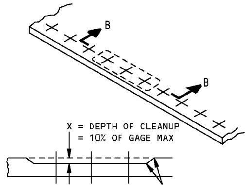
REMOVAL OF NICK, GOUGE AND SCRATCH DAMAGE ON A SURFACE DETAIL VI
