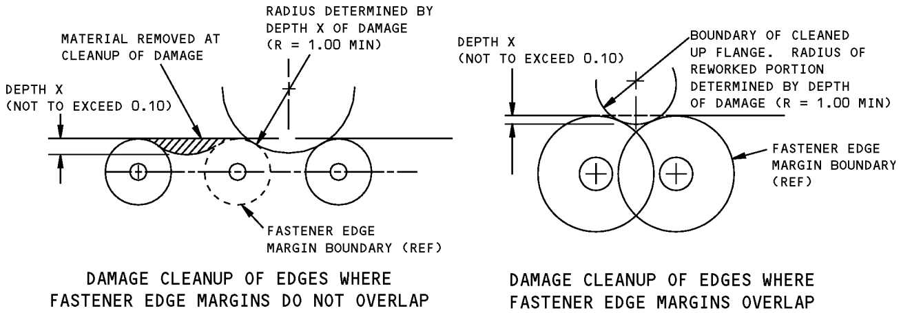
DETAIL I
