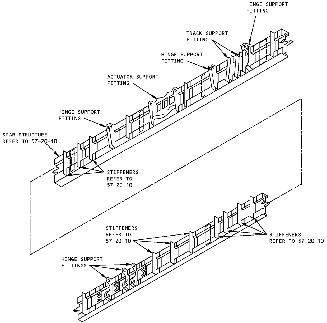
REAR SPAR – REAR VIEW DETAIL IV
