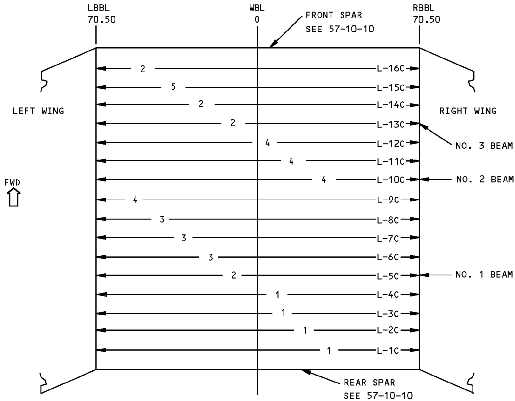
PLAN VIEW ON LOWER PANEL
