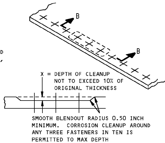
REMOVAL OF NICK, GOUGE AND SCRATCH DAMAGE ON A SURFACE DETAIL V
