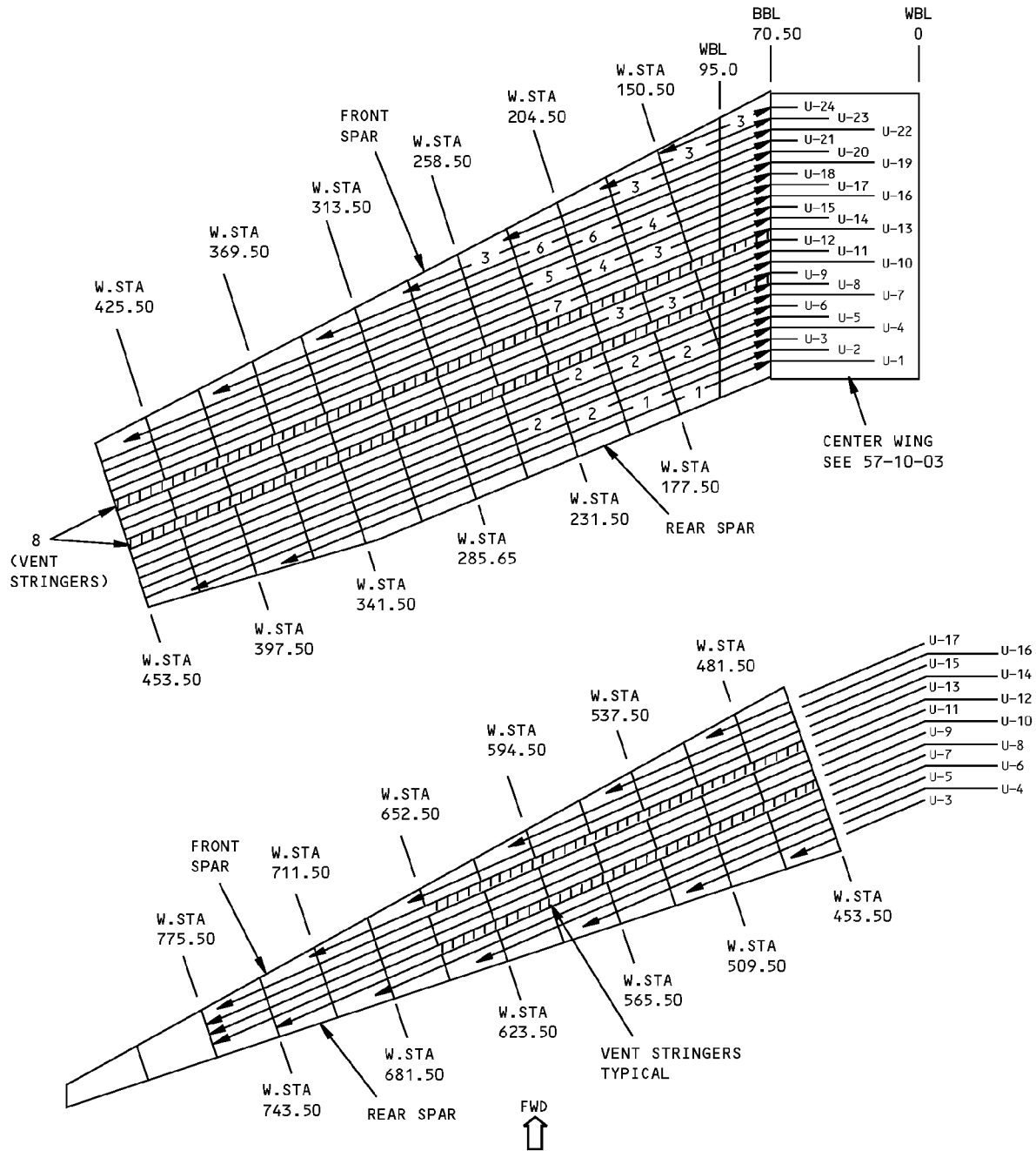
PLAN VIEW UPPER SURFACE LEFT WING SHOWN RIGHT WING OPPOSITE DETAIL I
