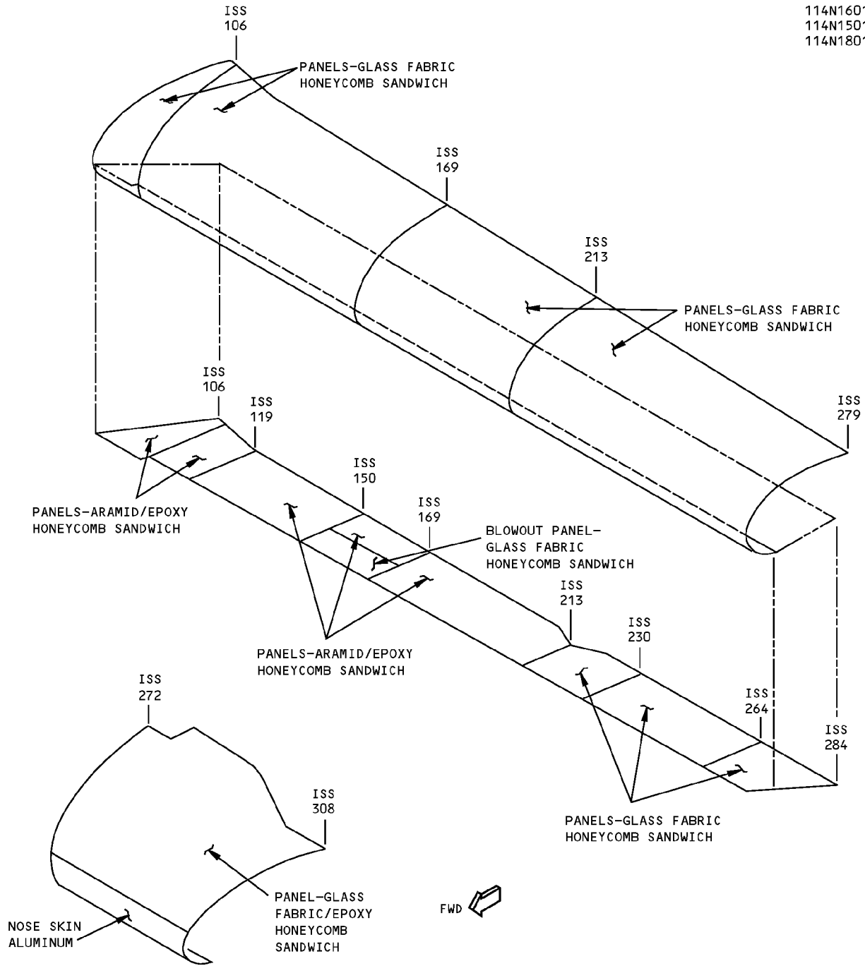
LEADING EDGE SKIN AT NACELLE
