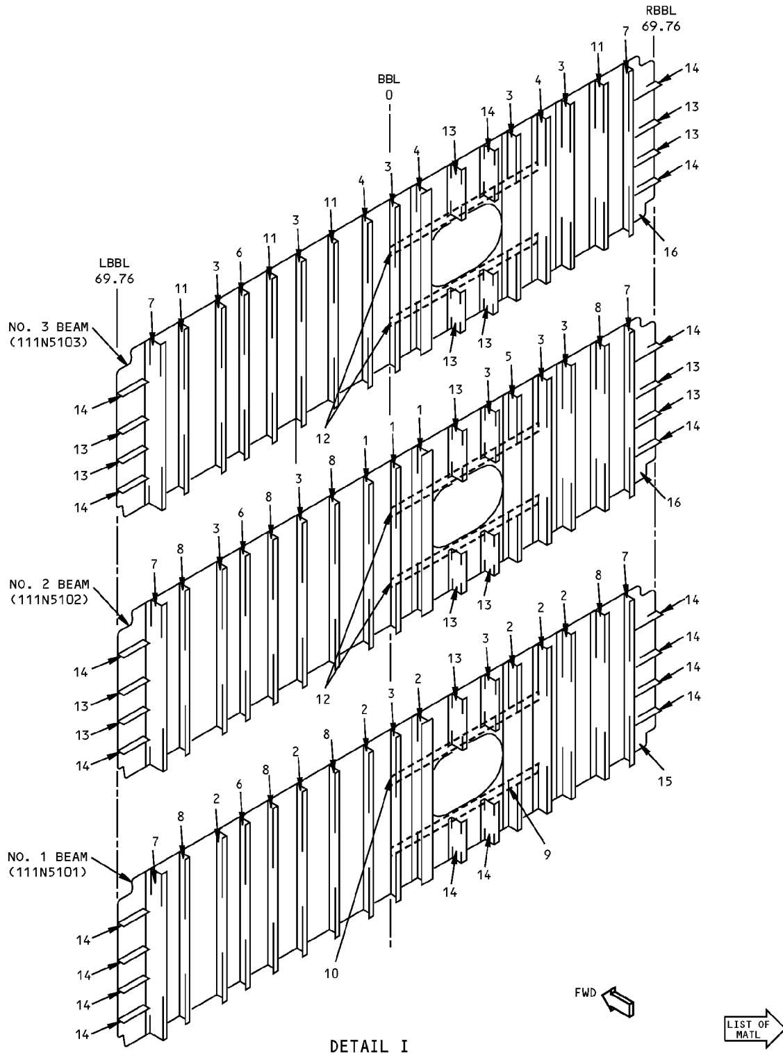
Center Section Spanwise Beam Identification Figure 1 (Sheet 2 of 3)
