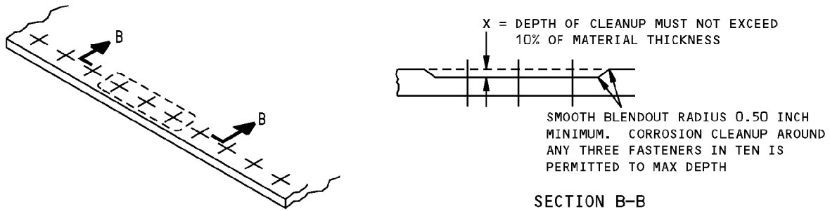
CORROSION CLEANUP DETAIL IV
