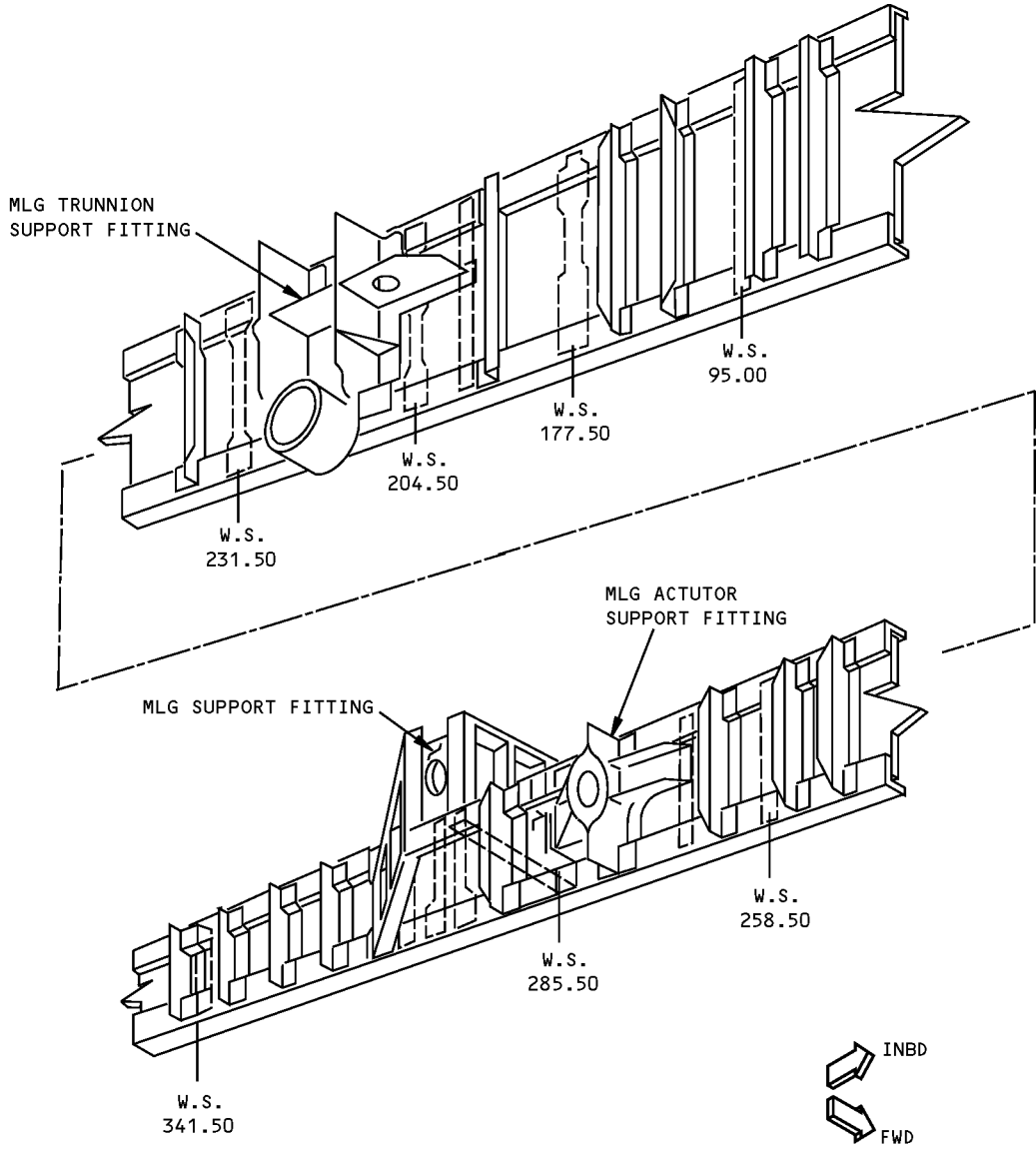
DETAIL I
