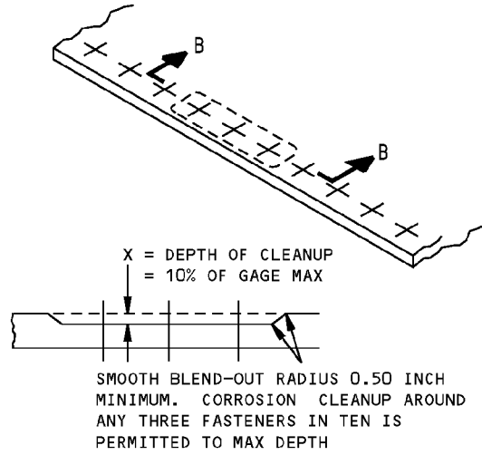
CORROSION CLEANUP DETAIL VII
