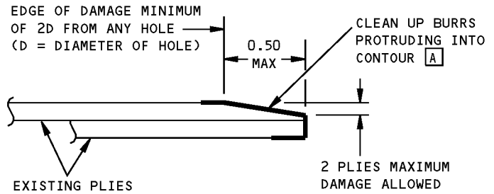
DAMAGE CLEANUP AND SEALING OF EDGE EROSION DETAIL III
