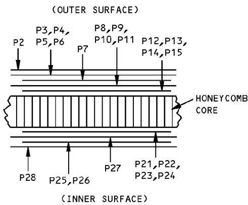
SECTION THRU PANEL - ITEM 4 U
