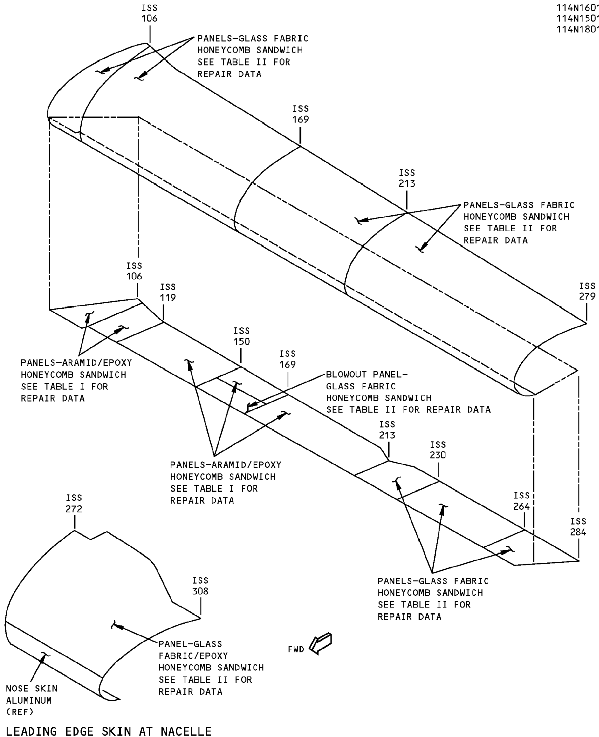
Wing Fixed Leading Edge Skin Repairs Figure 201 (Sheet 2 of 8)
