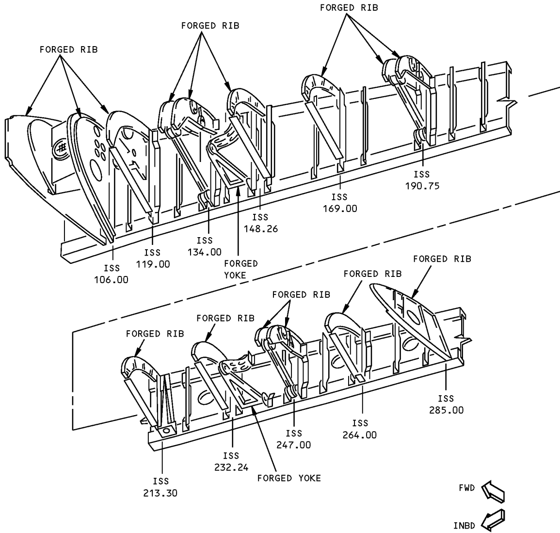
DETAIL I
