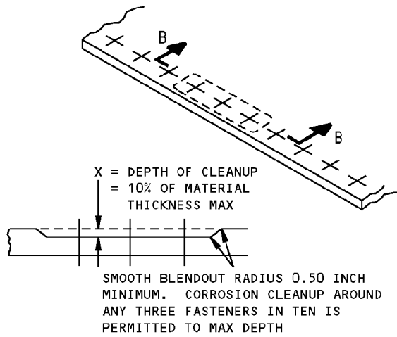
CORROSION CLEANUP DETAIL X
