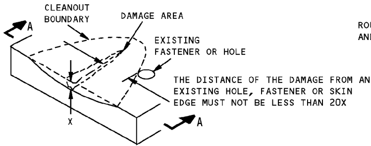
REMOVAL OF NICK, GOUGE AND SCRATCH DAMAGE ON A SURFACE DETAIL VIII
