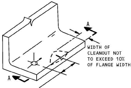
REMOVAL OF NICK OR CRACK DAMAGE ON AN EDGE DETAIL V
