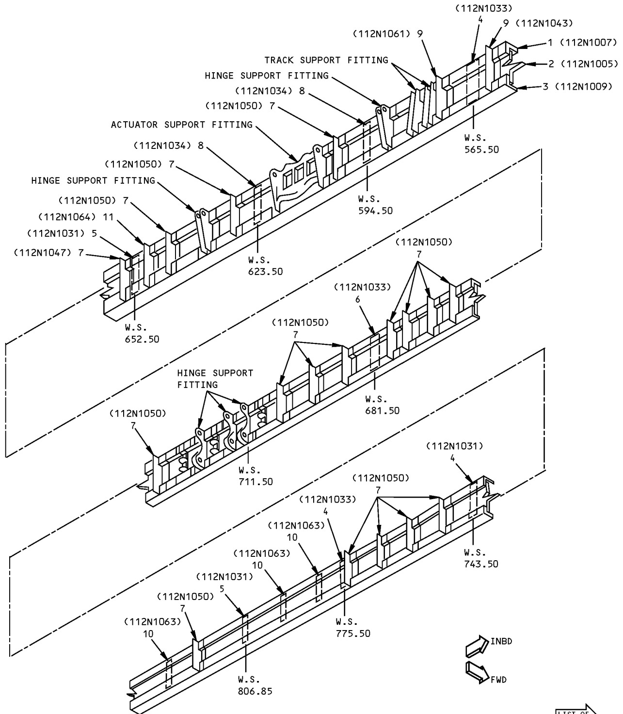
DETAIL III
