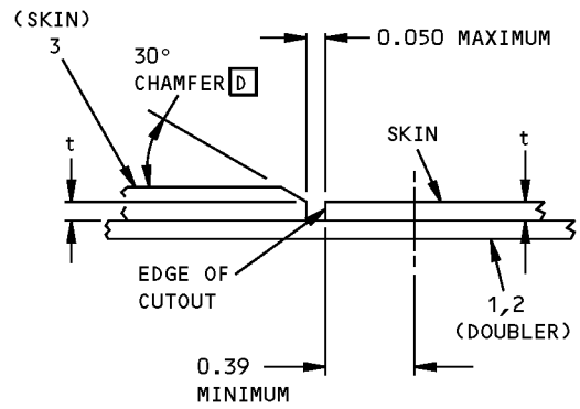
DETAIL II
