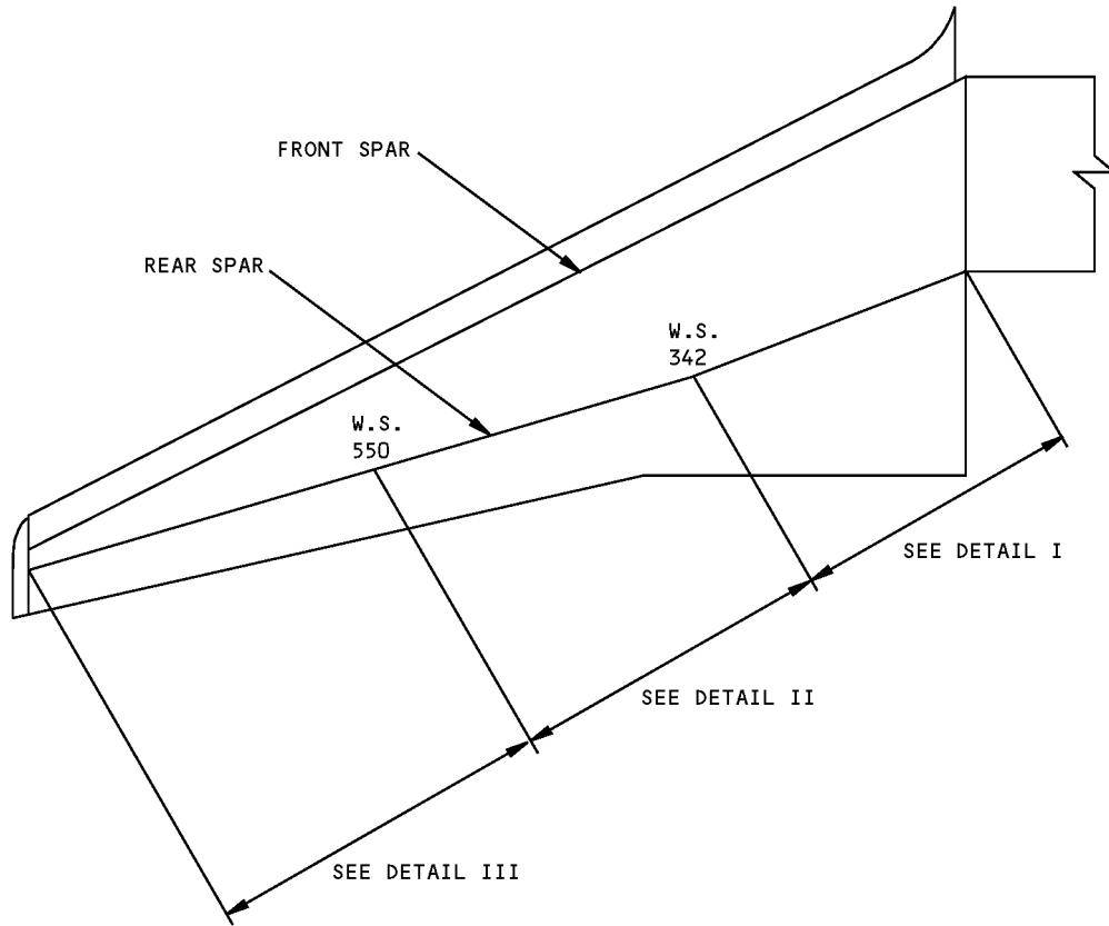
Outer Wing Rear Spar Fitting Repair Figure 201 (Sheet 1 of 4)
