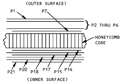
SECTION THRU PANEL - ITEM 3 X
