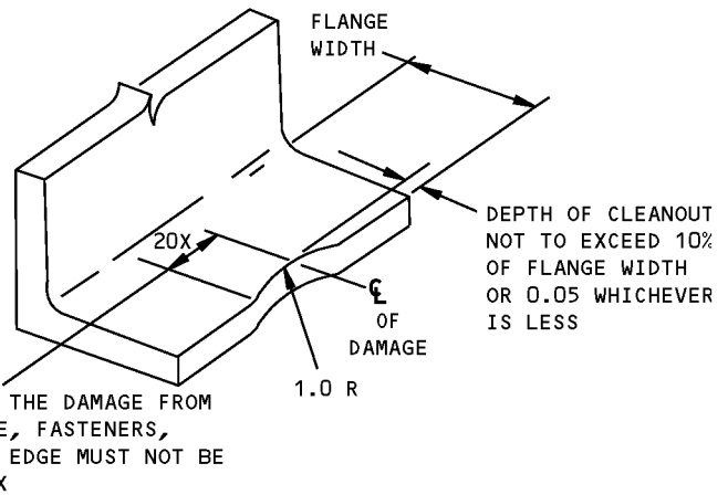
REMOVAL OF EDGE DAMAGE FROM FREE FLANGE WITHOUT FASTENERS DETAIL IV
