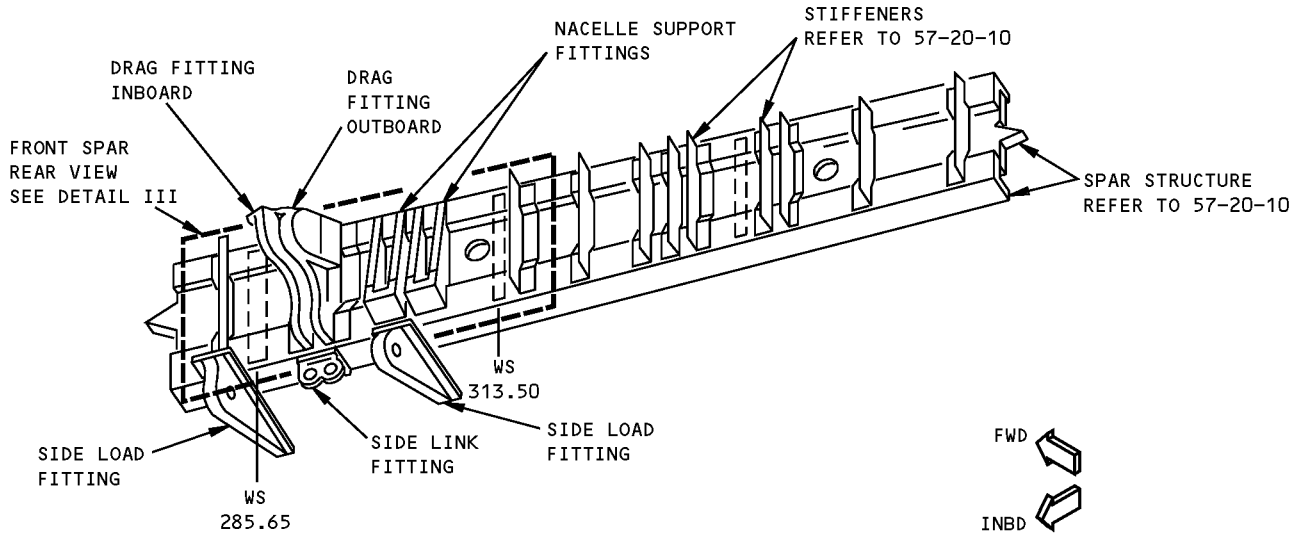
DETAIL II
