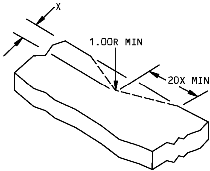
DETAIL V
