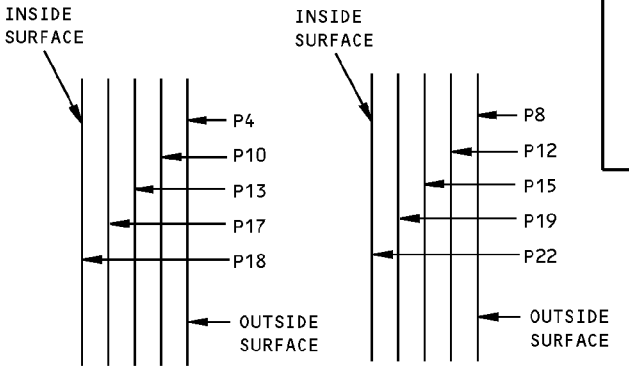
SECTION THRU SPAR SPOILER NO. 4
