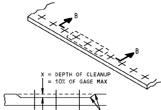
REMOVAL OF NICK, GOUGE AND SCRATCH DAMAGE ON A SURFACE DETAIL IV
