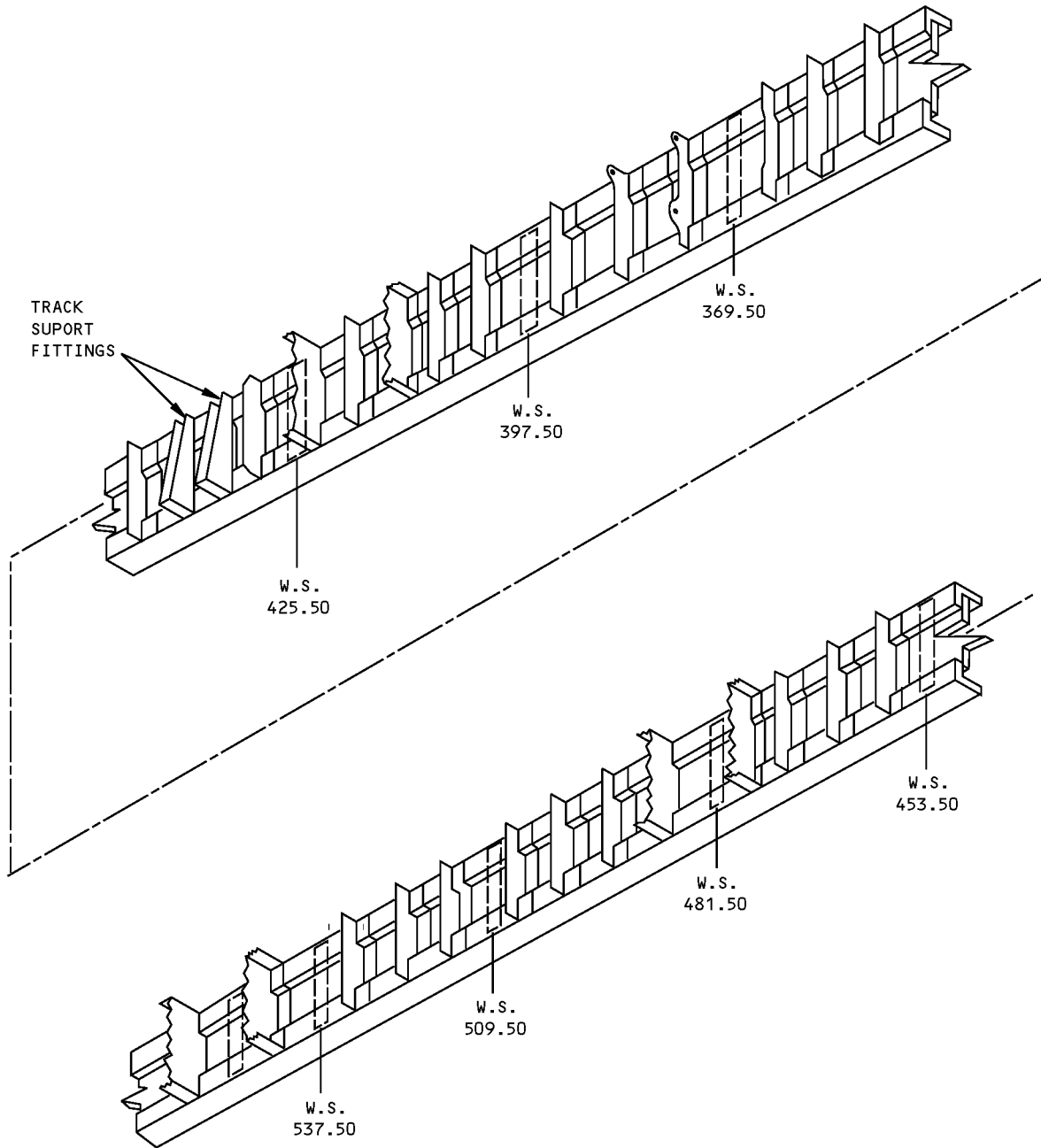
DETAIL II
