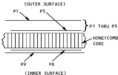
SECTION THRU PANEL - ITEM 4 T
