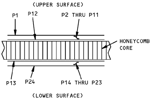
SECTION THRU HONEYCOMB PANEL SPOILERS 1,2,3,5,6
