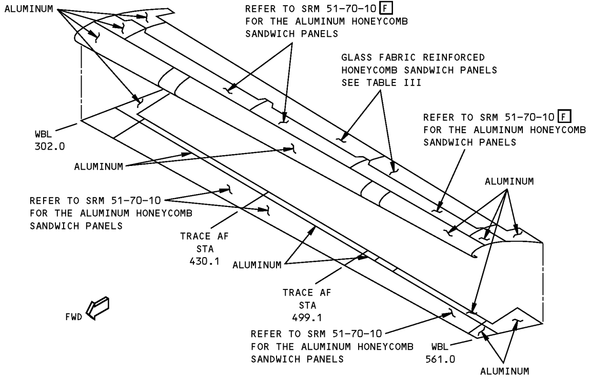
MAIN FLAP - OUTBOARD TRAILING EDGE FLAP DETAIL III
