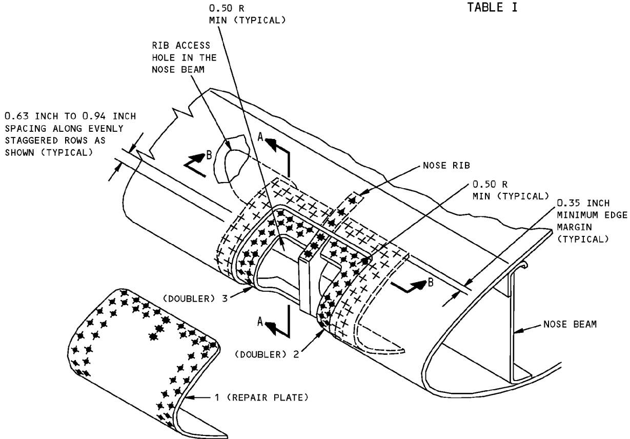
DETAIL I
