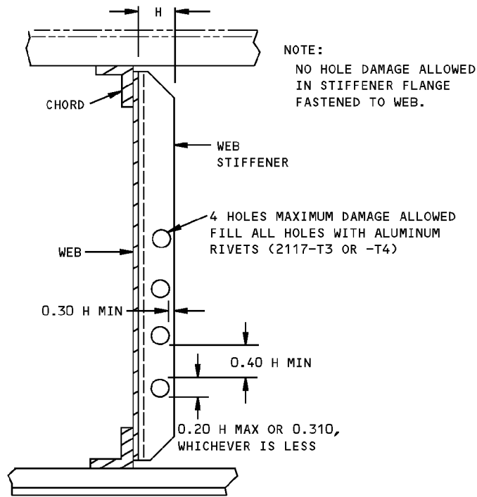
H = WIDTH OF STIFFENER FLANGE ALLOWABLE DAMAGE LIMITS FOR HOLES IN WEB STIFFENERS DETAIL V
