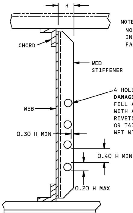
ALLOWABLE DAMAGE LIMITS FOR HOLES IN WEB STIFFENERS DETAIL X
