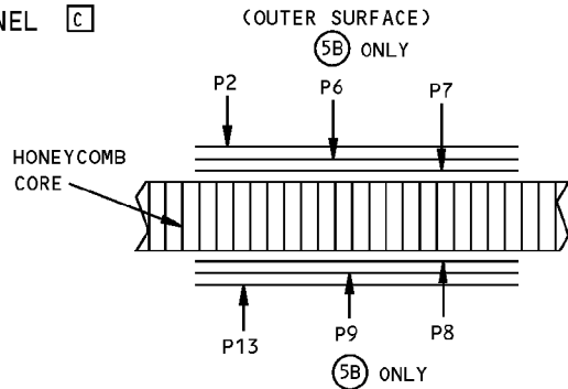
(INNER SURFACE) SECTION THRU PANEL
