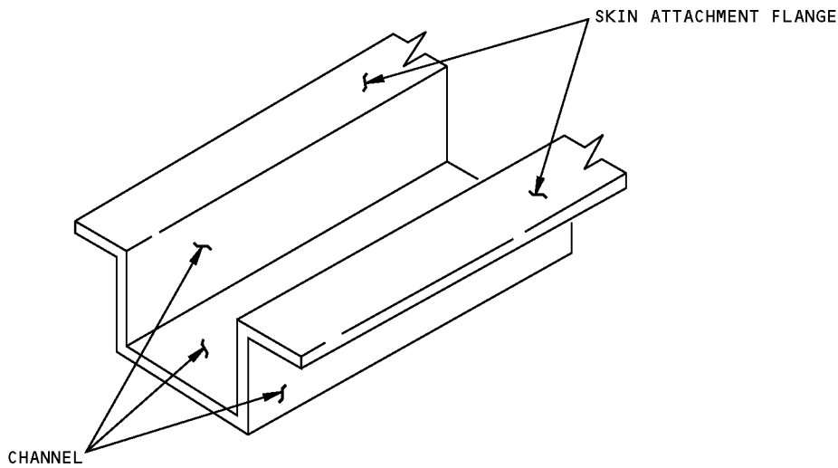
TYPICAL STRINGER SECTIONS
