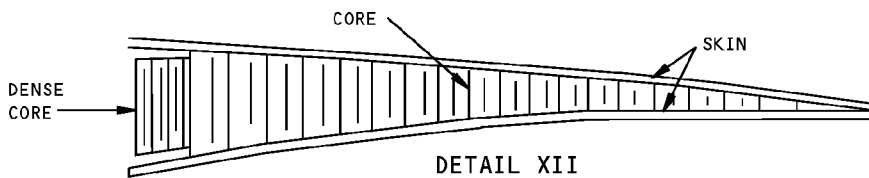
Leading Edge Slat Structure Identification Figure 1 (Sheet 8 of 11)
