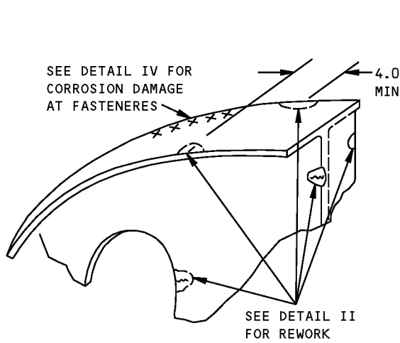
REMOVAL OF DAMAGE ON NOSE RIB AND END RIB DETAIL V
