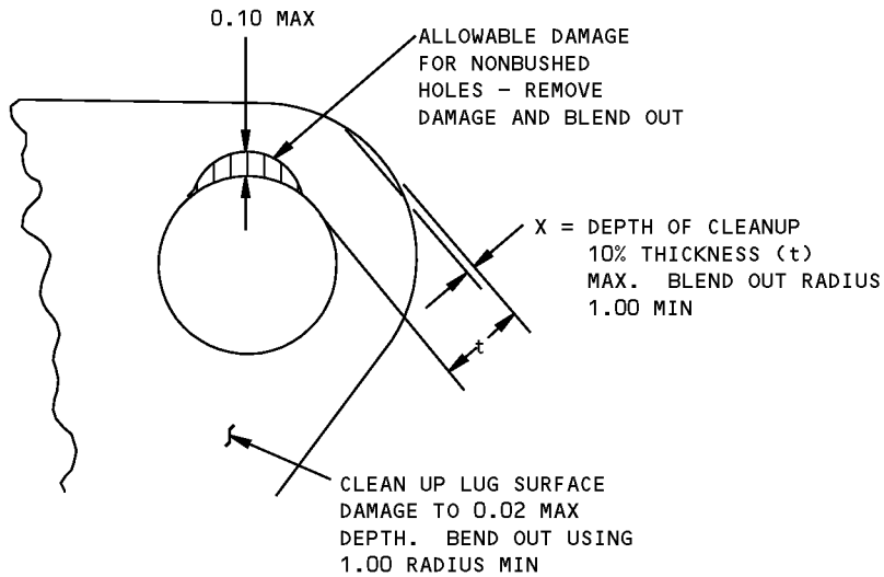
DAMAGE CLEANUP FOR SURFACES OF LUG DETAIL VII
