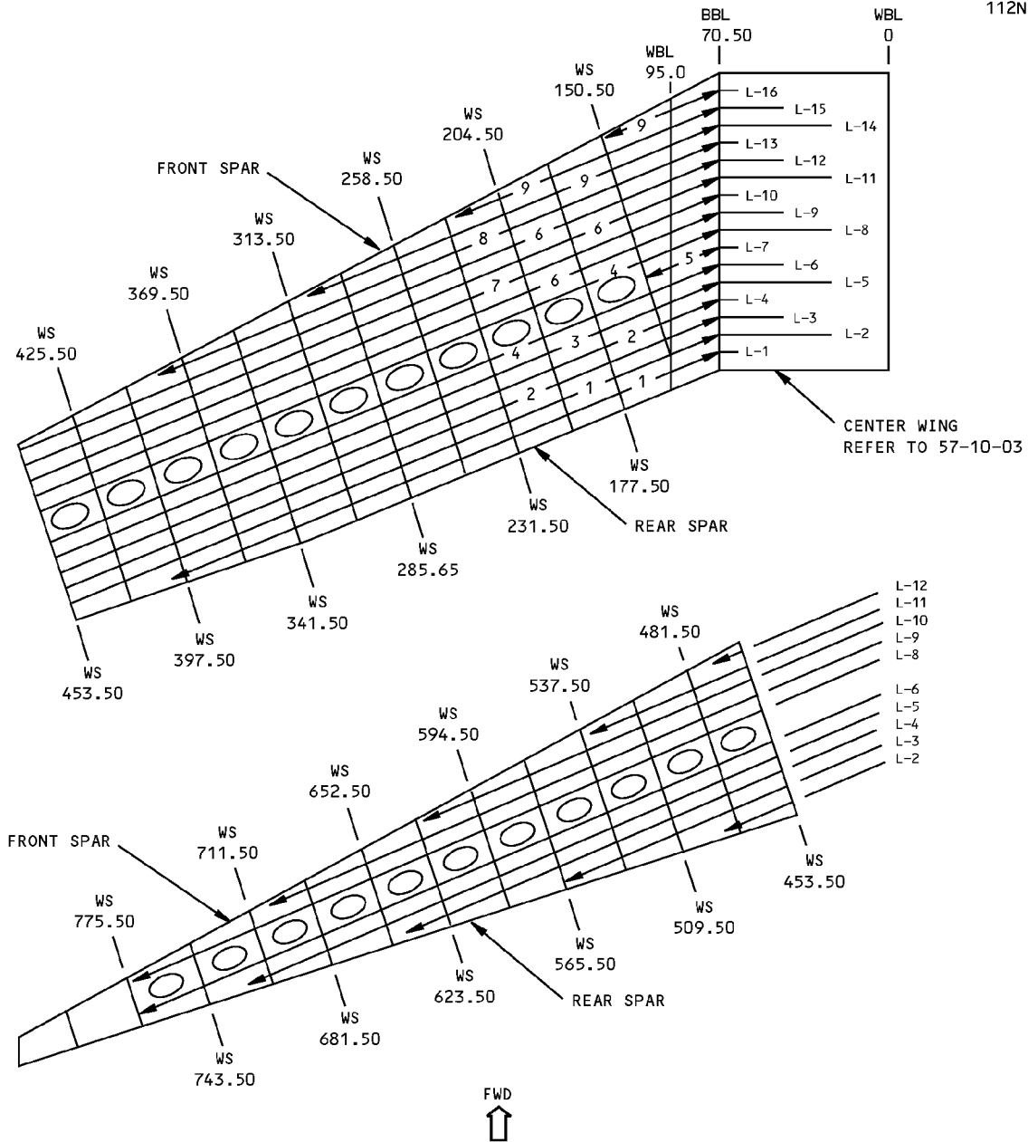
PLAN VIEW LOWER SURFACE LEFT WING SHOWN RIGHT WING OPPOSITE DETAIL I
