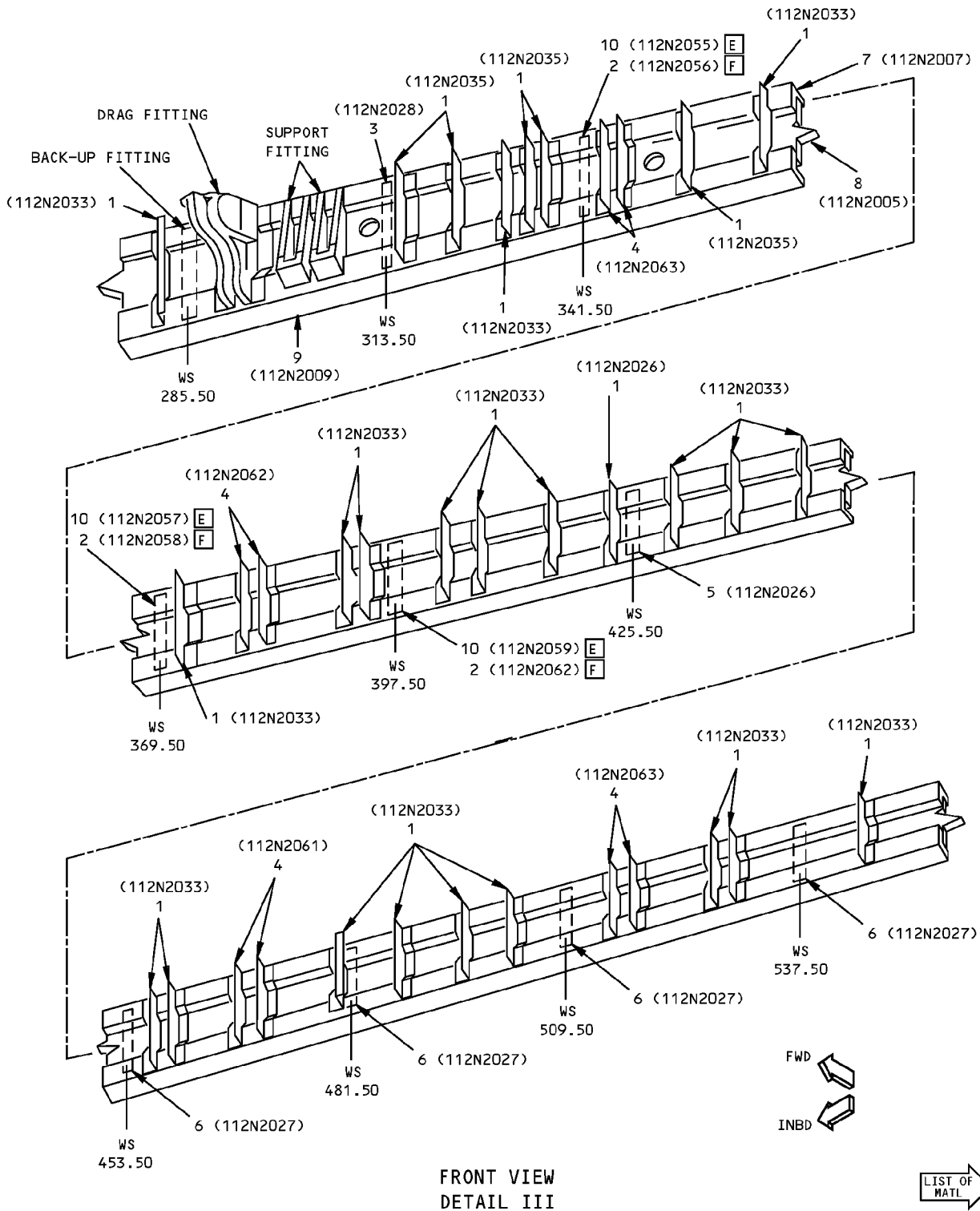
Outer Wing Front Spar Identification Figure 1 (Sheet 4 of 7)
