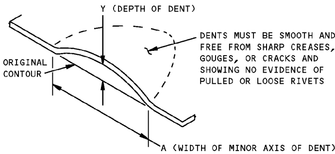
ALLOWABLE DAMAGE FOR DENT DETAIL V
