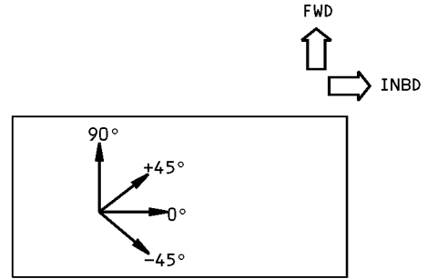
PLY ORIENTATION DIAGRAM SEE TABLE III FOR INDIVIDUAL PLY ORIENTATION AND MATERIALS
