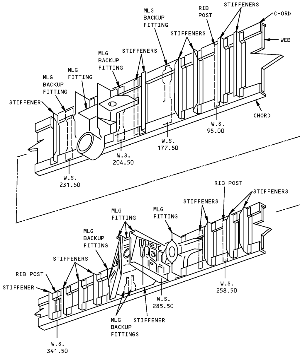
DETAIL I
