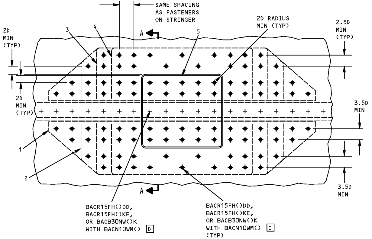
DETAIL I
