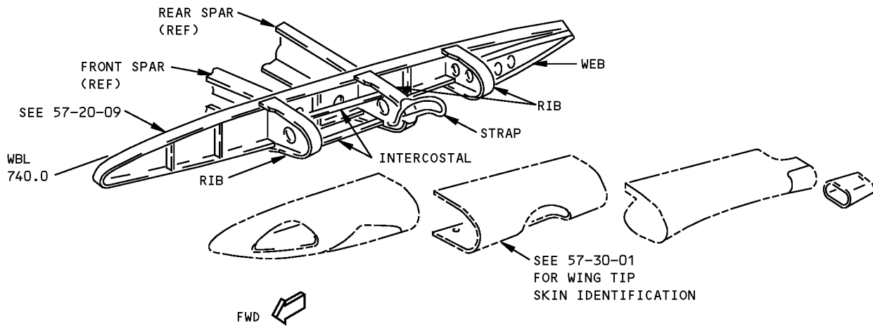
DETAIL I
