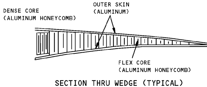
Leading Edge Slat - Trailing Edge Wedge Repairs Figure 201
