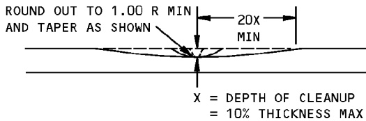
REMOVAL OF NICK, GOUGE AND SCRATCH DAMAGE ON A SURFACE DETAIL VI
