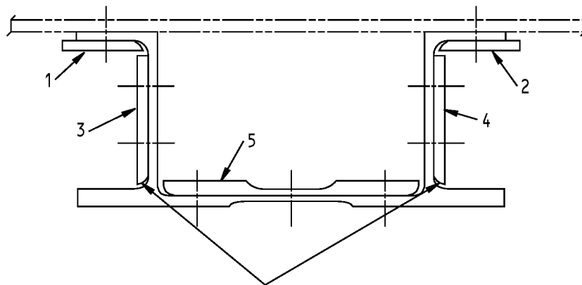
TRIM REPAIR PARTS 3 AND 4 TO FIT AROUND RIB ATTACHMENT TAB
