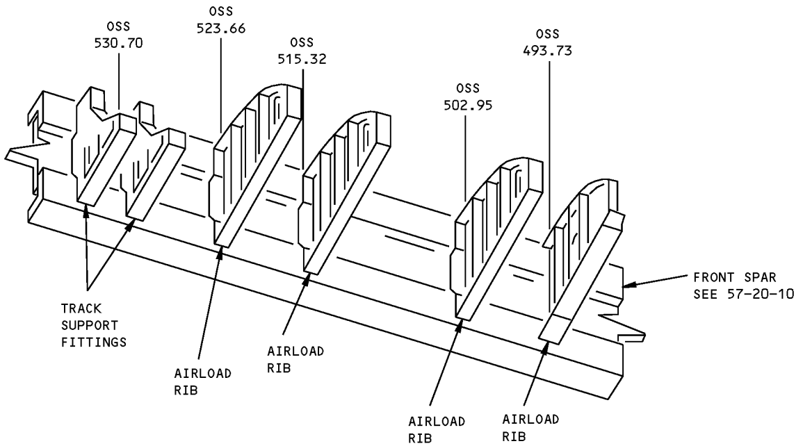
RIGHT WING ONLY DETAIL IV
