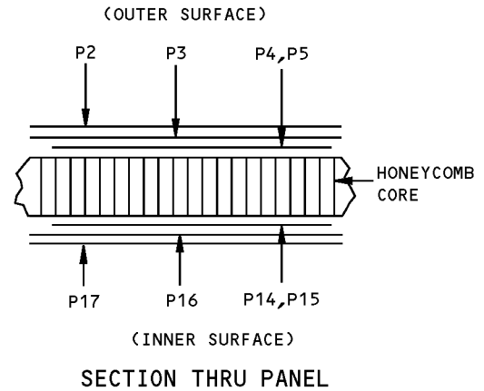
SECTION THRU PANEL
