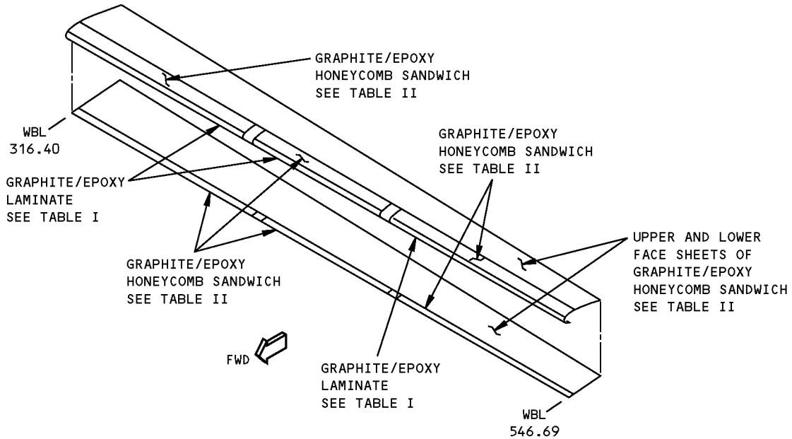
AFT FLAP - OUTBOARD TRAILING EDGE FLAP DETAIL IV
