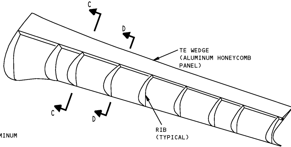
SLAT NO. 5
