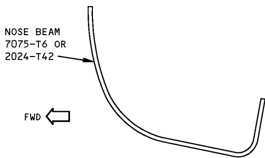
CROSS-SECTIONAL VIEW OF NOSE BEAM TYPICAL FOR ISS 106.0 THRU ISS 285.0 SECTION A-A
