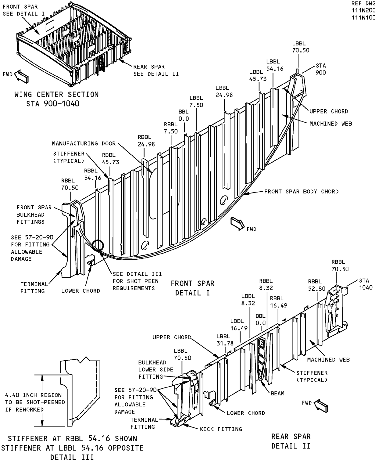
Wing Center Section Front and Rear Spars Allowable Damage Figure 101 (Sheet 1 of 4)
