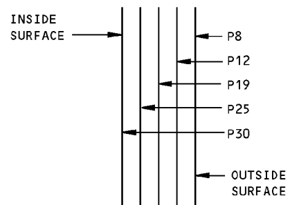
SECTION THRU SPOILER NO. 6
