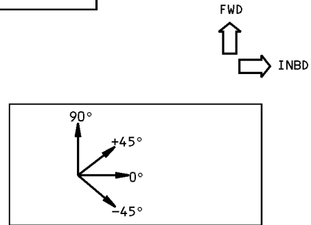
PLY ORIENTATION DIAGRAM SEE TABLE IV FOR INDIVIDUAL PLY ORIENTATION AND MATERIALS
