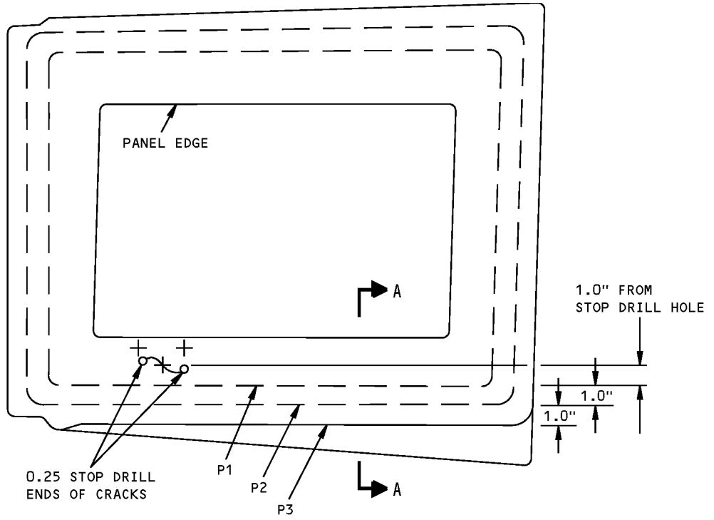
DETAIL I
