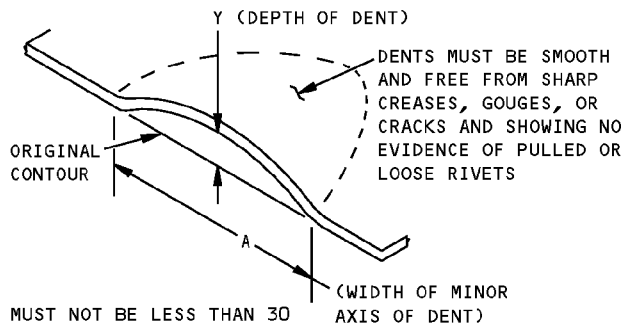
ALLOWABLE DAMAGE FOR DENT DETAIL VII
