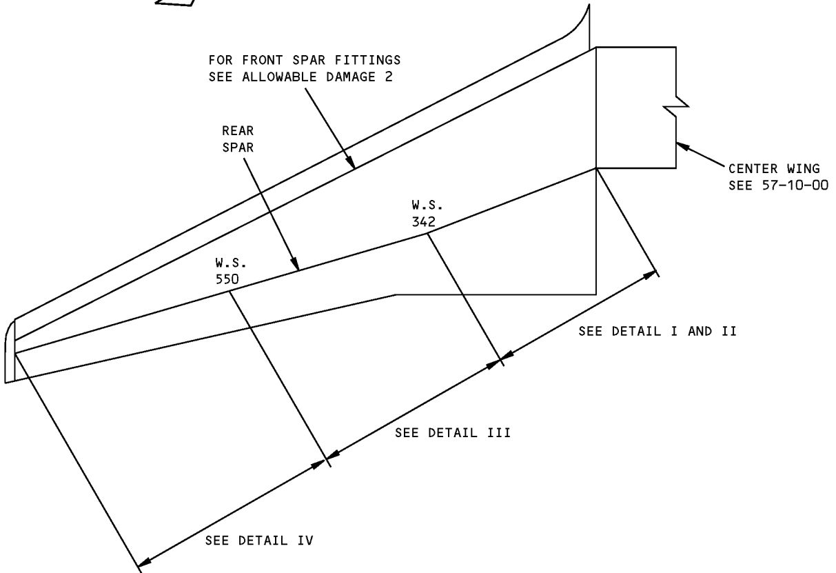
Outer Wing Rear Spar Fittings Allowable Damage Figure 101 (Sheet 1 of 8)
