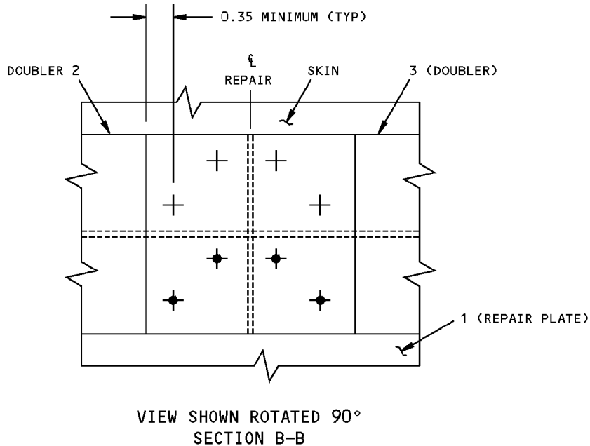
Leading Edge Slats - Nose Skin Repairs Figure 201 (Sheet 3 of 3)
