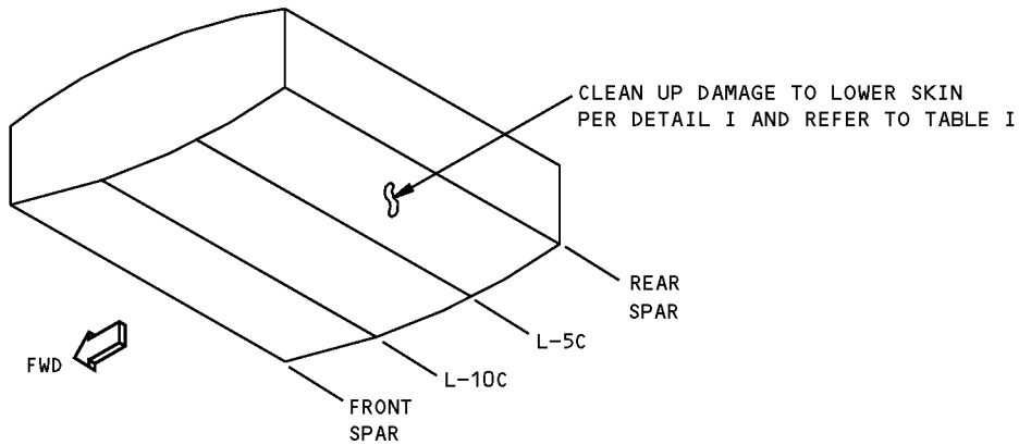
Center Wing Skin Allowable Damage Figure 101 (Sheet 1 of 3)
