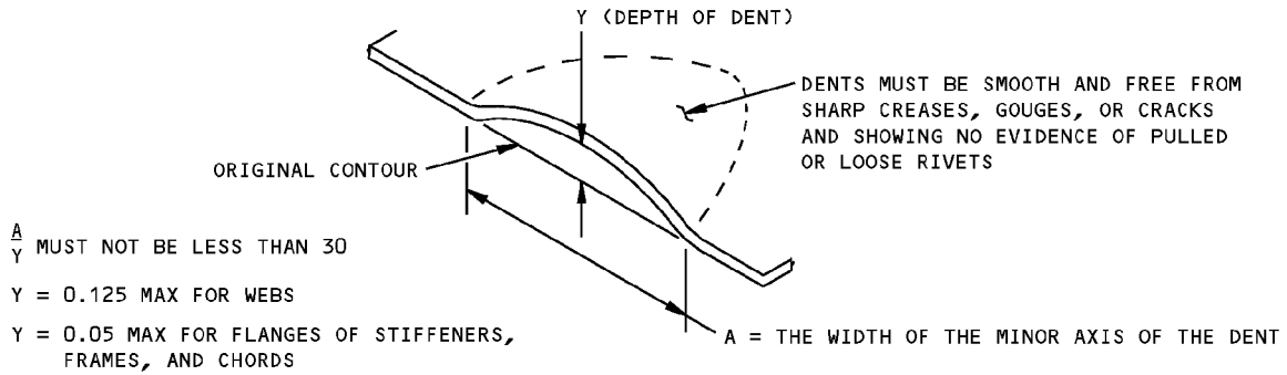
ALLOWABLE DAMAGE FOR DENT DETAIL III
