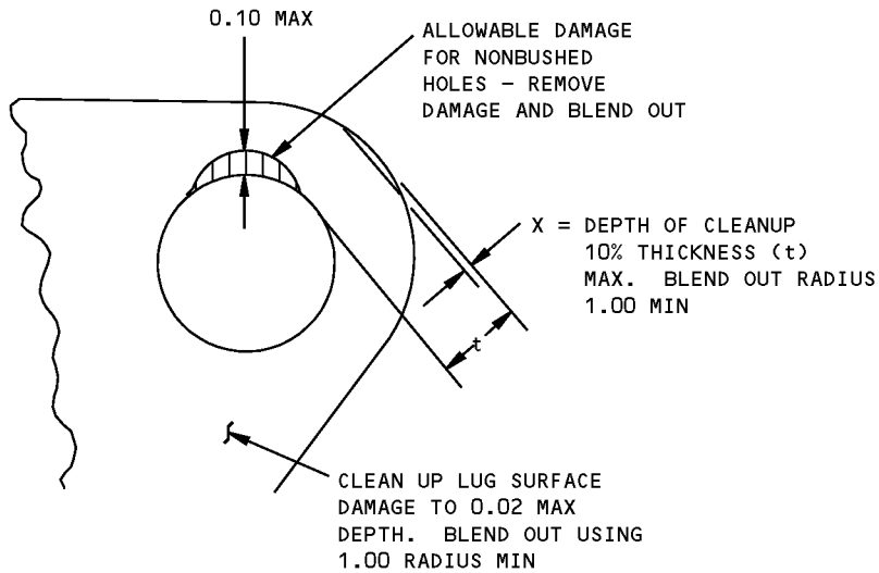
DAMAGE CLEANUP FOR SURFACES OF LUG DETAIL VI
