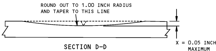
Wing Skin Lower Surface Corrosion Repair at Fuel Tank Access Door Cutouts Figure 201 (Sheet 3 of 6)
