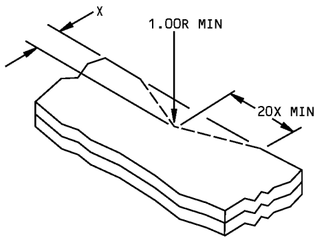
DETAIL II
