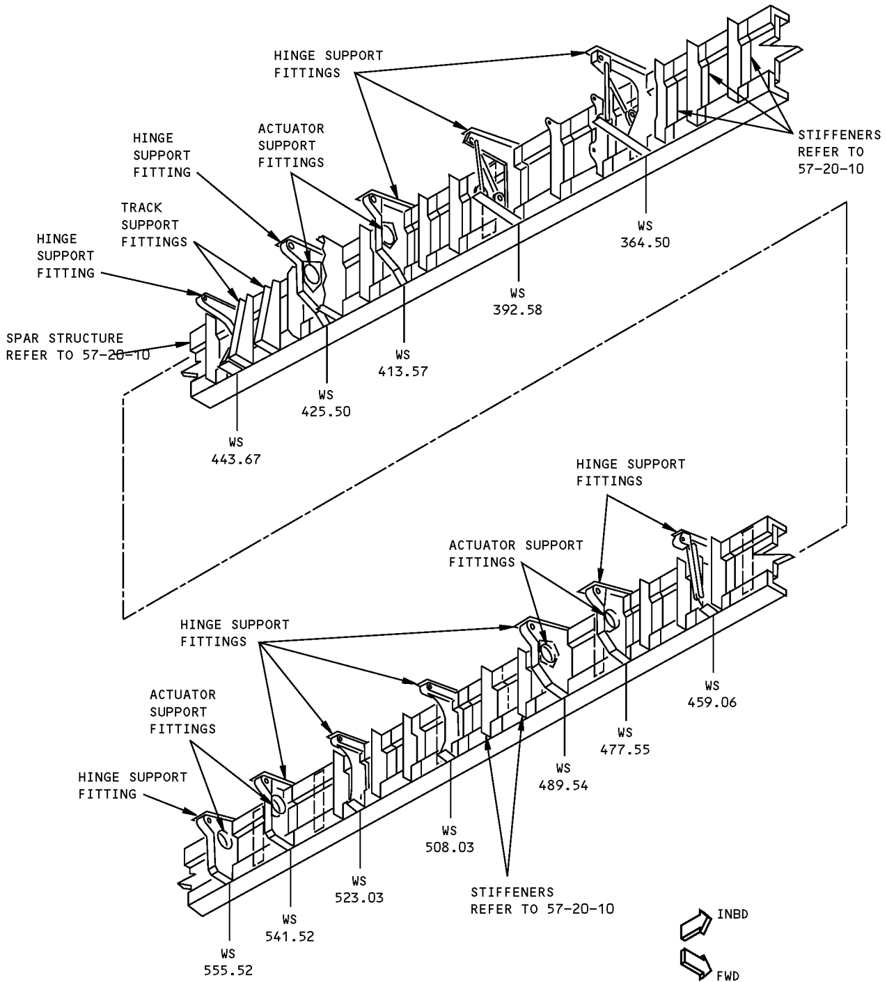
REAR SPAR - REAR VIEW DETAIL III
