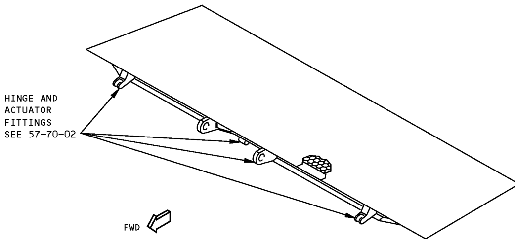
TYPICAL SPOILER DETAIL I
