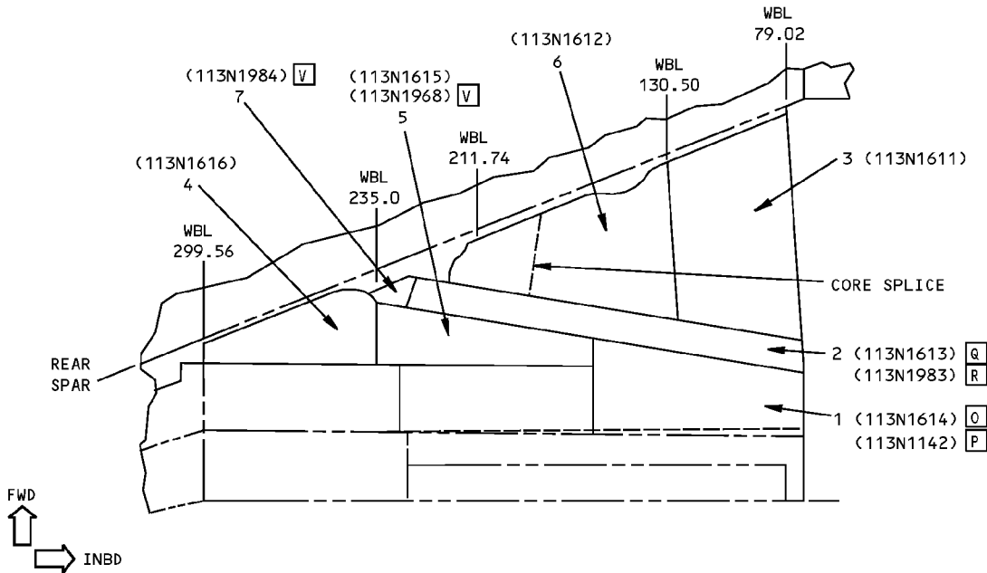
DETAIL I
