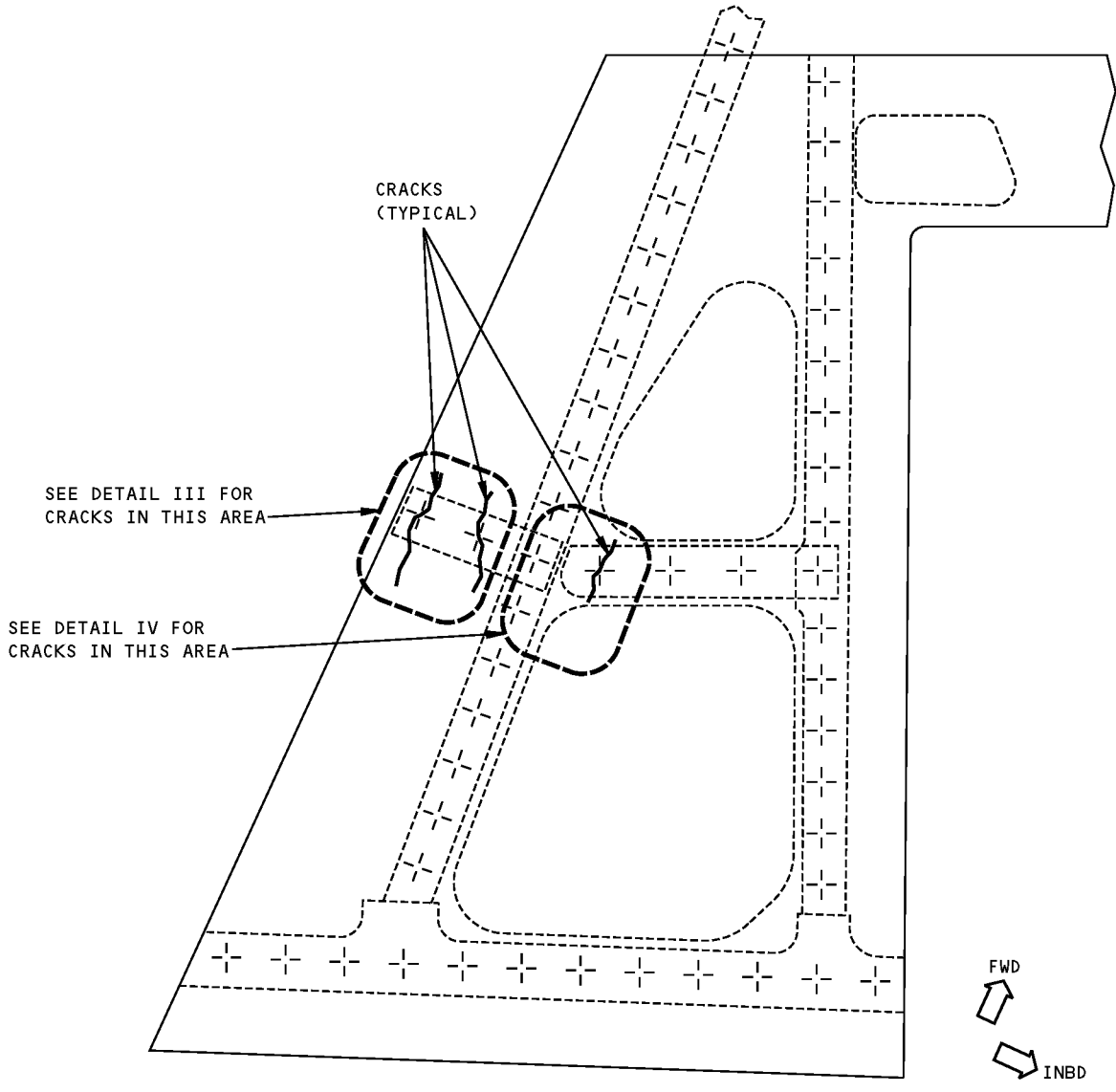
DETAIL II
