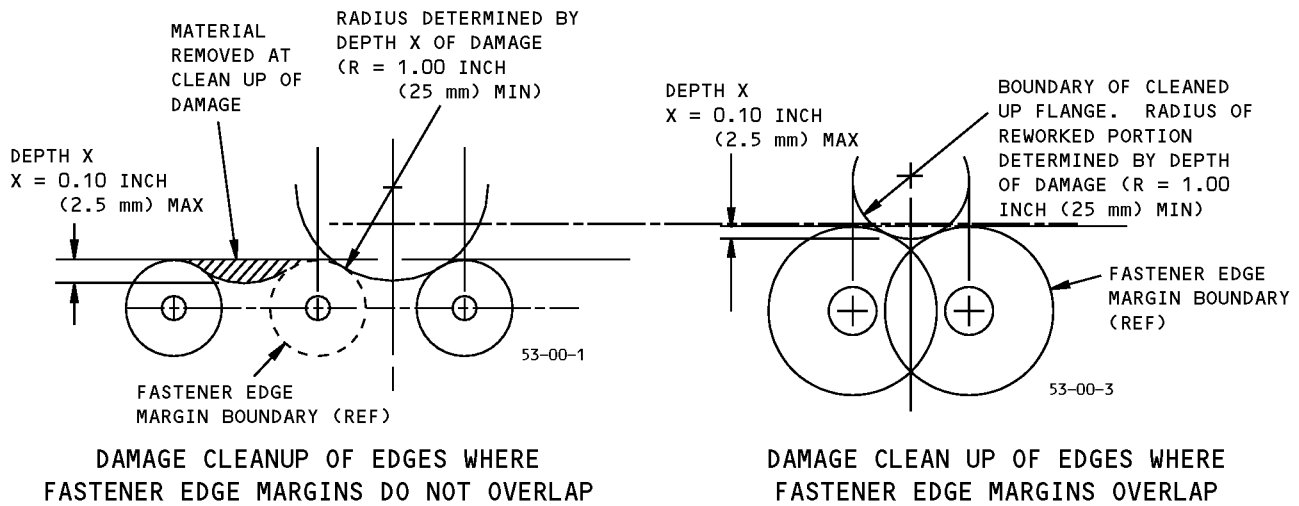
DETAIL V
