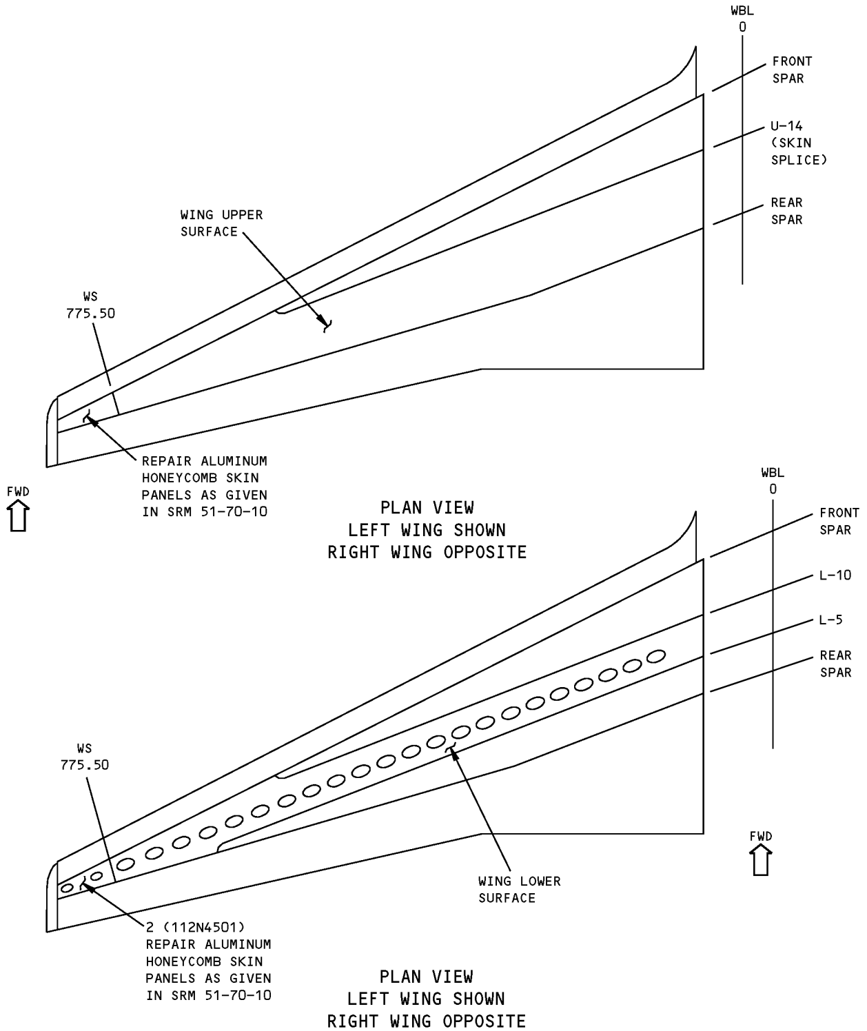
Outer Wing Skin Panel Repair Figure 201 (Sheet 2 of 2)
