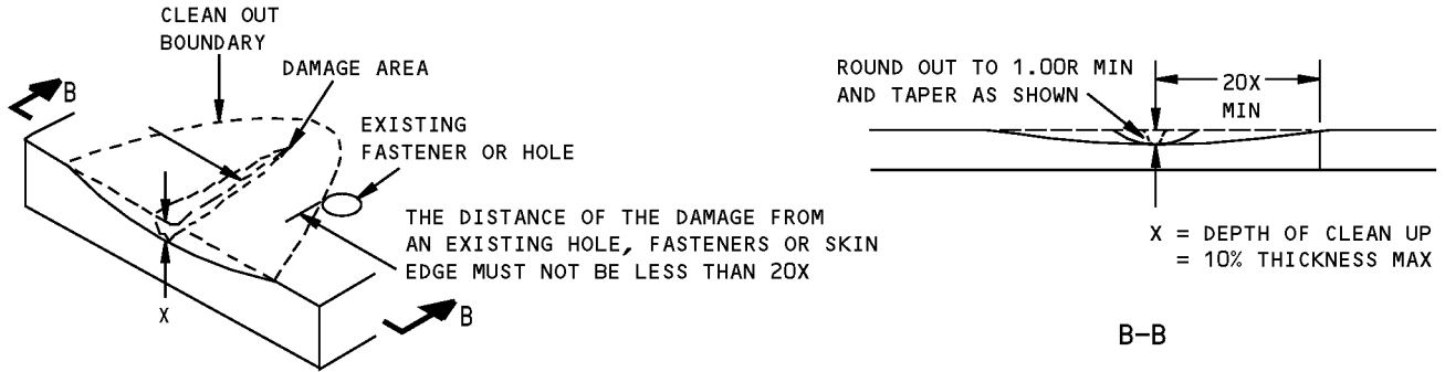
REMOVAL OF NICK, GOUGE AND SCRATCH DAMAGE ON A SURFACE DETAIL V
