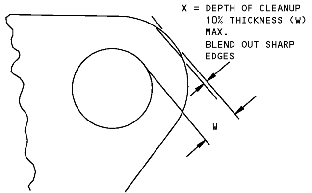
DAMAGE CLEANUP FOR EDGES OF LUG DETAIL VI
