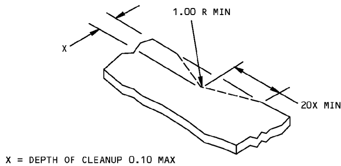
DETAIL V
