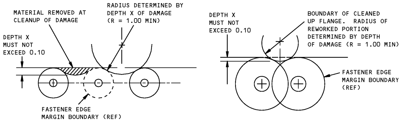
DETAIL I
