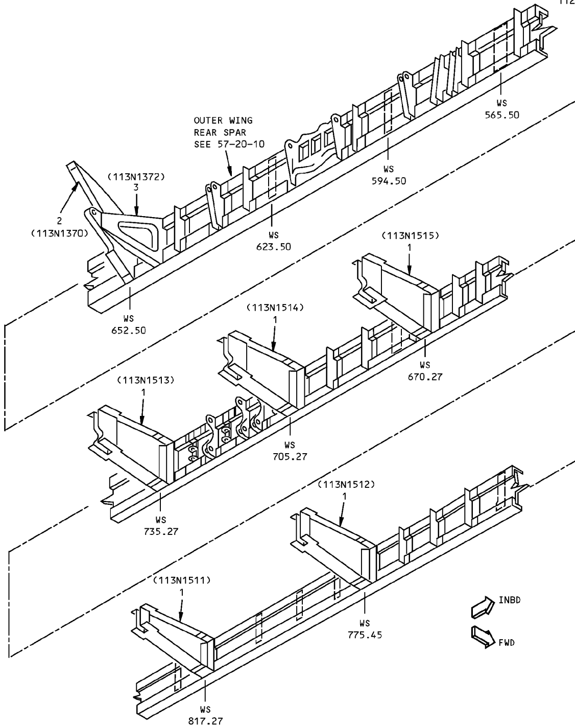
DETAIL I
