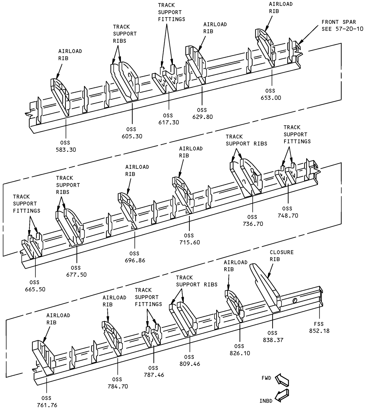
DETAIL III
