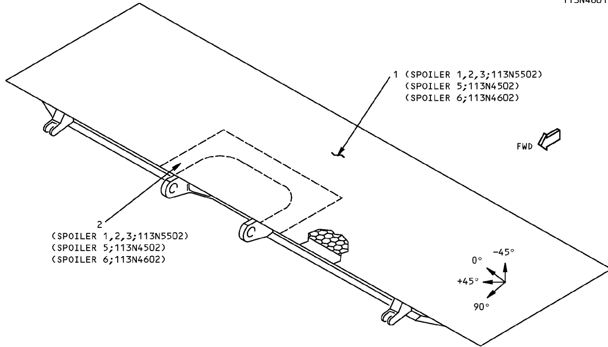
SPOILERS NO. 1,2,3 SHOWN SPOILERS NO. 5,6 SIMILAR DETAIL VII E
