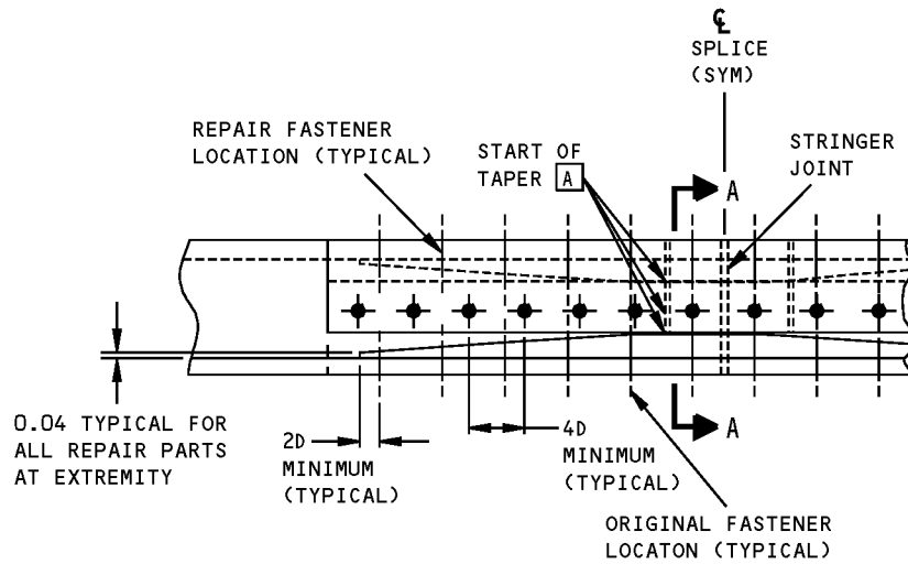
DETAIL III
