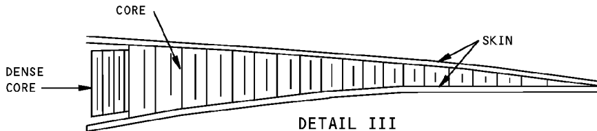
Leading Edge Slat Structure Identification Figure 1 (Sheet 2 of 11)
