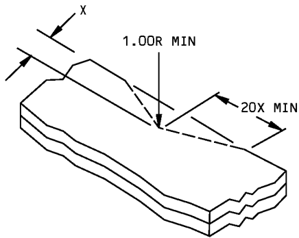
DETAIL II
