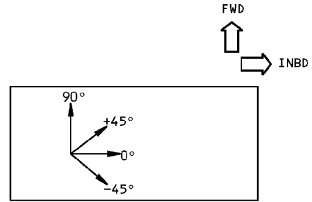
PLY ORIENTATION DIAGRAM SEE TABLE VII FOR INDIVIDUAL PLY ORIENTATION AND MATERIALS
