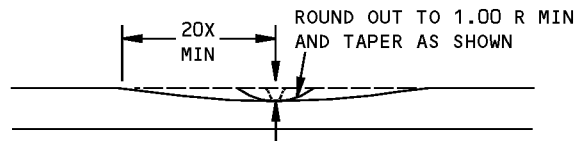
SECTION C-C
