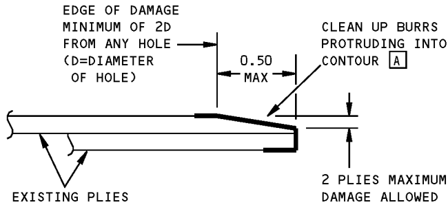
DAMAGE CLEANUP AND SEALING OF EDGE EROSION DETAIL V
