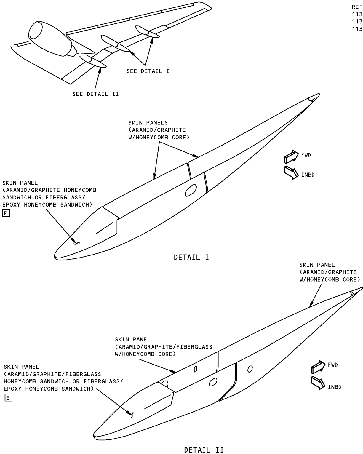
Flap Track Fairing Skin Allowable Damage Figure 101 (Sheet 1 of 4)
