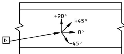
VIEW ON SPAR LOOKING AFT
