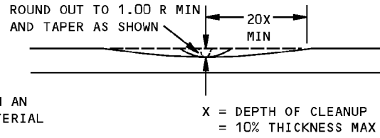
SECTION E-E
