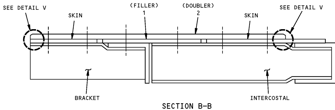
Time Limited Repair - Main Flap - Out Board Trailing Edge - Out Board End Skin Panel Figure 201 (Sheet 5 of 6)
