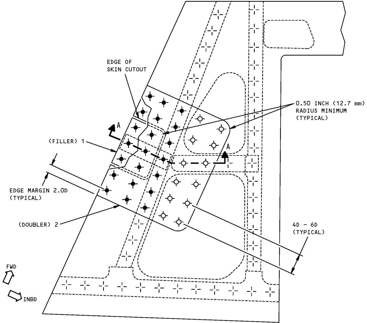
DETAIL III
