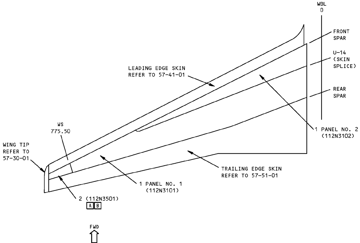
PLAN VIEW LEFT WING SHOWN RIGHT WING OPPOSITE
