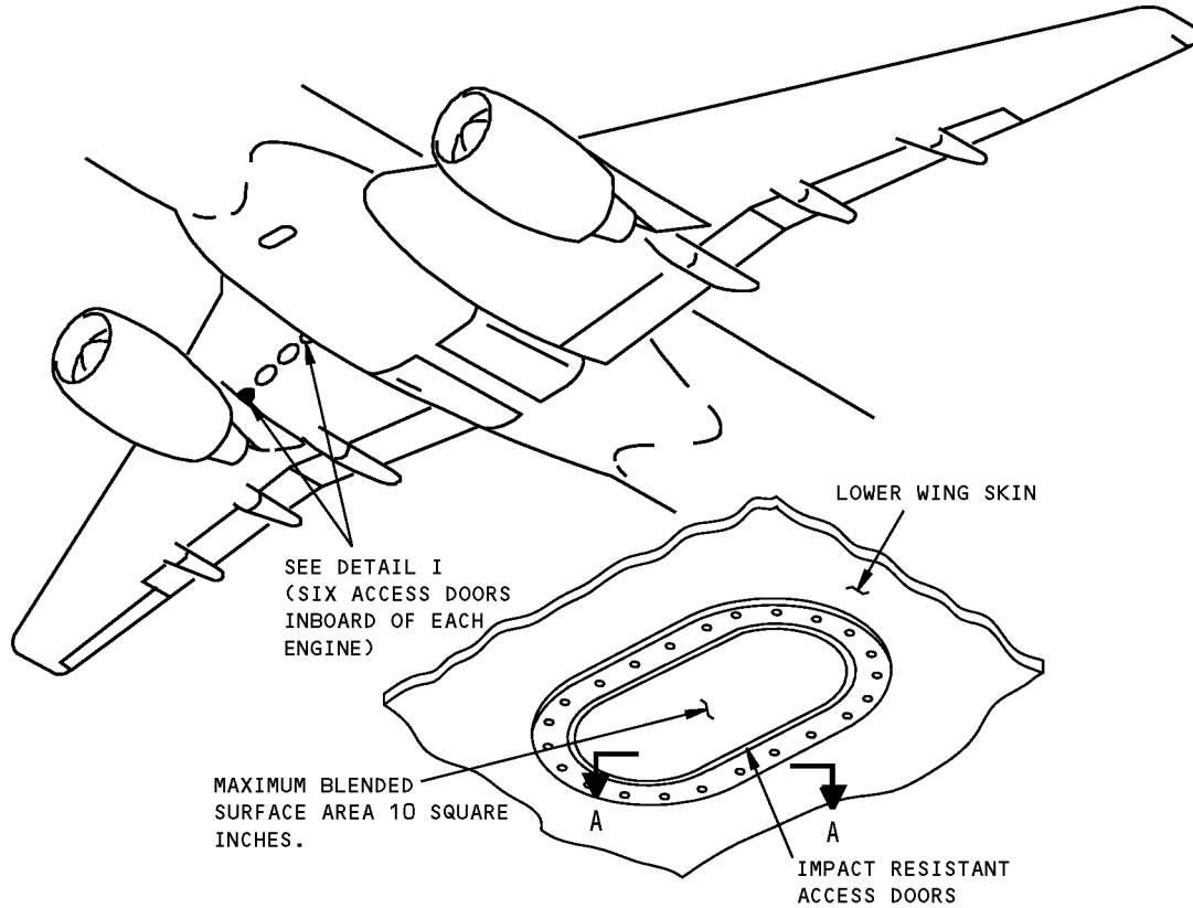
DETAIL I
