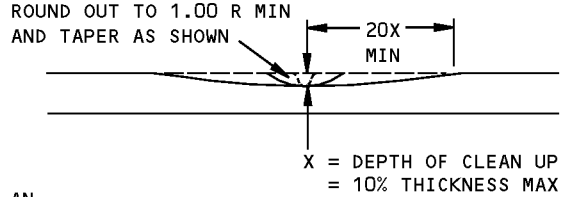
SECTION C-C
