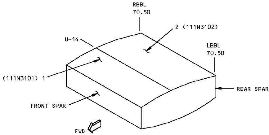
UPPER SKIN PANELS DETAIL I
