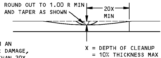
REMOVAL OF NICK, GOUGE AND SCRATCH DAMAGE ON A SURFACE DETAIL V
