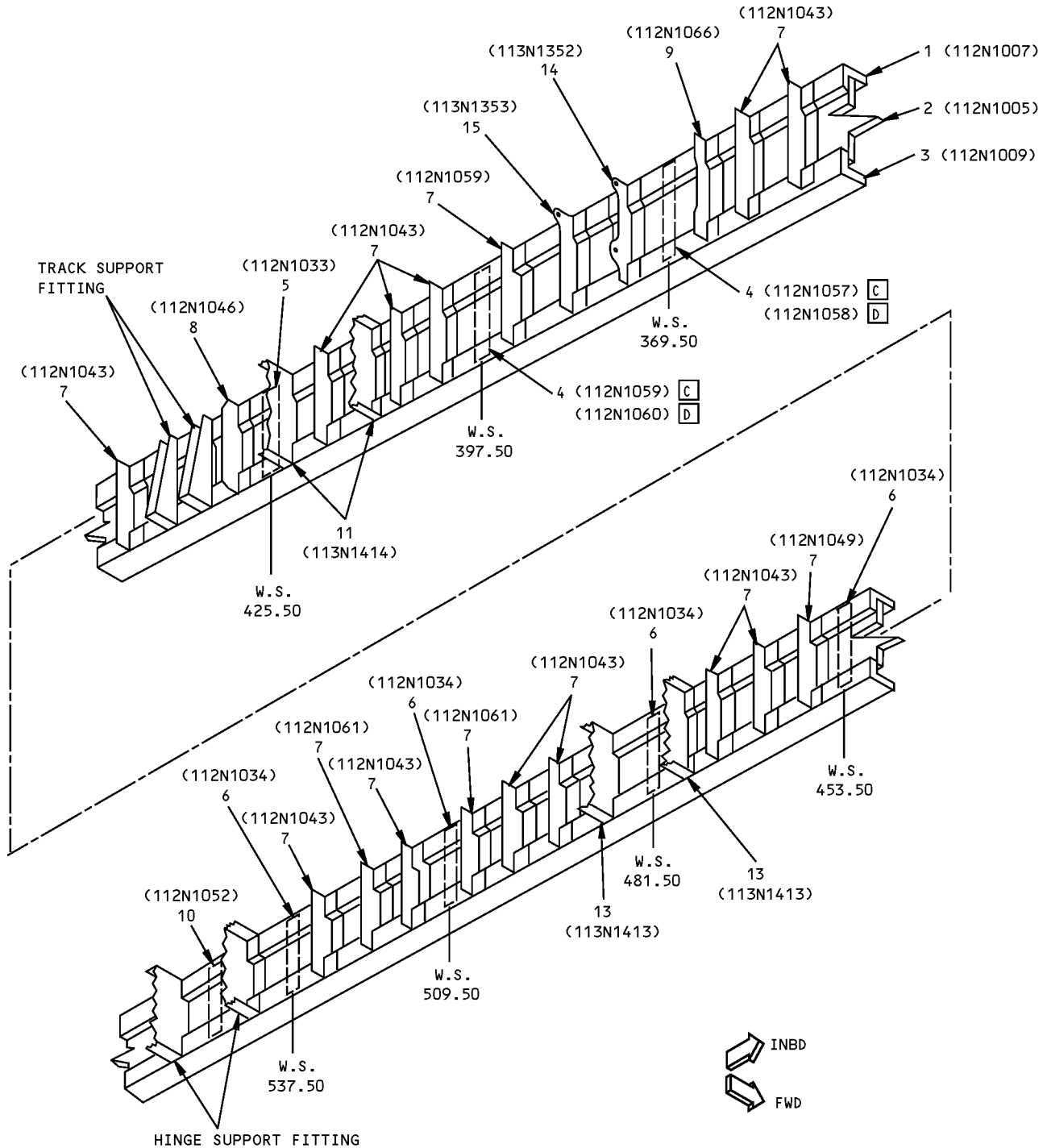
DETAIL II
