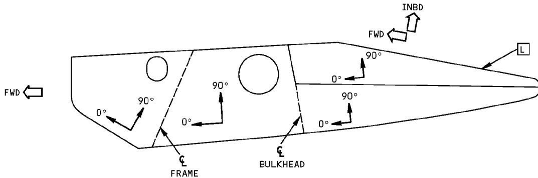
SIDE VIEW VIEW ON PANEL C
