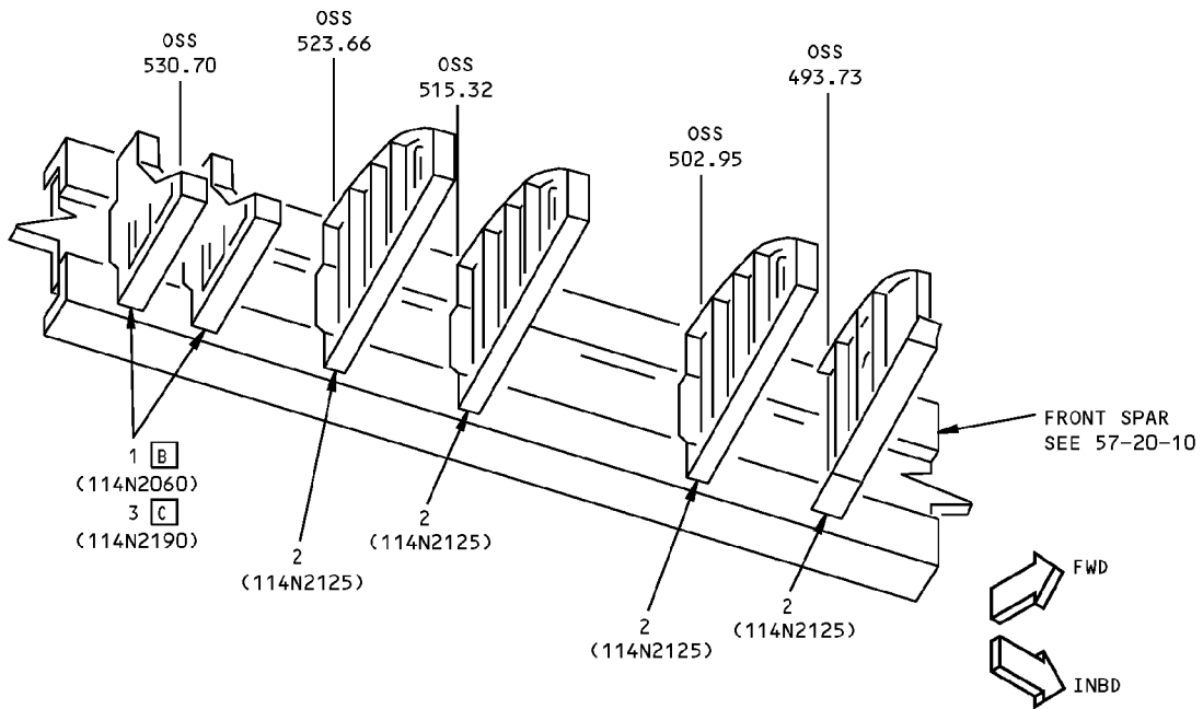
DETAIL IV
