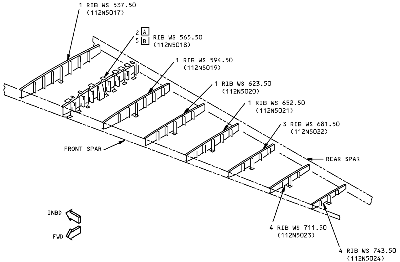
DETAIL V
