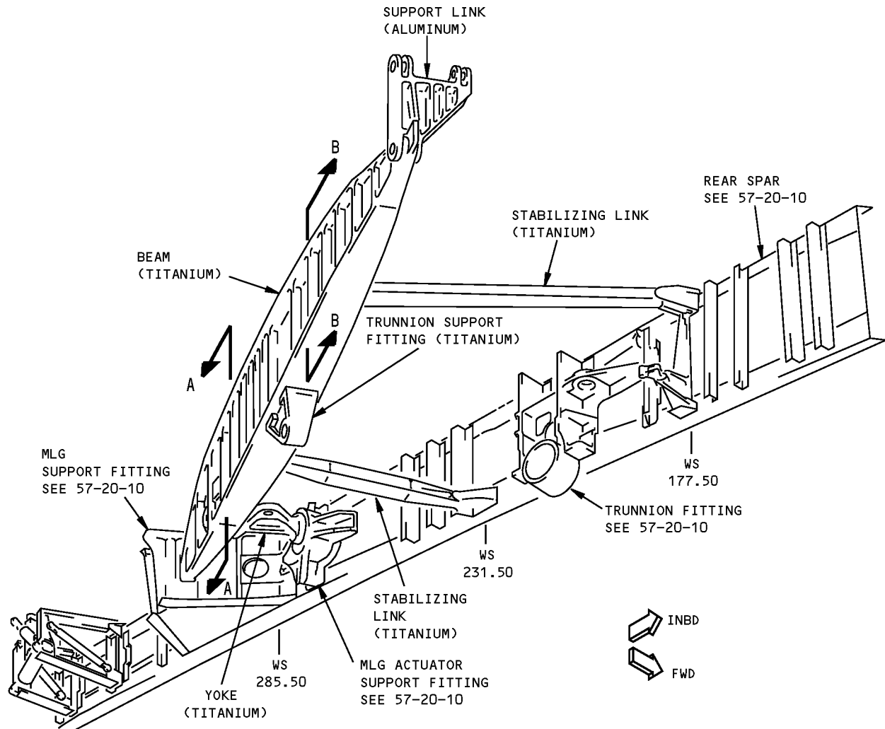
DETAIL I
