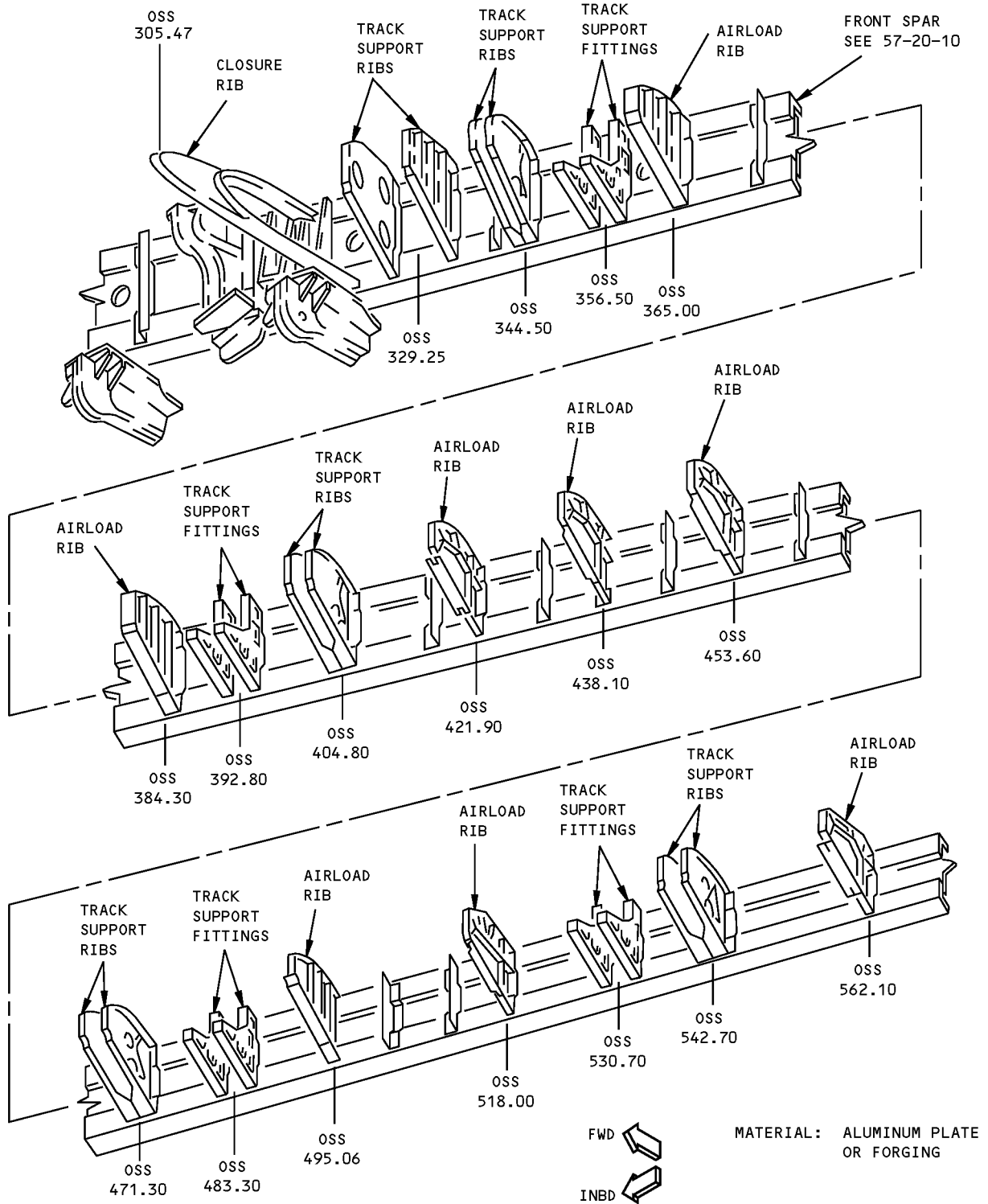
DETAIL II
