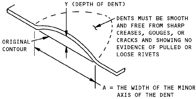
ALLOWABLE DAMAGE FOR DENT DETAIL XI
