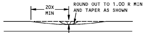
SECTION C-C REMOVAL OF NICK OR CRACK DAMAGE ON AN EDGE DETAIL IX
