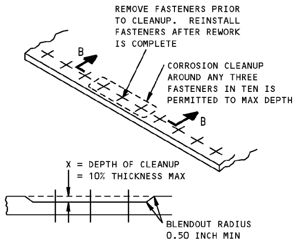
SECTION B-B CORROSION CLEANUP DETAIL V
