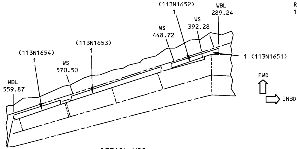
DETAIL VII
