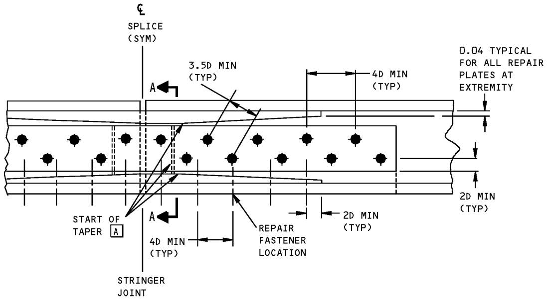
DETAIL III
