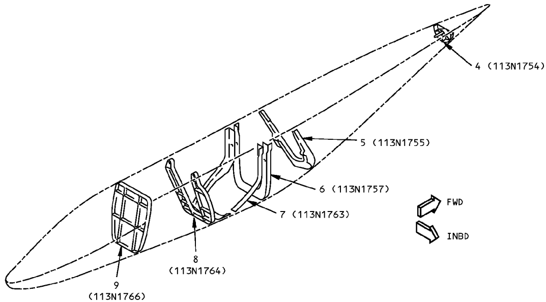
DETAIL II
