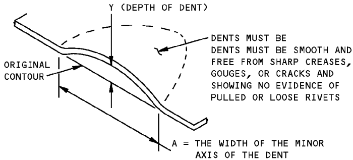
ALLOWABLE DAMAGE FOR DENT DETAIL III
