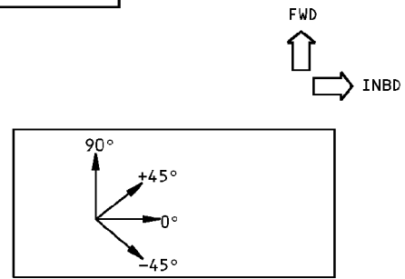
PLY ORIENTATION DIAGRAM SEE TABLE VIII FOR INDIVIDUAL PLY ORIENTATION AND MATERIALS
