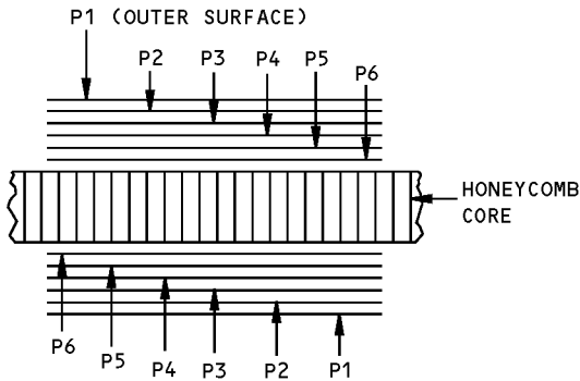
SECTION THRU THE WEDGE HONEYCOMB PANEL
