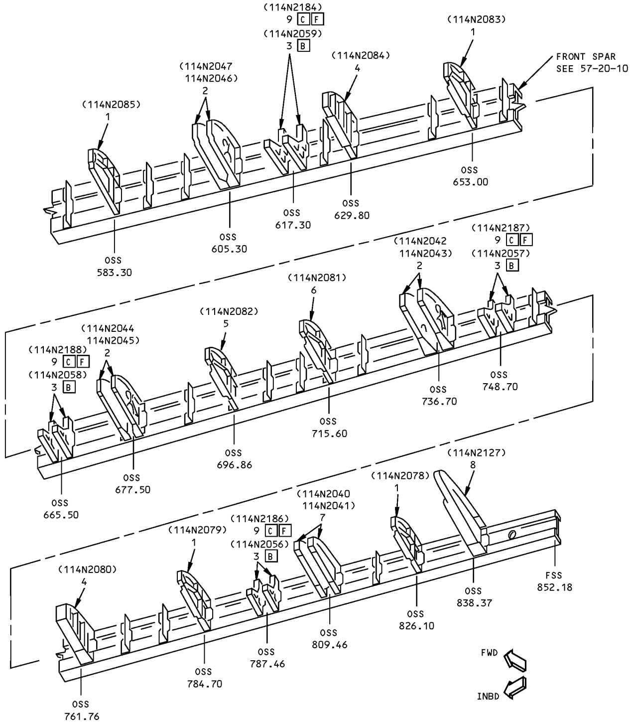
DETAIL III
