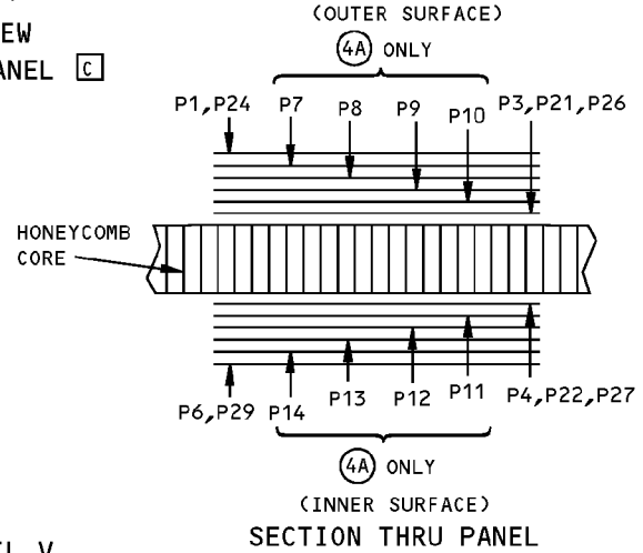
Flap Track Fairing Skin Identification Figure 1 (Sheet 5 of 7)
