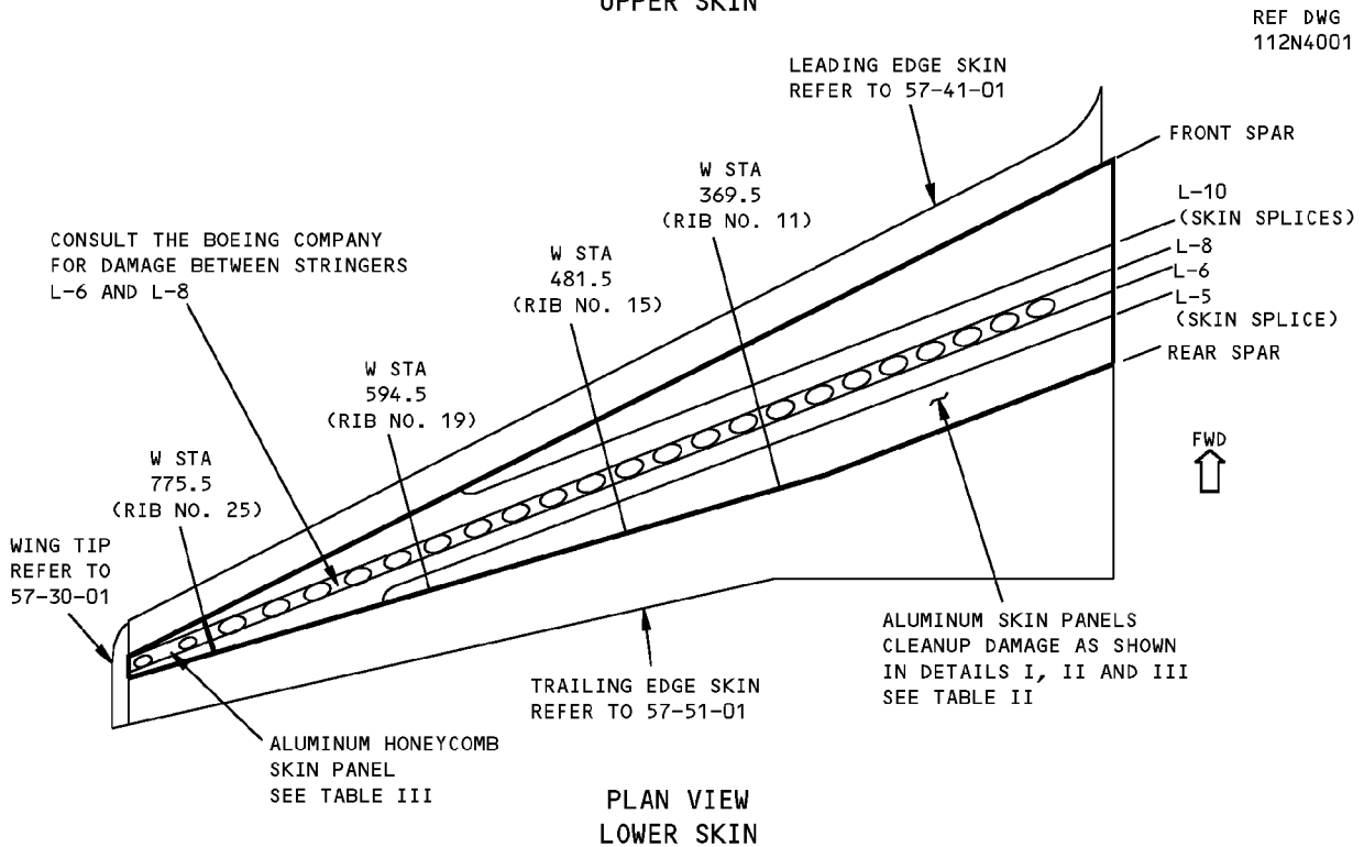
Outer Wing Skin Allowable Damage Figure 101 (Sheet 2 of 8)
