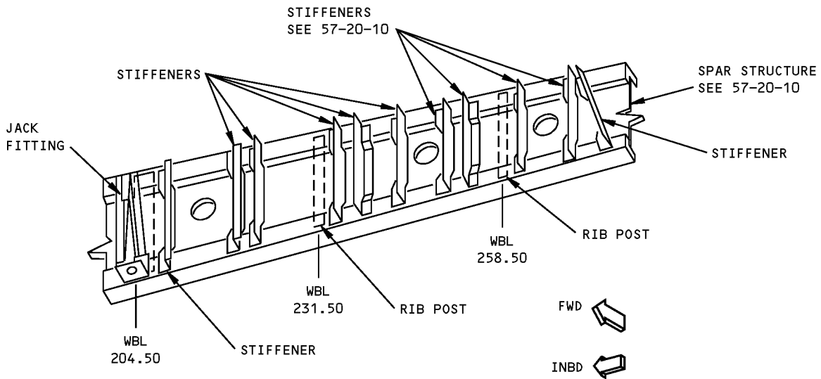
DETAIL I
