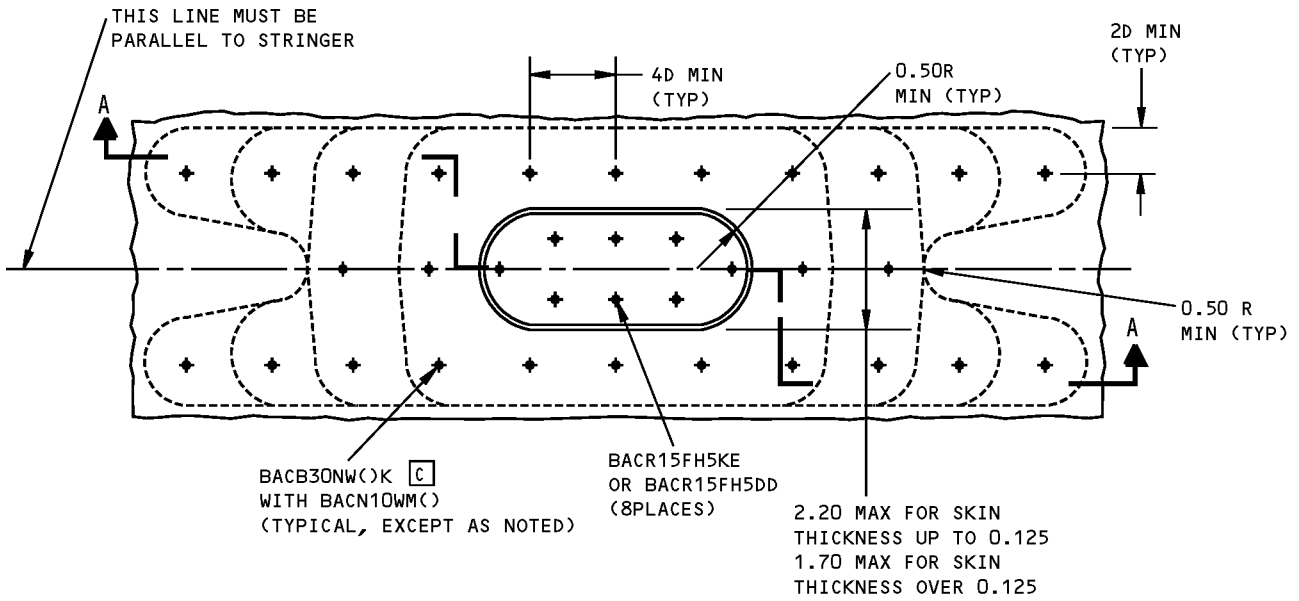
DETAIL I
