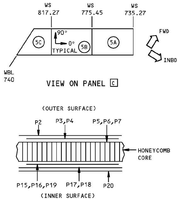
DETAIL XIII
