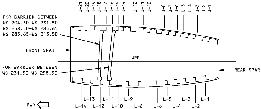
SECTION THRU WING AT WS 231.50 WS 204.50, WS 258.50, WS 285.65 AND WS 313.50 SIMILAR SECTION A-A
