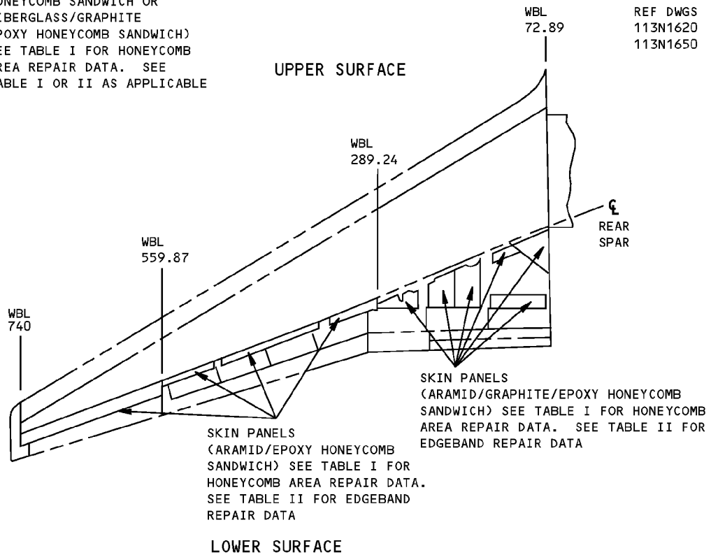
Wing Fixed Trailing Edge Skin Repairs Figure 201 (Sheet 1 of 6)
