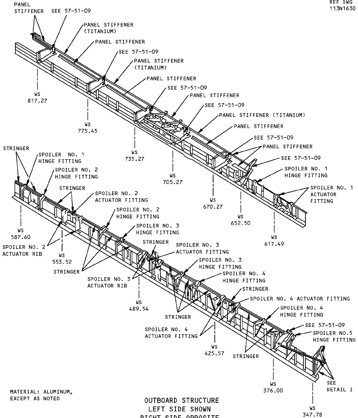
Wing Trailing Edge Structure Allowable Damage Figure 101 (Sheet 3 of 7)
