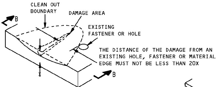
CORROSION CLEANUP DETAIL V
