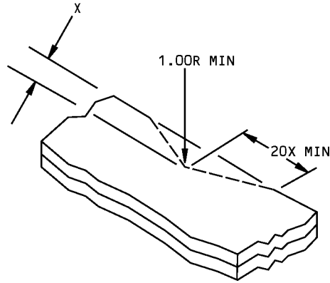
DETAIL I
