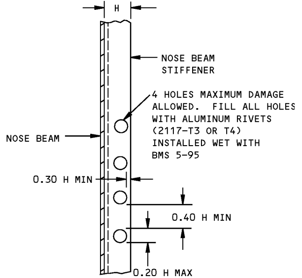
ALLOWABLE DAMAGE LIMITS FOR HOLES IN NOSE BEAM STIFFENERS DETAIL VIII
