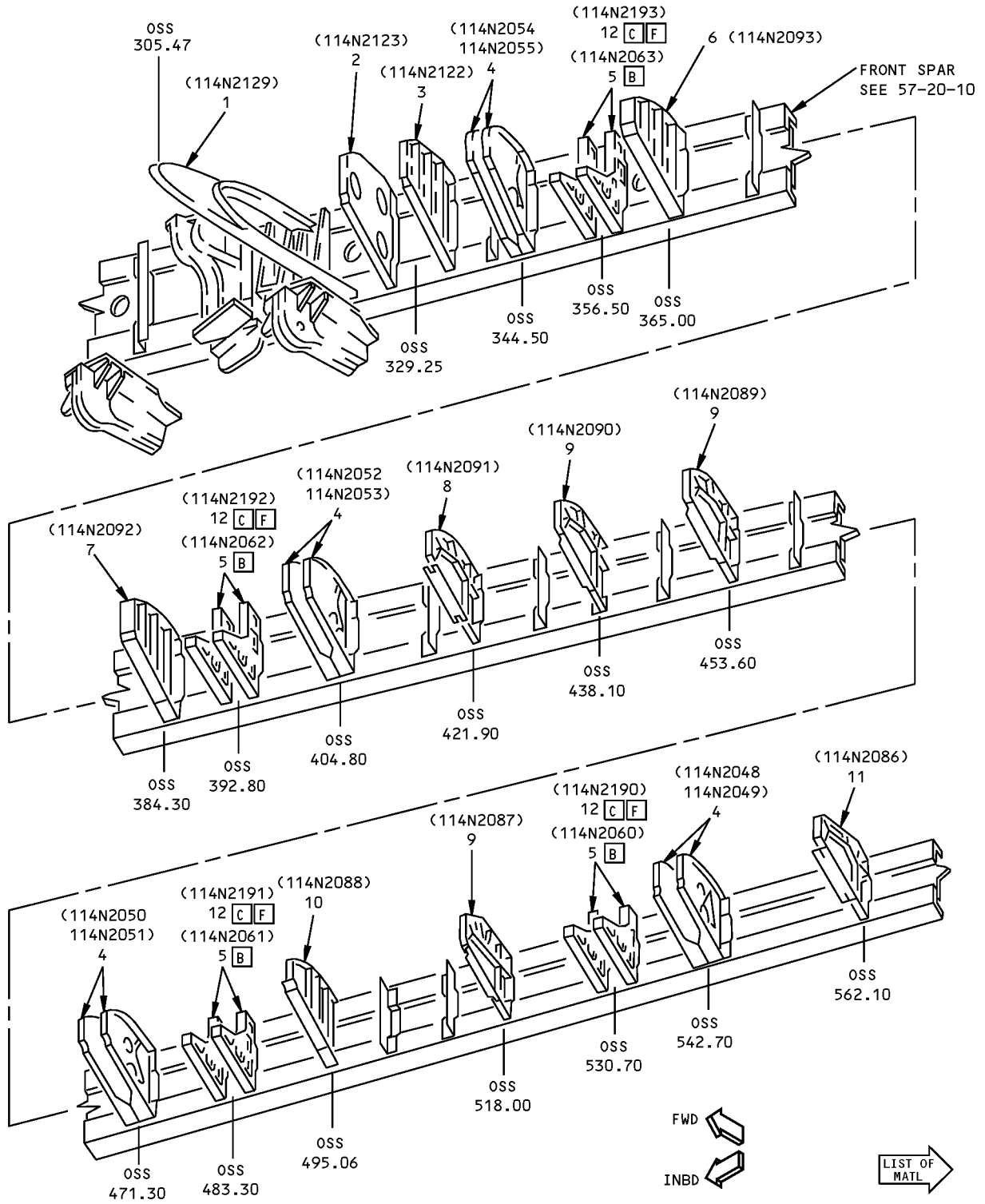
DETAIL II
