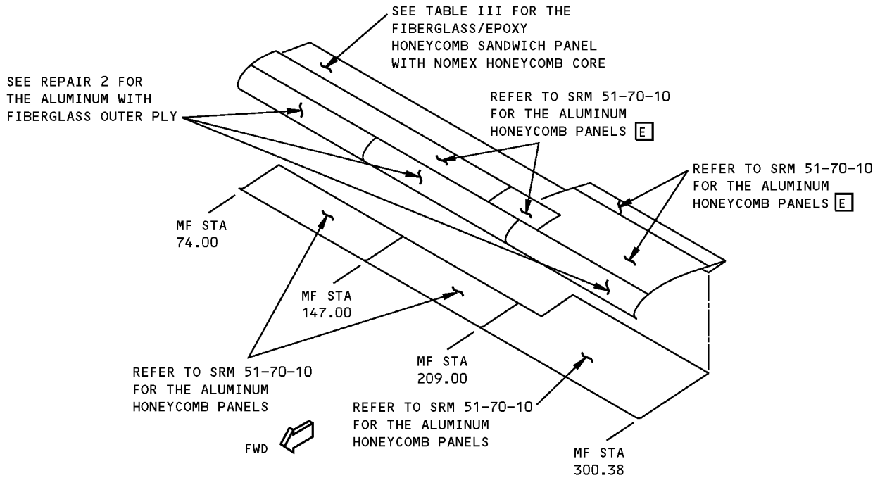
MAIN FLAP - INBD TRAILING EDGE FLAP DETAIL I
