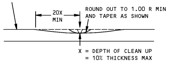
SECTION B-B DETAIL VIII
