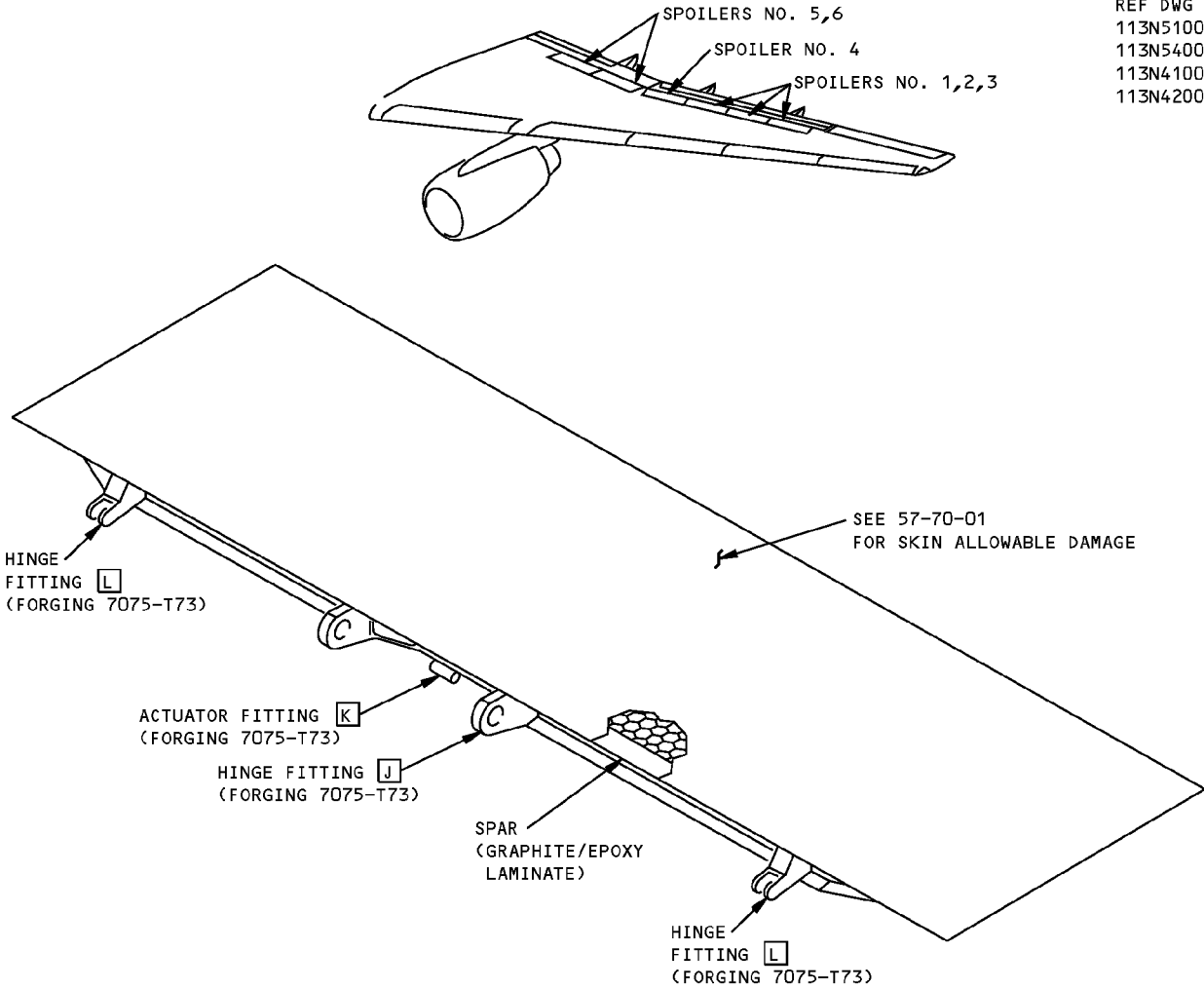
SPOILER NO. 1 SHOWN SPOILERS 2 THRU 6 SIMILAR DETAIL I
