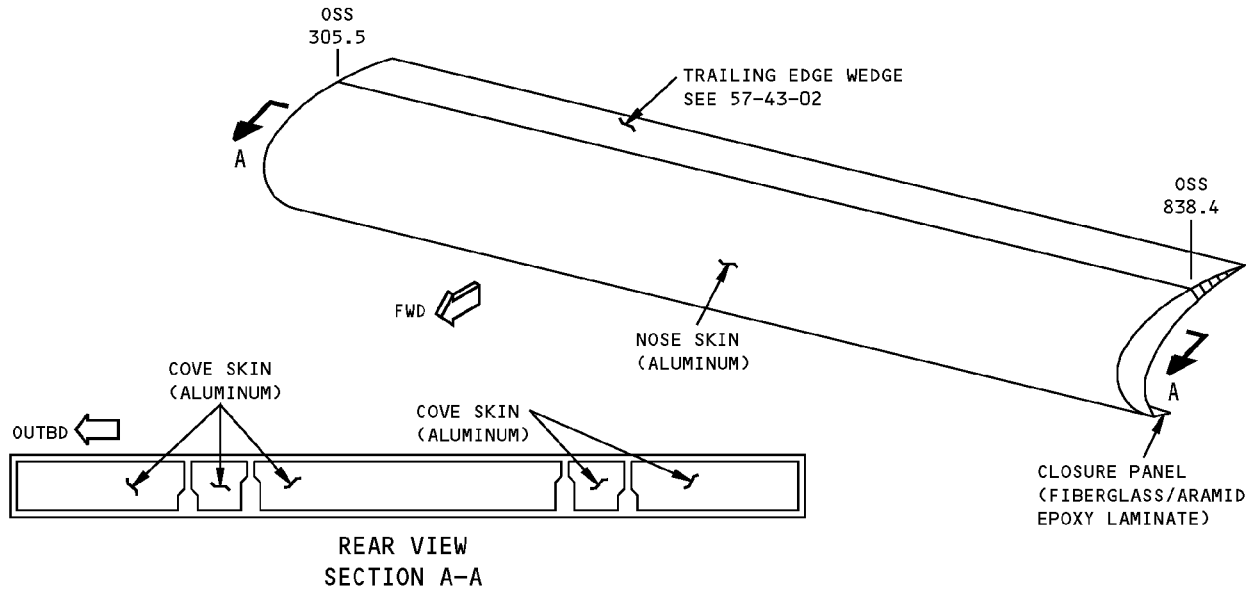
SLATS NO. 1 THRU NO. 4 DETAIL I
