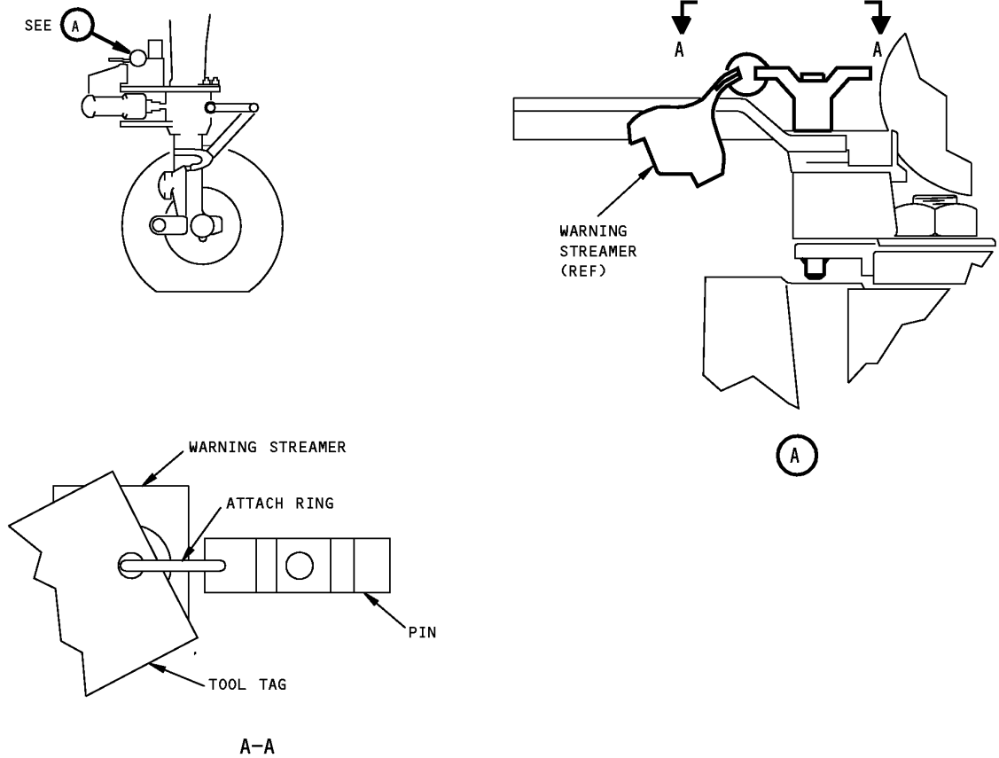
Nose Gear Towing Lever Lockpin Figure 1
