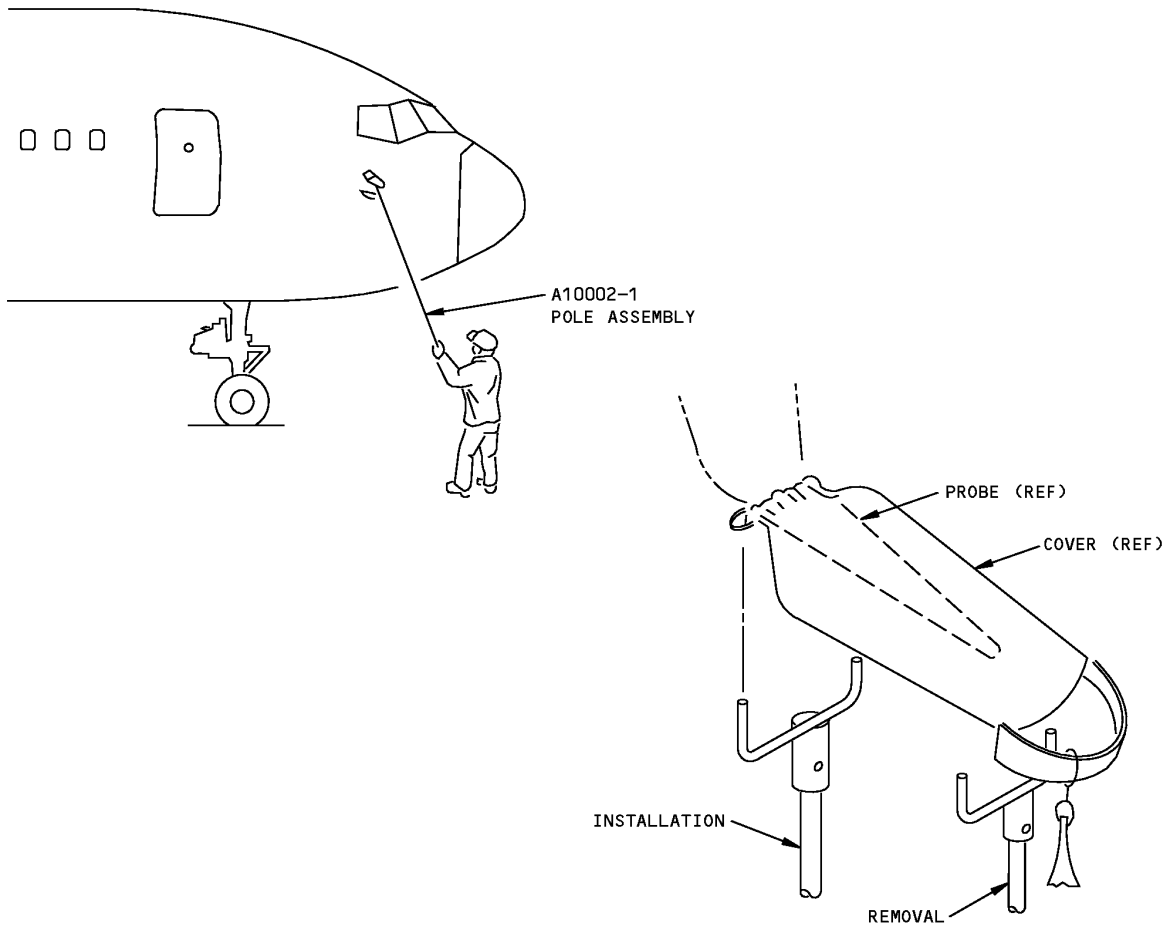
Pitot Probe Cover Removal/Installation Pole Figure 1
