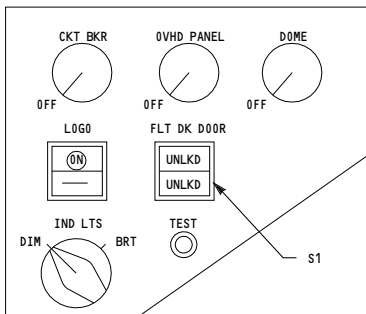
M10057 RIGHT LIGHTING CONTROL MODULE ASSY (P5)
