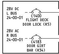
P11 OVERHEAD CIRCUIT BREAKER PANEL
