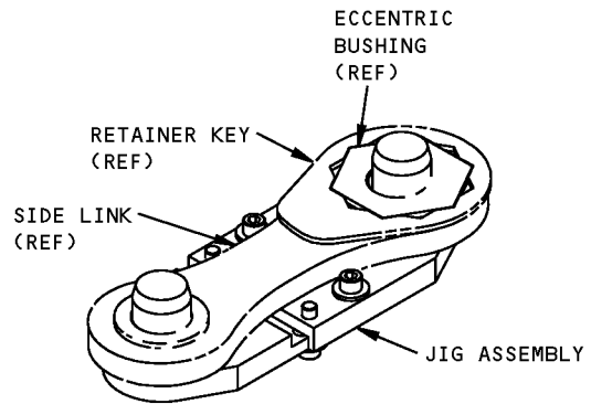
HOLDING JIG FOR DRILLING STEP II
