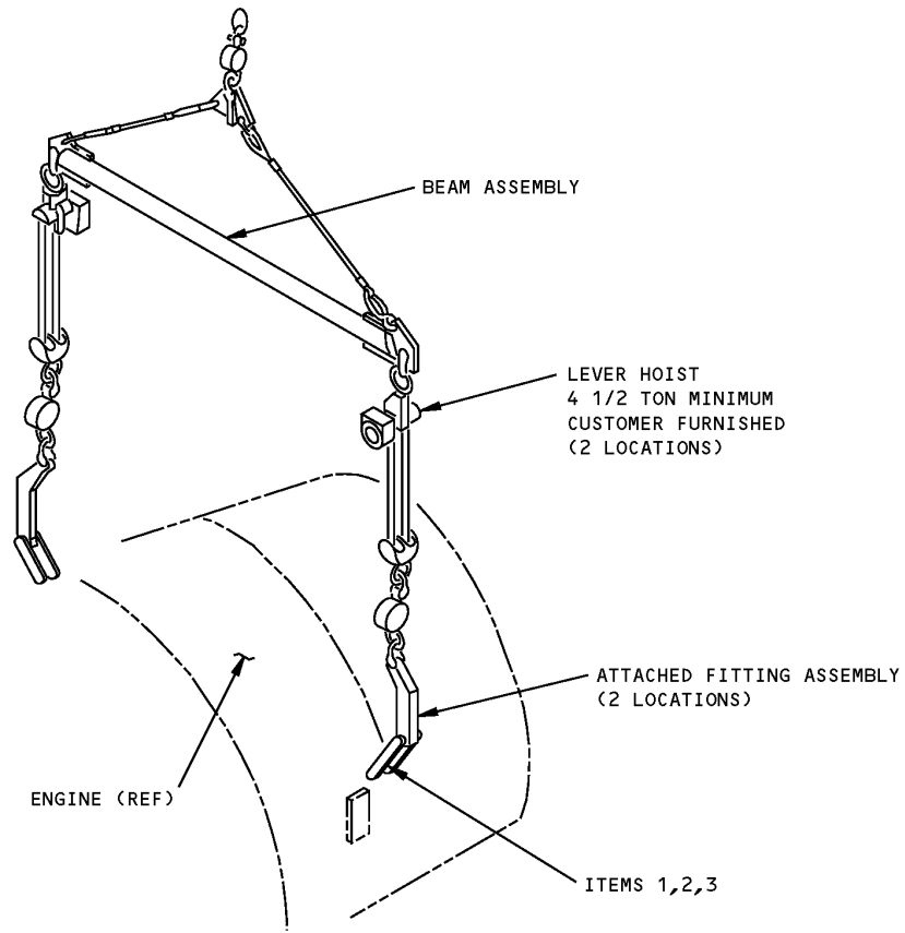
A54001-165 AND -168 SLING EQUIPMENT
