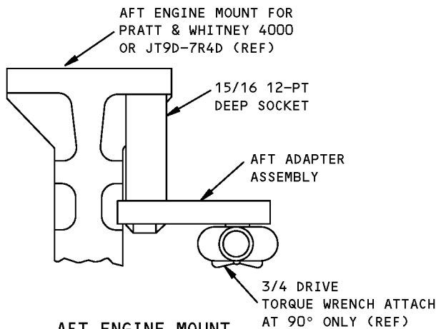
AFT ENGINE MOUNT A71003-25,-53 (767 ONLY)
