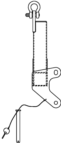
A71047-13 RIGHT HAND FORWARD HOIST ASSEMBLY SHOWN A71047-14 LEFT HAND FORWARD HOIST ASSEMBLY SIMILAR
