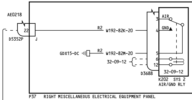
P37 RIGHT MISCELLANEOUS ELECTRICAL EQUIPMENT PANEL
