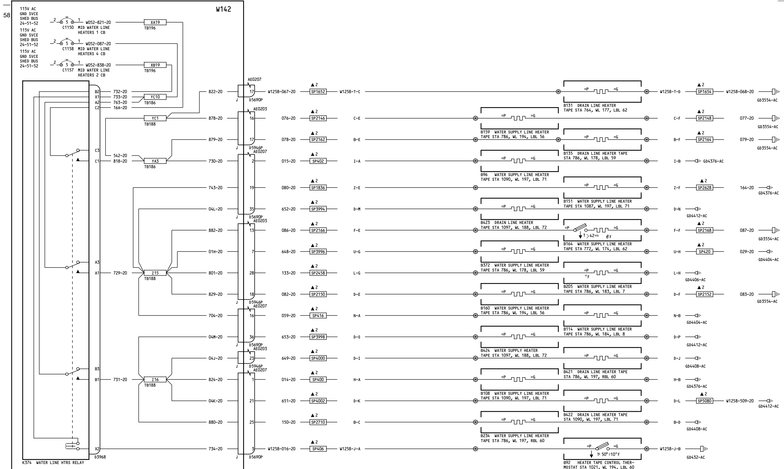
P33 FORWARD MISCELLANEOUS ELECTRICAL EQUIPMENT PANEL
