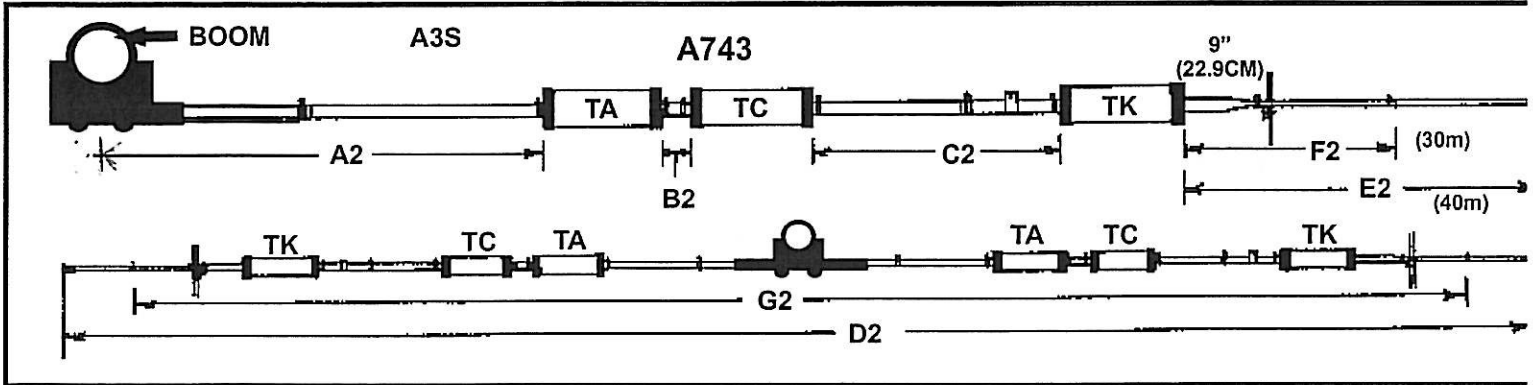
A743 DRIVEN ELEMENT LENGTH ADJUSTMENT
