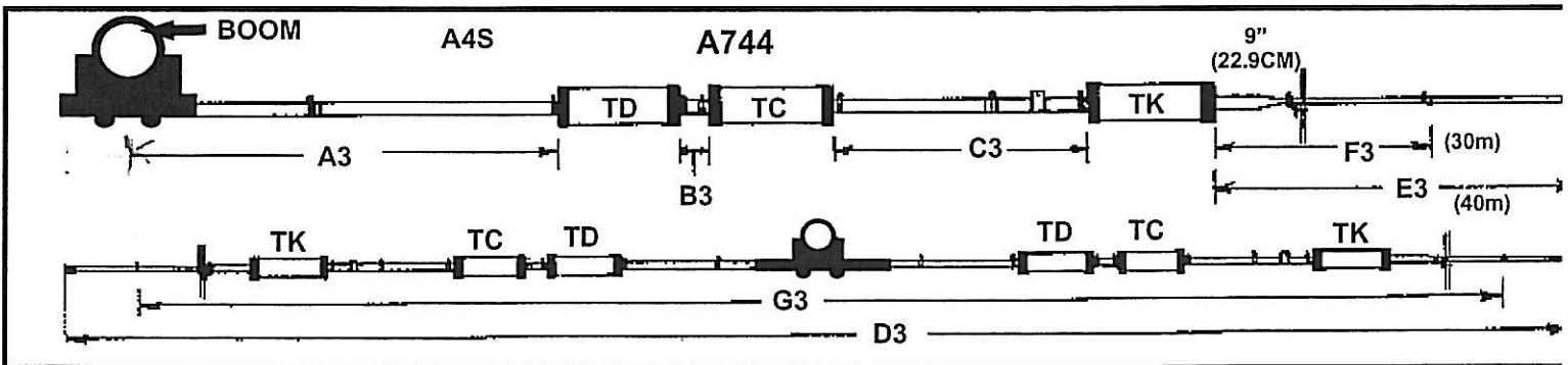
A744 DRIVEN ELEMENT LENGTH ADJUSTMENT
