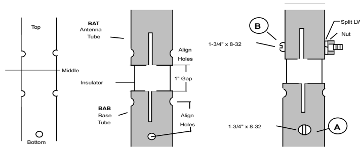
Figure-1: Base Insulator Assembly
