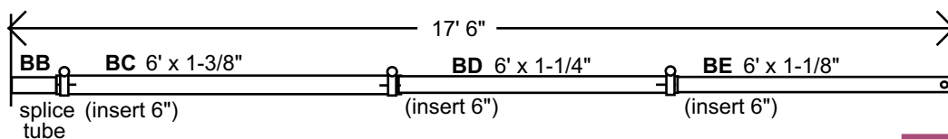
Figure-8: Vertical Radiator Assembly
