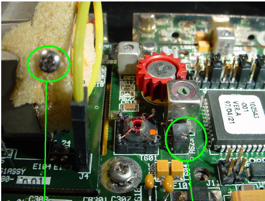
Fig 12, Cavity tuning 6.8 GHz
