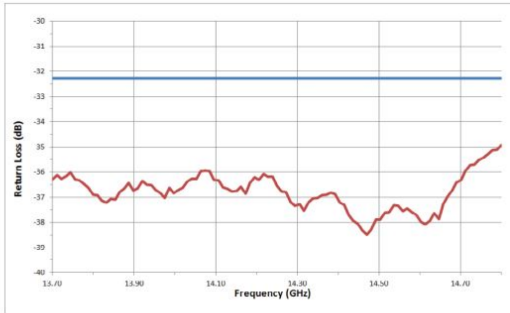
Typical Return Loss for Model 17094-SF48
