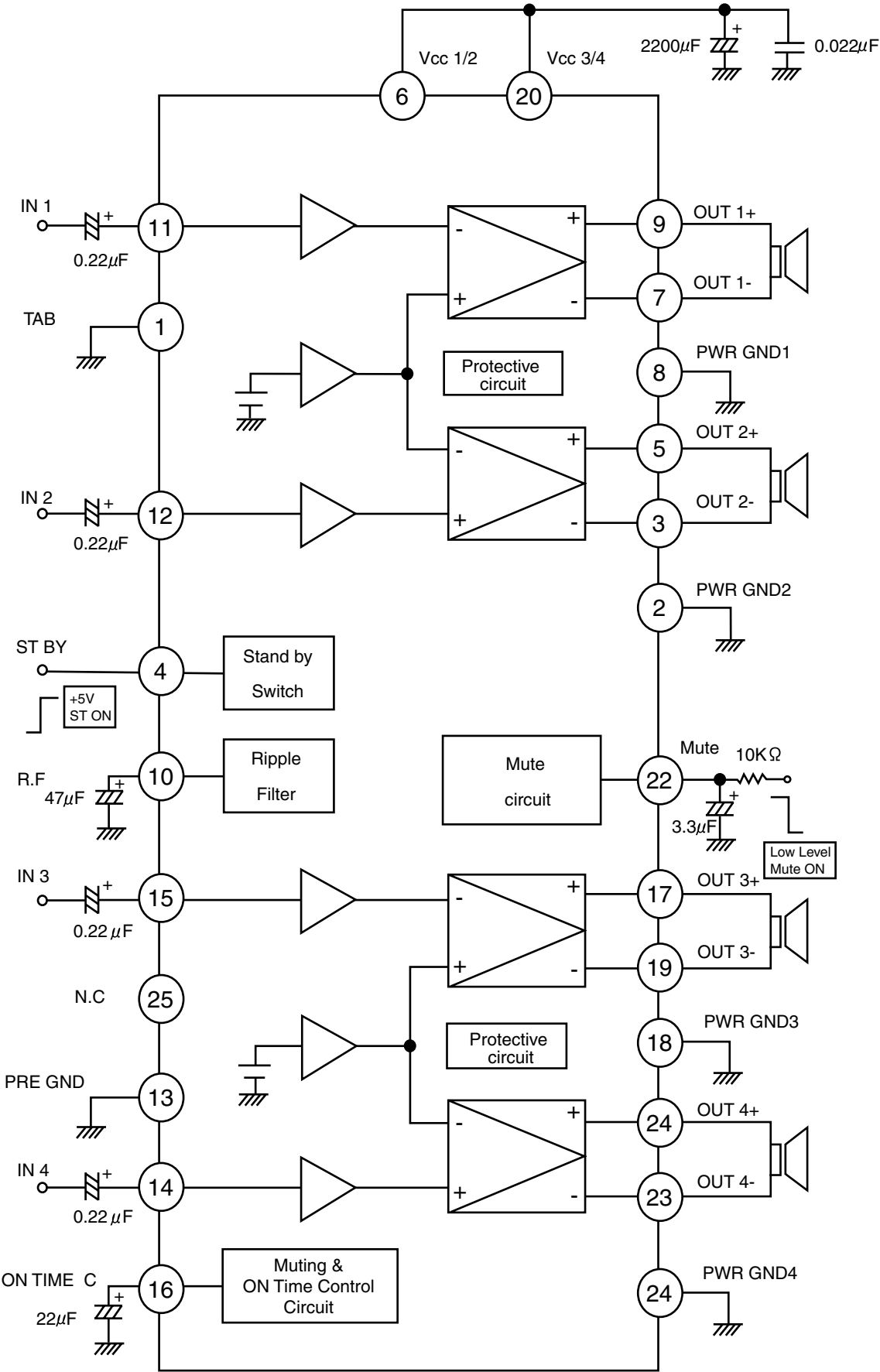
1.Block diagram
