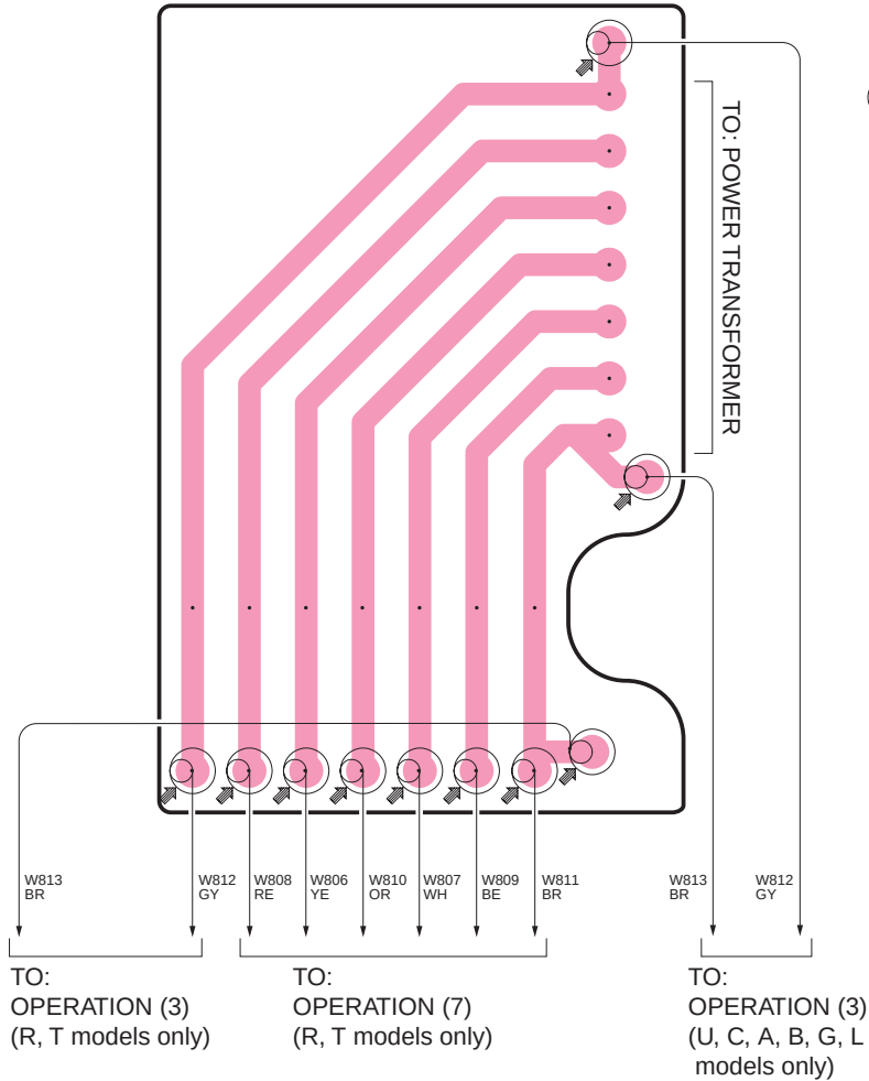
● U, C, R and T models P. C. B. OPERATION (3)
