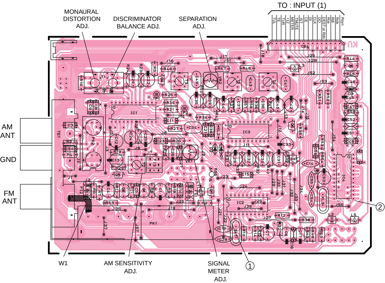
B and G models P. C. B. TUNER (Lead Type)
