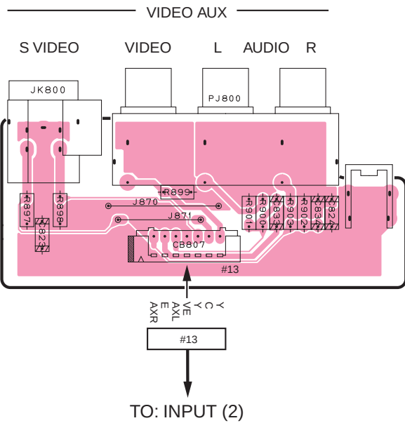
P. C. B. OPERATION (2)
