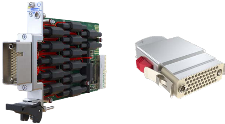
Figure 3 – PXI switching module from Pickering with 9 kV capability (left) and associated Redel high-voltage connector (right).
