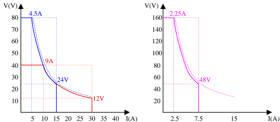
80V 15A/ 40V 30A Output Operating Area
