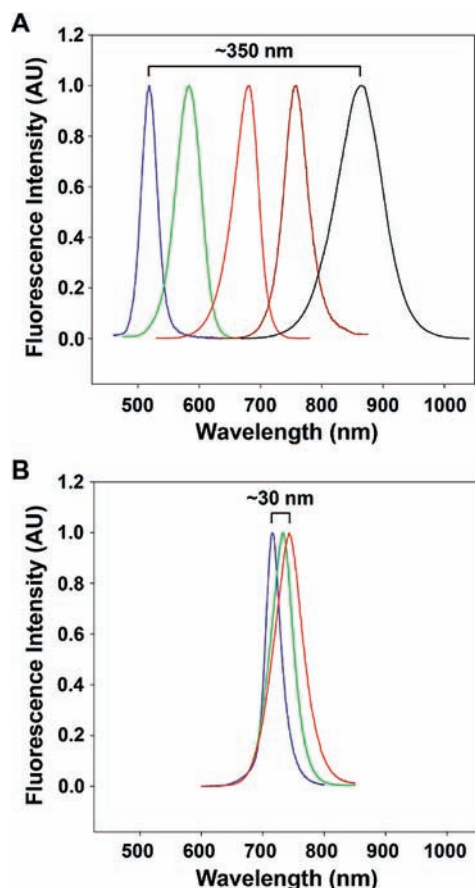
FIGURE 8. Fluorescence spectra of strain-tunable (CdTe)ZnSe quantum dots. (A) Fluorescence from 1.8 nm CdTe cores strongly red-shifts when capped with 0–6 monolayers of ZnSe shell (from blue to black) due to strain-induced changes in the core and shell lattices. (B) Fluorescence from 6.2 nm CdTe cores only exhibits a small red-shift when capped with 0–5 monolayers of ZnSe shell (from blue to red) due to strain relaxation through lattice defect formation. See ref 41.
