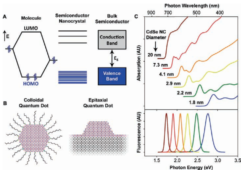
FIGURE 1. (A) Electronic energy states of a semiconductor in the transition from discrete molecules to nanosized crystals and bulk crystals. Blue shading denotes ground state electron occupation. (B) Comparison of a colloidal quantum dot and an islandlike, self-assembled quantum dot epitaxially deposited on a crystalline substrate. (C) Absorption (upper) and fluorescence (lower) spectra of CdSe semiconductor nanocrystals showing quantum confinement and size tunability. AU = arbitrary units.
