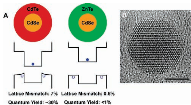
FIGURE 9. Band-edge warping induced by lattice strain. (A) Energy band levels of quantum confined, strained (core)shell (CdSe)CdTe and (CdSe)ZnTe nanocrystals show that band warping is only significant in the highly strained structure (CdSe)CdTe, resulting in efficient recombination efficiency. (B) Representative transmission electron micrograph of a highly strained (CdSe)ZnS shows direct evidence of lattice warping at core–shell interfaces. Scale bar is 5 nm.
