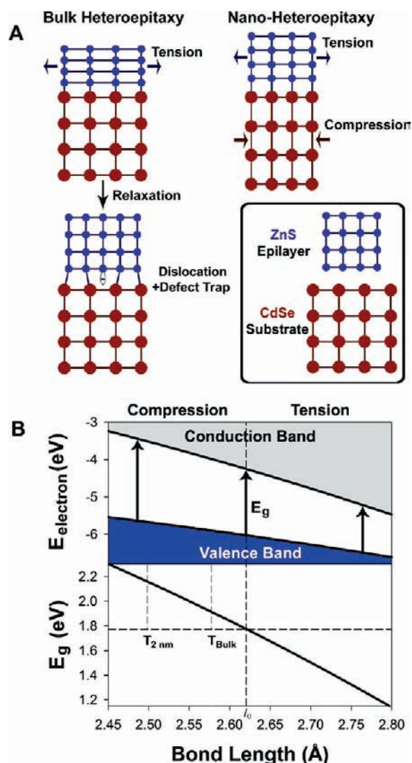
FIGURE 7. Epitaxial semiconductor heterostructures and impact of strain on band gap energy. Panel (A) shows exaggerated crystal domains of CdSe and ZnS with a large mismatch in lattice constant. Epitaxial growth of ZnS on a bulk CdSe substrate results in tensile strain in ZnS that cannot be tolerated, resulting in relaxation of the tension through a misfit dislocation. However, a nanometer-sized CdSe substrate can deform with growth of a ZnS shell, resulting in a sharing of the strain through compression of the CdSe domain, preventing defect formation. Panel (B) depicts how the energy of the valence band edge, conduction band edge, and band gap change with CdSe bond length. The equilibrium bond length is noted on the x-axis ( l_0 = 2.62 \text{ \AA} ) in addition to the bond length that results in a phase transition in bulk ( T_{\text{Bulk}} ) and for small 2 nm nanocrystals ( T_{2\text{nm}} ).
