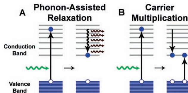
FIGURE 5. Schematic illustration of electronic energy relaxation and carrier multiplication in quantum dots. (A) Electrons excited to energies greater than the band edge efficiently relax to the band edge through the release of phonons, or quanta of lattice vibration. (B) Alternatively, excited state electrons with kinetic energy greater than the band gap can transfer their energy to a second electron via impact ionization, yielding two excitons.
