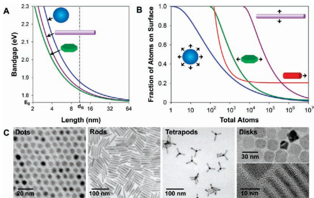
FIGURE 2. Impact of shape on the electronic and surface properties of semiconductor nanocrystals. (A) Band gaps of CdSe quantum wells, wires, and dots are plotted against the length of the confined dimension. The bulk band gap and exciton diameter are noted on the axes. (B) Fractions of atoms on the nanocrystal surface are plotted against the total number of atoms. The wires (purple) are 1 \mu\text{m} in length, the rods (green) are 20 nm in length, and the rods (red) are 4 nm in diameter. (C) Transmission electron micrographs depicting CdSe dots, rods, 13 tetrapods, 14 and disks. 12
