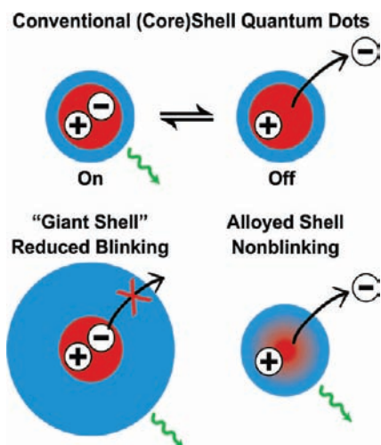
FIGURE 4. Schematic diagrams showing on/off light emission (blinking) in conventional (core)shell nanocrystals (upper), and suppression of blinking in giant-shell and gradient alloy nanocrystals (lower). See text for discussion.
