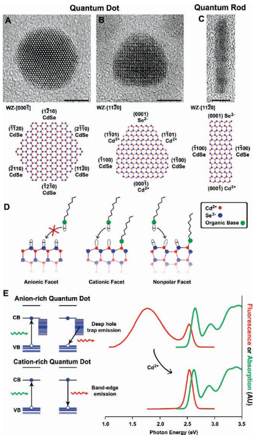
FIGURE 3. Surface properties of CdSe nanocrystals. Panels (A) and (B) depict transmission electron micrographs of quasi-spherical quantum dots with two orientations on the substrate, and panel (C) depicts a quantum rod. 11 All scale bars are 5 nm. In the atomic models, the crystalline orientations and lattice facets are identified by their Wurtzite (WZ) Miller indices, and the polarity of each facet is noted as Cd ^{2+} for cationic, Se ^{2-} for anionic, and CdSe for nonpolar. Panel (D) illustrates the terminal dangling orbitals on each type of facet, and panel (E) shows the effects of surface hole traps on the fluorescence of small 2.1 nm nanocrystals.
