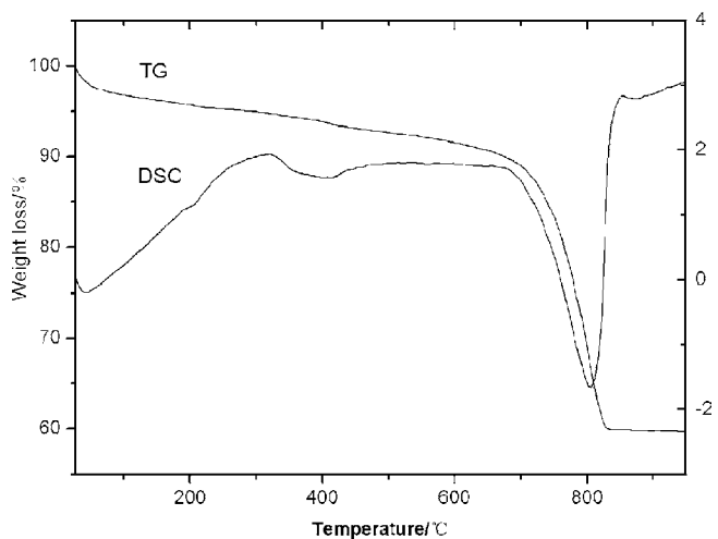
FIGURE 3. TG-DSC curves of mortar samples obtained from the Nanjing city wall.
