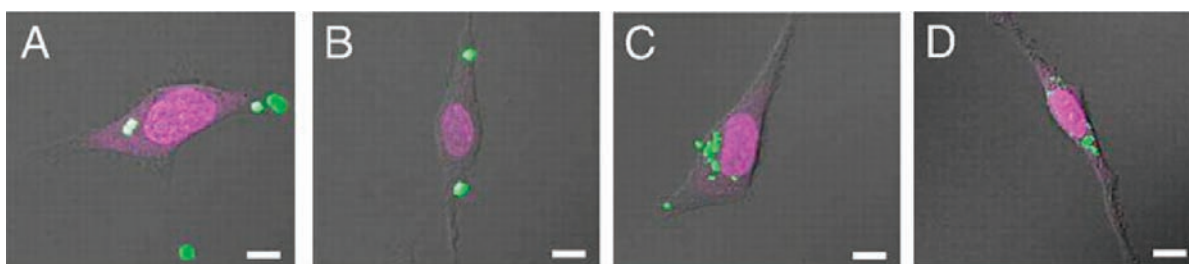
FIGURE 5. Confocal laser scanning microscopy micrographs of HeLa cells after a 1 h incubation period at 37 ^{\circ}\text{C} with (A) 3 \mu\text{m} cubic, (B) 2 \mu\text{m} cubic, (C) 1 \times 1 \mu\text{m} cylindrical, and (D) 200 \times 200 nm cylindrical particles. Scale bar represents 10 \mu\text{m} in all images. Reprinted with permission from ref 28. Copyright 2008 National Academy of Science.
