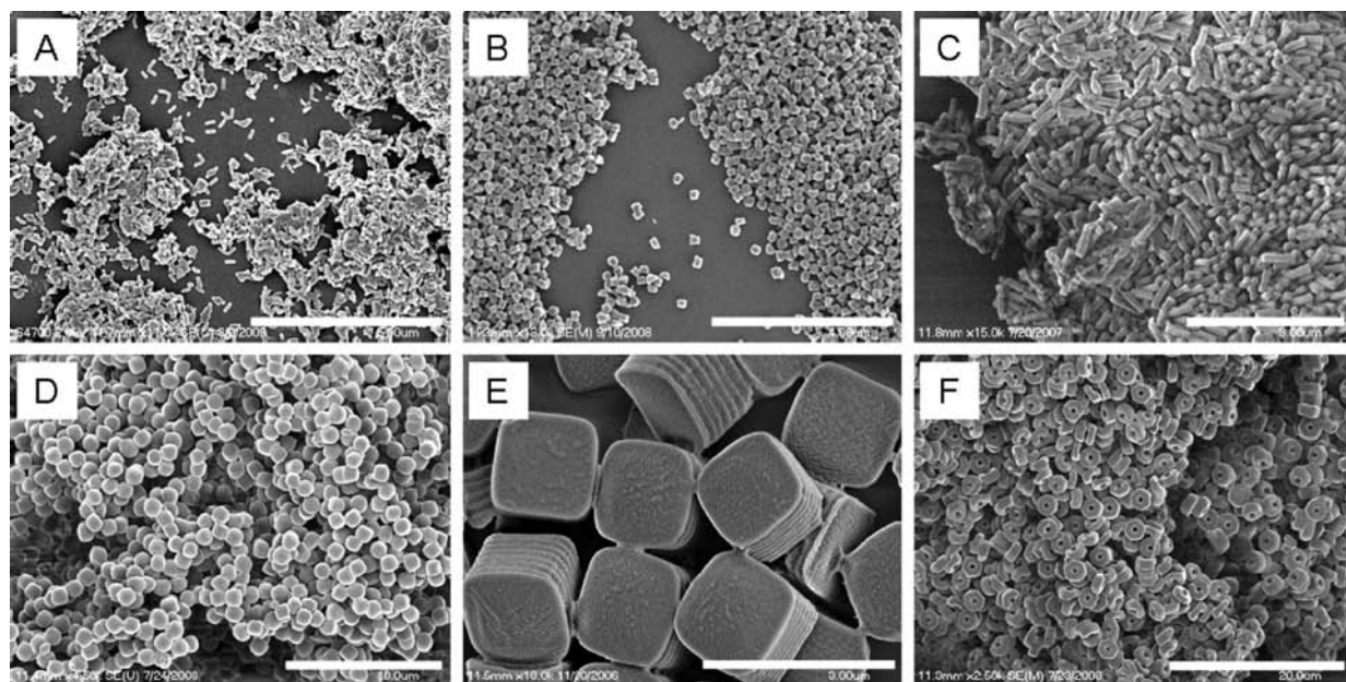
FIGURE 3. Scanning electron micrographs of PLGA PRINT particles: (A) 80 \times 320 nm cylinders, (B) 200 \times 200 nm cylinders, (C) 200 \times 600 nm cylinders, (D) 1 \mu\text{m} sphere approximates, (E) 2 \mu\text{m} cubes with ridges, and (F) 3 \mu\text{m} particles with center fenestrations. Scale bars: (A) 5 \mu\text{m} , (B) 4 \mu\text{m} , (C) 3 \mu\text{m} , (D) 10 \mu\text{m} , (E) 3 \mu\text{m} , and (F) 20 \mu\text{m} . Reprinted with permission from ref 43. Copyright 2011 American Chemical Society.
