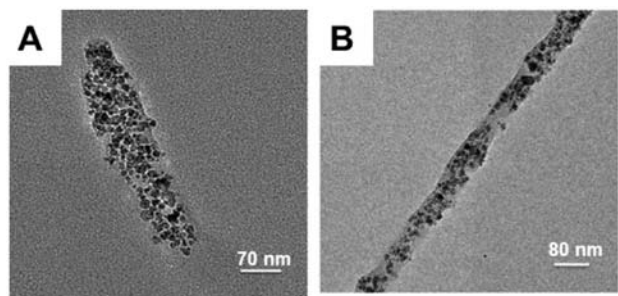
FIGURE 9. Transmission electron microscopy images of PRINT particles (A) 80 \times 320 nm and (B) 80 \times 2000 nm containing iron oxide nanoparticles. Reprinted with permission from ref 39. Copyright 2010 American Chemical Society.
