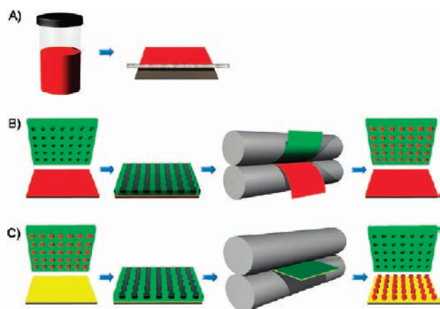
FIGURE 1. Schematic illustration of the PRINT process. (A) Delivery sheet casting: A true solution (red) is made and then cast on a PET substrate using a mayer rod. Solvent is removed under heat, generating a solid state solution film referred to as the delivery sheet, as it will deliver the composition to the mold. (B) Particle fabrication: a perfluoropolyether elastomeric mold (green) is brought into contact with a delivery sheet (red), passed through a heated nip (gray), and split. The cavities of the mold are filled. (C) Particle harvesting: a filled mold is brought into contact with a high energy film or excipient layer (yellow) and passed through the heated nip without splitting. After cooling, the mold is removed to reveal an array of particles on the high-energy film or excipient layer. Reprinted with permission from ref 43. Copyright 2011 American Chemical Society.
