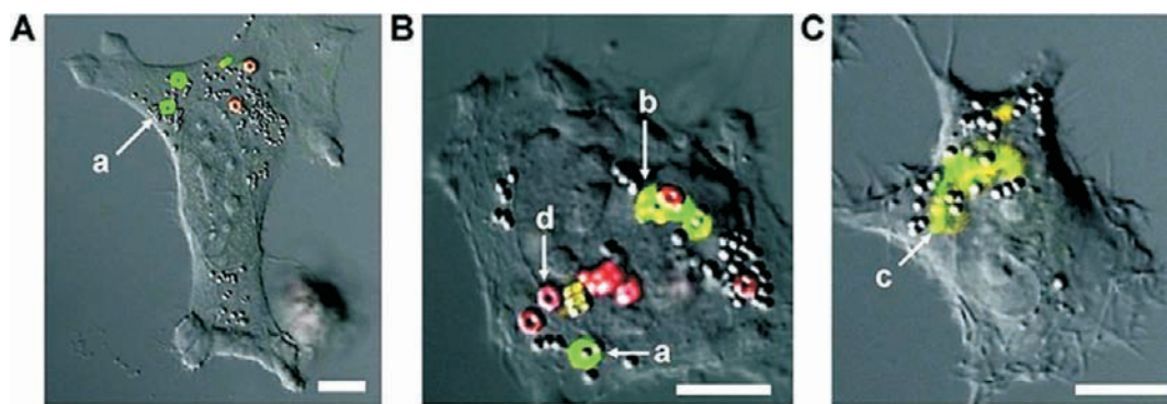
FIGURE 4. Confocal laser scanning micrographs of HeLa cells incubated with rapidly degrading hexnut particles (green) and nondegrading hexnut particles (red). Micrographs (A–C) highlight the phases of particle degradation: swelling (a), fragmentation (b), and complete degradation (c). The nondegradable particles showed no change when exposed to intracellular conditions (d). Scale bar represents 10 \mu\text{m} for all images. Reprinted with permission from ref 38. Copyright 2010 American Chemical Society.
