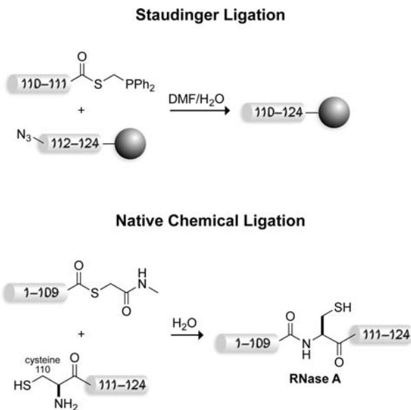
FIGURE 10. Semisynthesis of RNase A by integrating the traceless Staudinger ligation (here, on a resin) and NCL. 87
