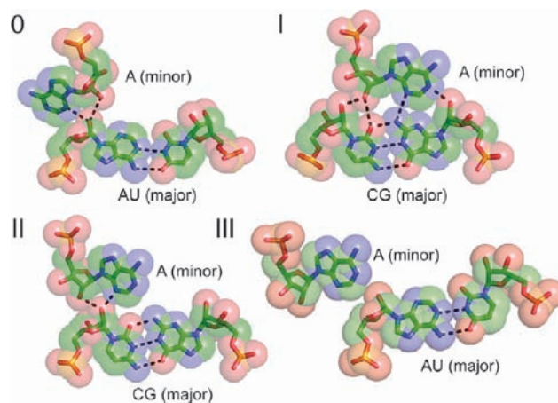
FIGURE 4. Examples of four A-minor interaction subtypes from the large ribosomal subunit, PDB ID 1FFK. Major and minor groove edges are indicated.
