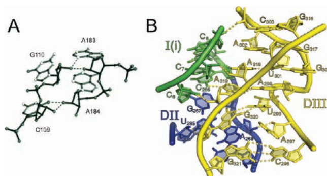
FIGURE 10. Ribose zippers in RNA structure: (A) a ribose zipper from P456; 25 (B) a network of ribose zippers joining domains 1, 2, and 3 in group II intron, PDB ID 3IG1. 46
