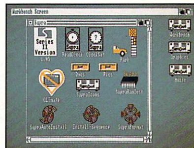
Included Software
