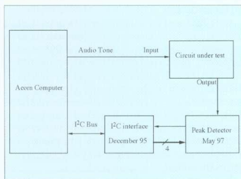
Figure I: The Frequency Response plotter set up
