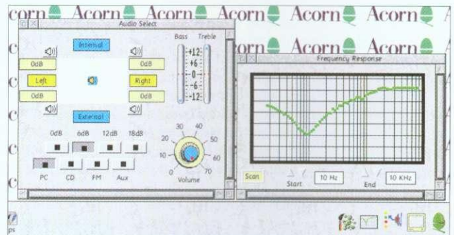
Figure IV: With a bass cut and a treble boost there's a dip in the response at 100 Hz before it climbs
