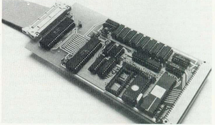
6809 second processor from CMS uses Tube interface
