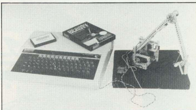
Beasty links Beeb to servo devices on crane
