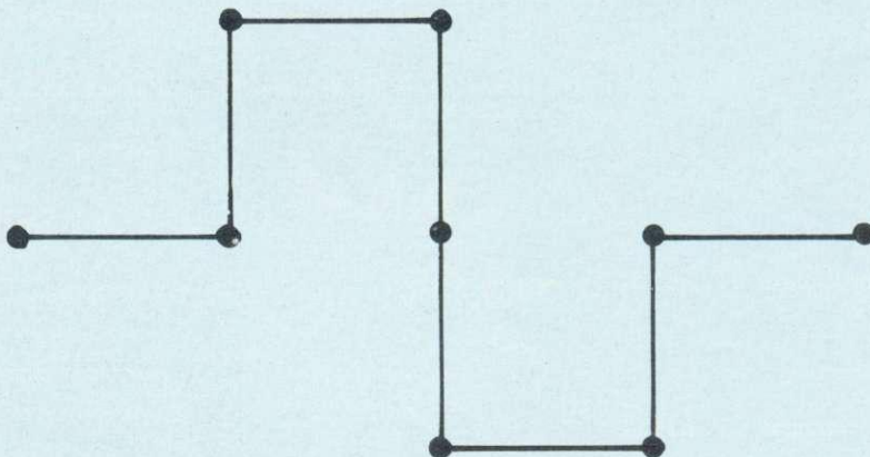
Figure 2b. The seven-point von Koch generator. Co-ordinates (1/4, 0), (1/4, 1/4), (1/2, 1/4), (1/2, 0), (1/2, -1/4), (3/4, -1/4), (3/4, 0). (Try also the six-point generator, with (3/4, 0) missing)
