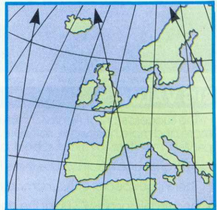
Figure 1. Consecutive orbits
