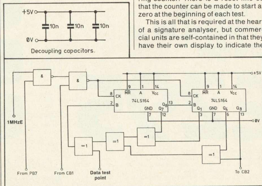
Figure 1. Hardware of the self-test signature analysis system
