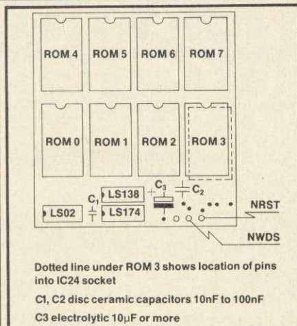
Figure 3. PCB layout
