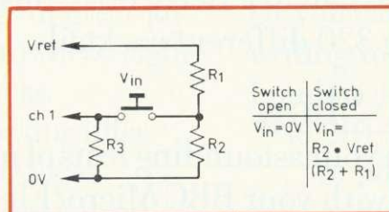
Figure 2. Switched divider
