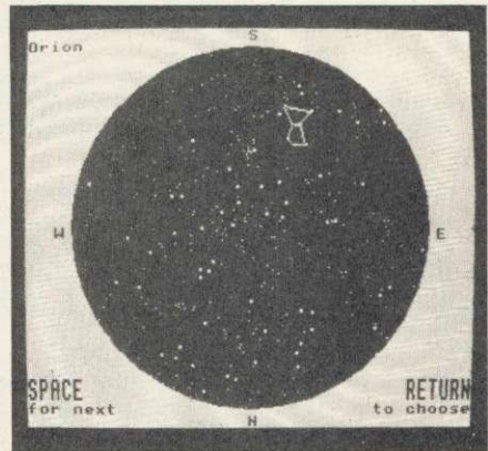
Star map showing the position of the constellation of Orion from the 'Star Gazer' program.
