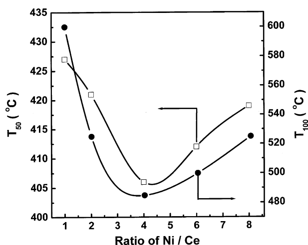
Figure 2. Temperature dependence for 50% and 100% conversion of CH 4 as a function of various Ni/Ce molar ratios.
