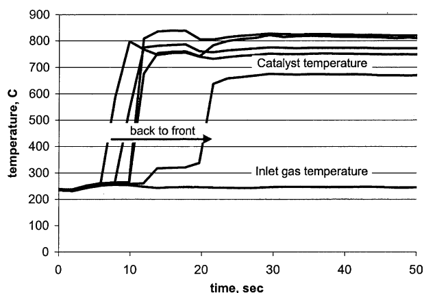
Figure 2. Light off of the Microlith based CPOX of methane reactor. P = 0.6 Mpa.
