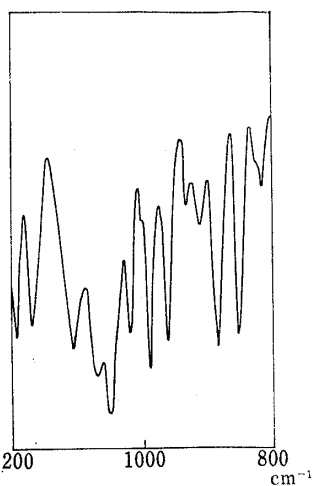
Fig. 2. Infrared Absorption Spectrum of 3- \beta -Methylphenethyltetrahydro-1,3-oxazine (XX) (Liquid)
