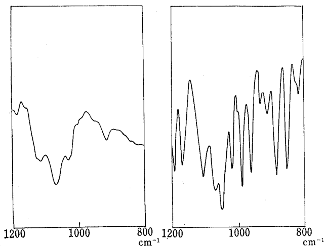
Fig. 1. Infrared Absorption Spectrum of N- \beta -Methylphenethyl-3-amino-1-propanol (X) (Liquid)
