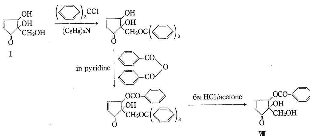
Chart 1. Synthesis of 4-O-Monobenzoyl Pentenomycin I (VIII)
