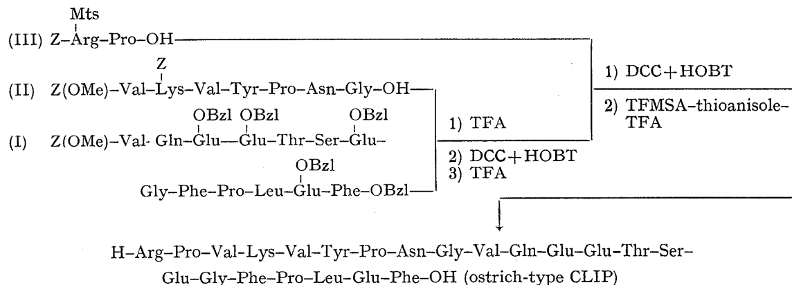
Fig. 1. Synthetic Route to Ostrich-type CLIP
