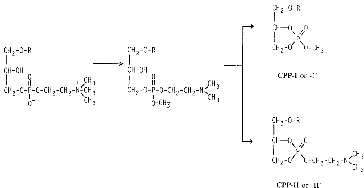
Chart 1. Major Pyrolysis Pathways for 16:0-Lyso-PC and 16:0-Lyso-PAF
