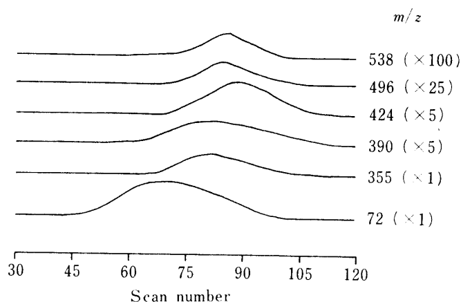
Fig. 5. Ion-Current Profiles of Extracted Ions in the Ammonia CI-MS of 16:0—2:0-PC
