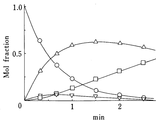
Fig. 3. Time Courses of CQ (○), 3 (▽), 7 (△) and 8 (□) During the Degradation of CQ in Proton-Rich Methanol at 60°C
