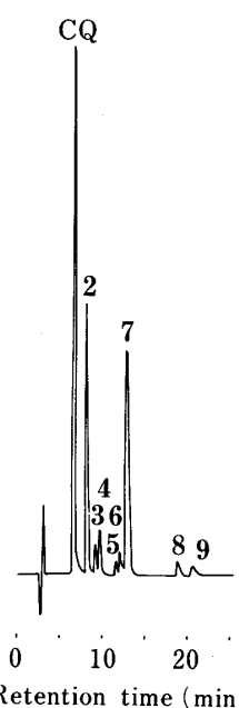
Fig. 2. Chromatogram Obtained by HPLC of CQ Stored in Methanol at 60 °C for 6 d
