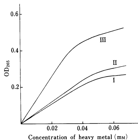
Fig. 8. Binding Study of Peptide with Cu
