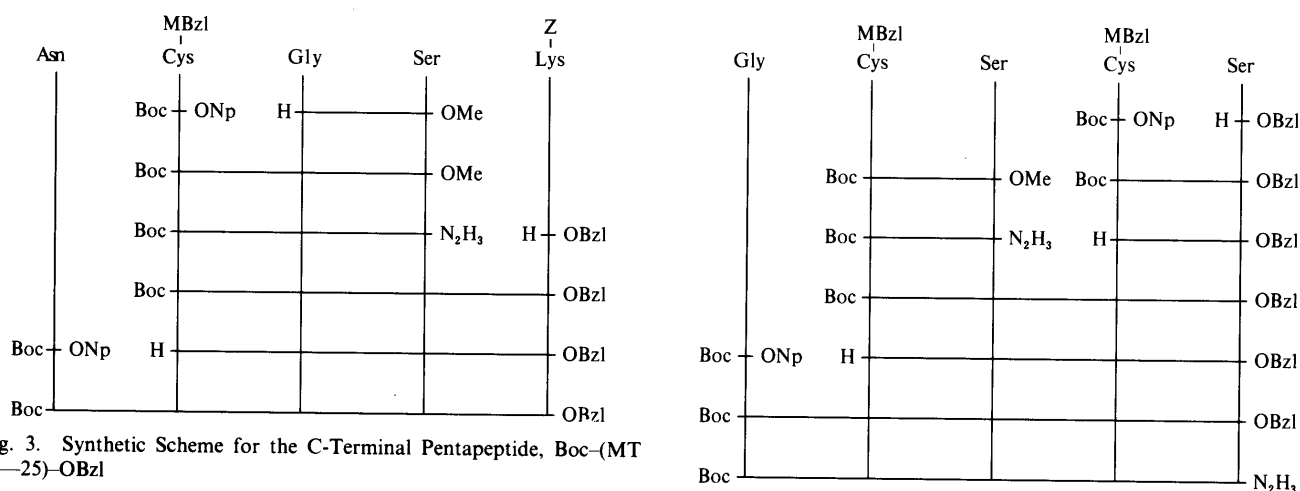
Fig. 4. Synthetic Scheme for the Protected Pentapeptide Hydrazide, Boc-(MT 16-20)-N 2 H 3
