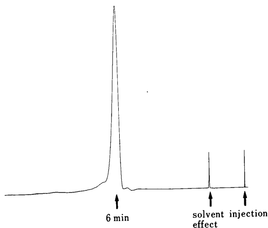
Fig. 6. HPLC Profile of the Synthetic Pentacosapeptide
