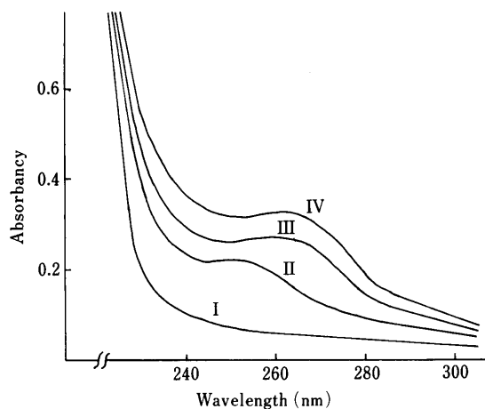
Fig. 7. Binding Study of Peptide with Heavy Metals
