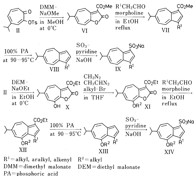
Chart 2. Synthetic Route to Azulene Derivatives
