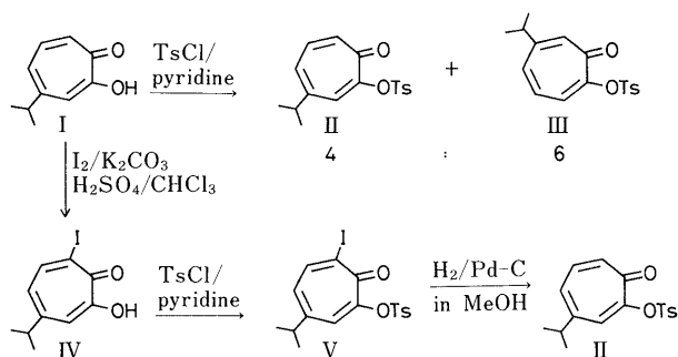
Chart 1. Synthetic Route to 4-Isopropyl-2-tosyloxypone
